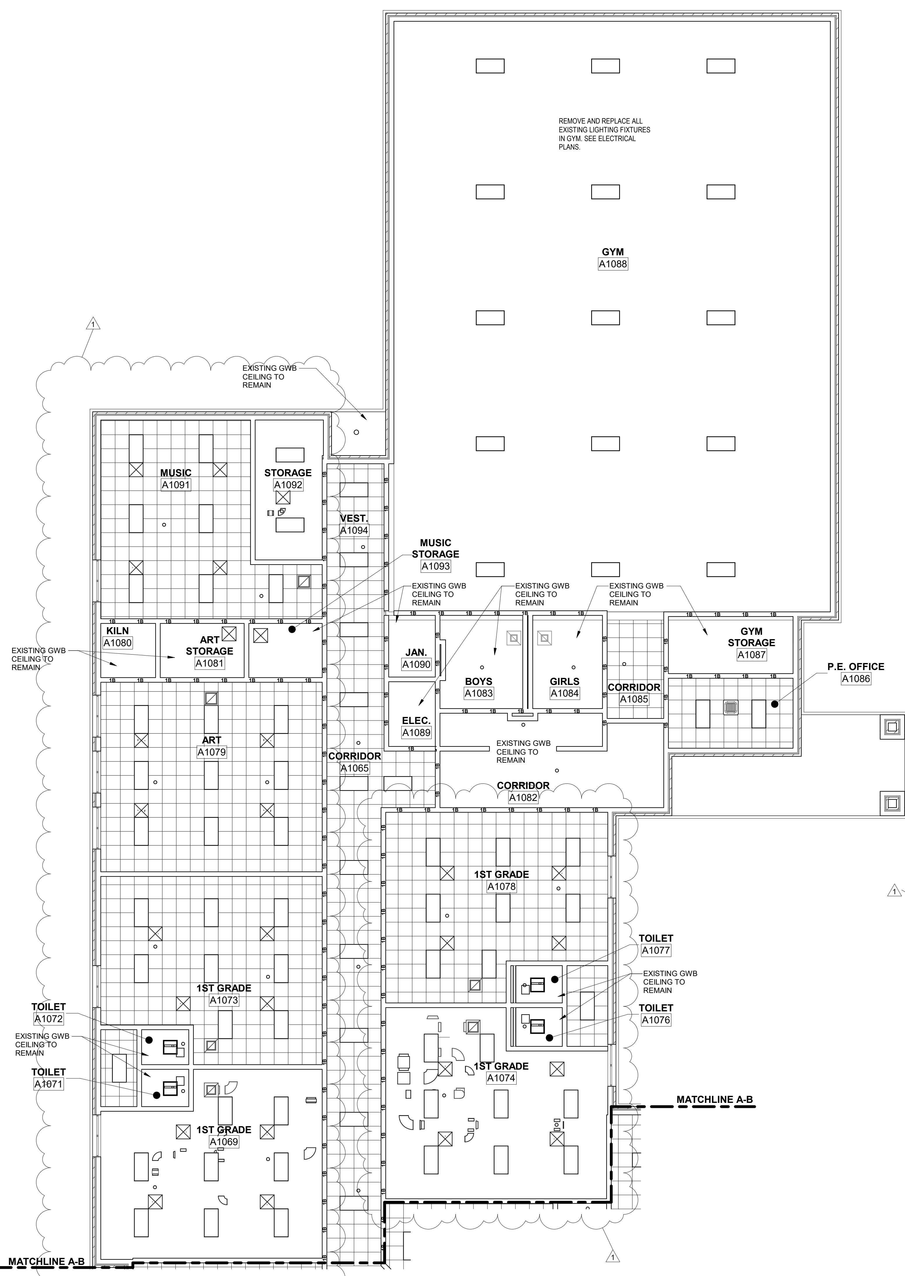
1 REFLECTED CEILING PLAN - WING A 1/8" = 1'-0"
