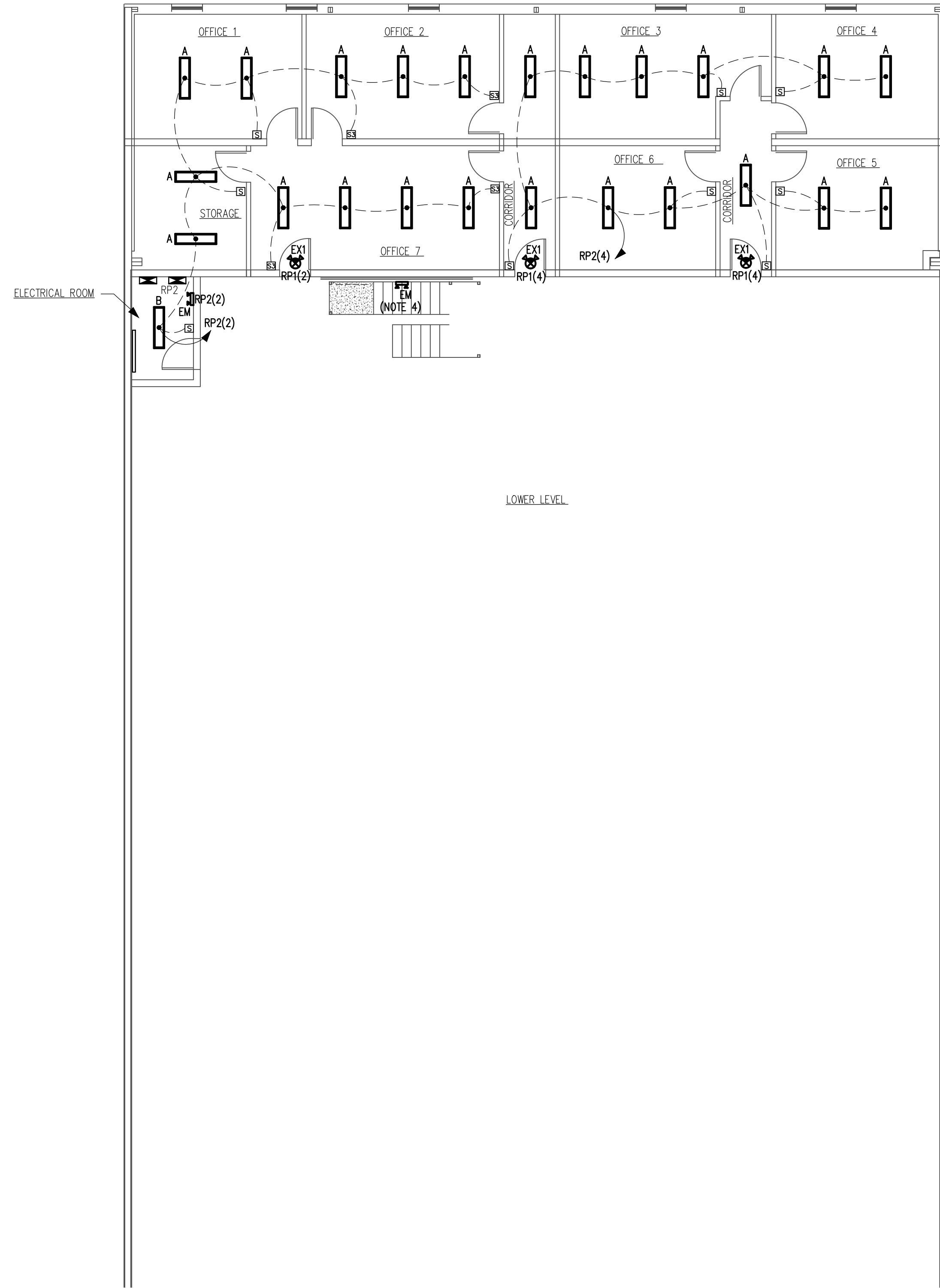
LOWER LEVEL LIGHTING PLAN SCALE: 1/8" = 1'-0"
