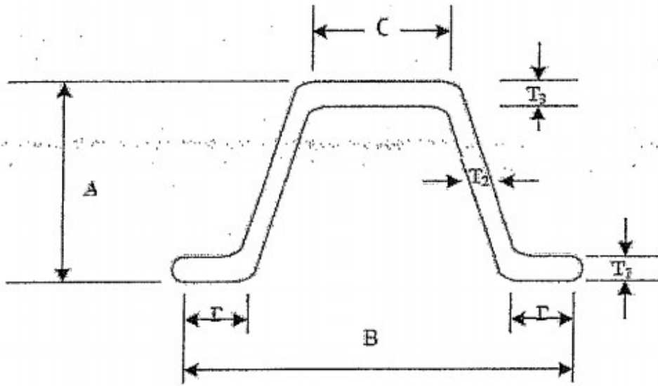
DRAWING 'A'
