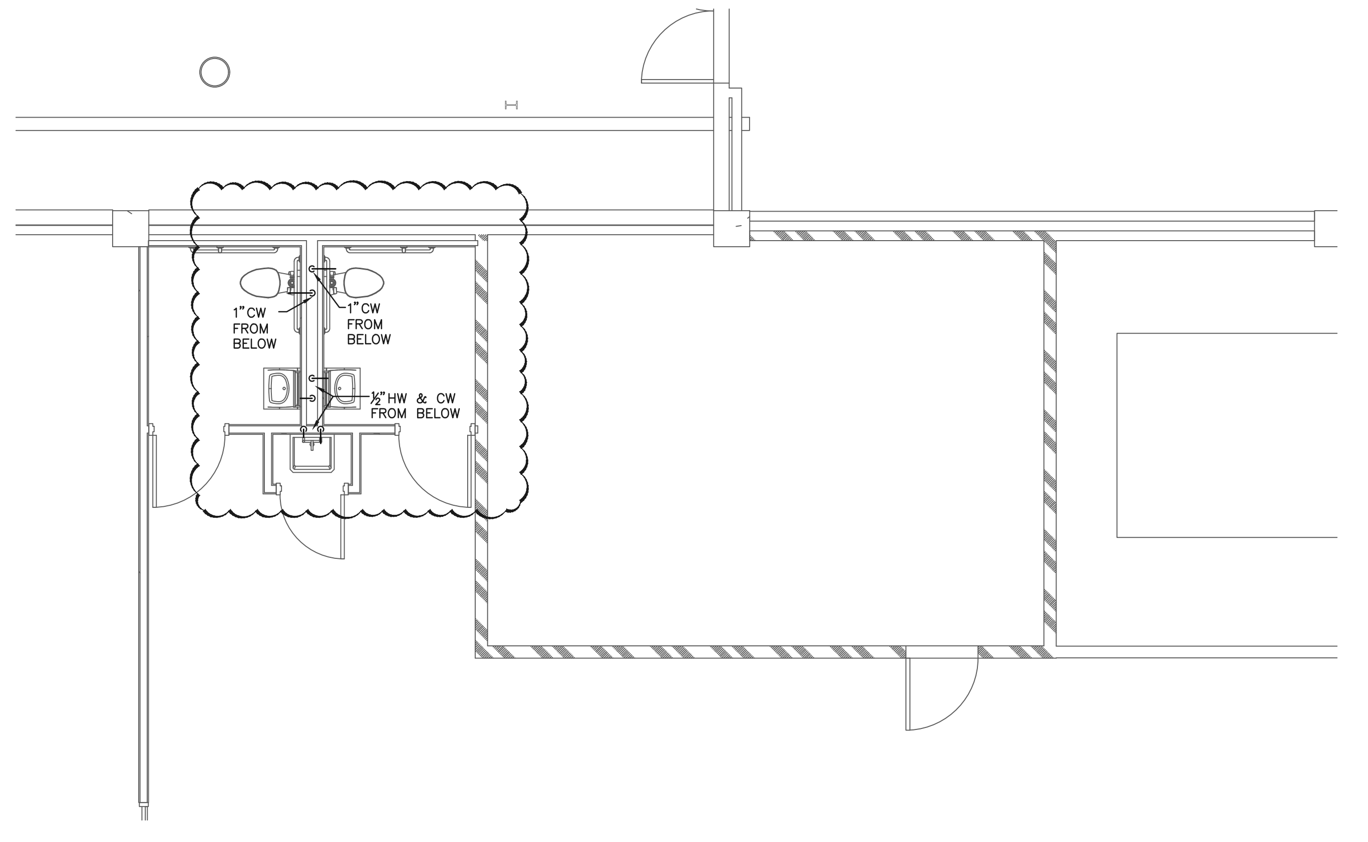
5 FOURTH LEVEL - WATER PIPING SCALE: 1/4" = 1'-0"
