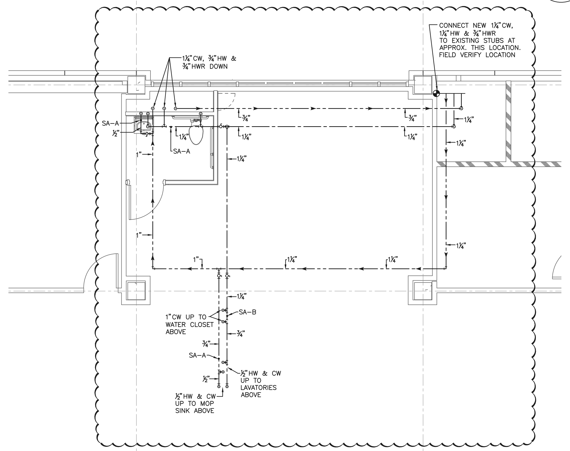
4 THIRD LEVEL - WATER PIPING SCALE: 1/4" = 1'-0"
