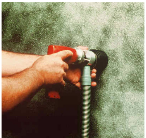
FIGURE 12.19 Needle Gun with HEPA Exhaust Ventilation.
