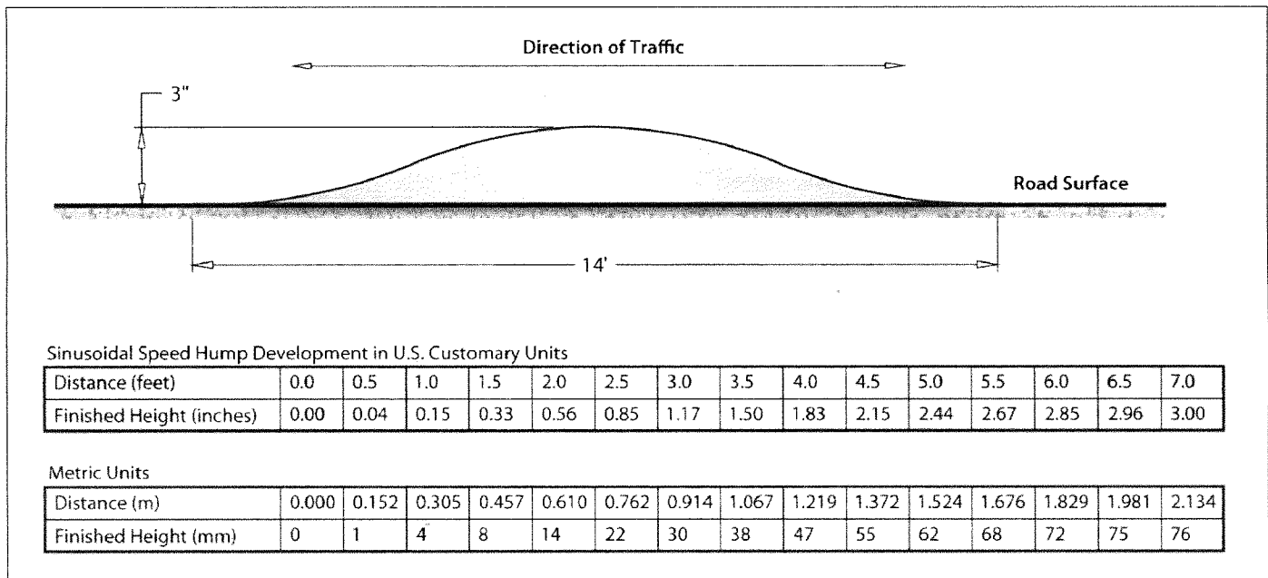
Figure 4.2. Typical sinusoidal speed hump. Note: Not to scale.
