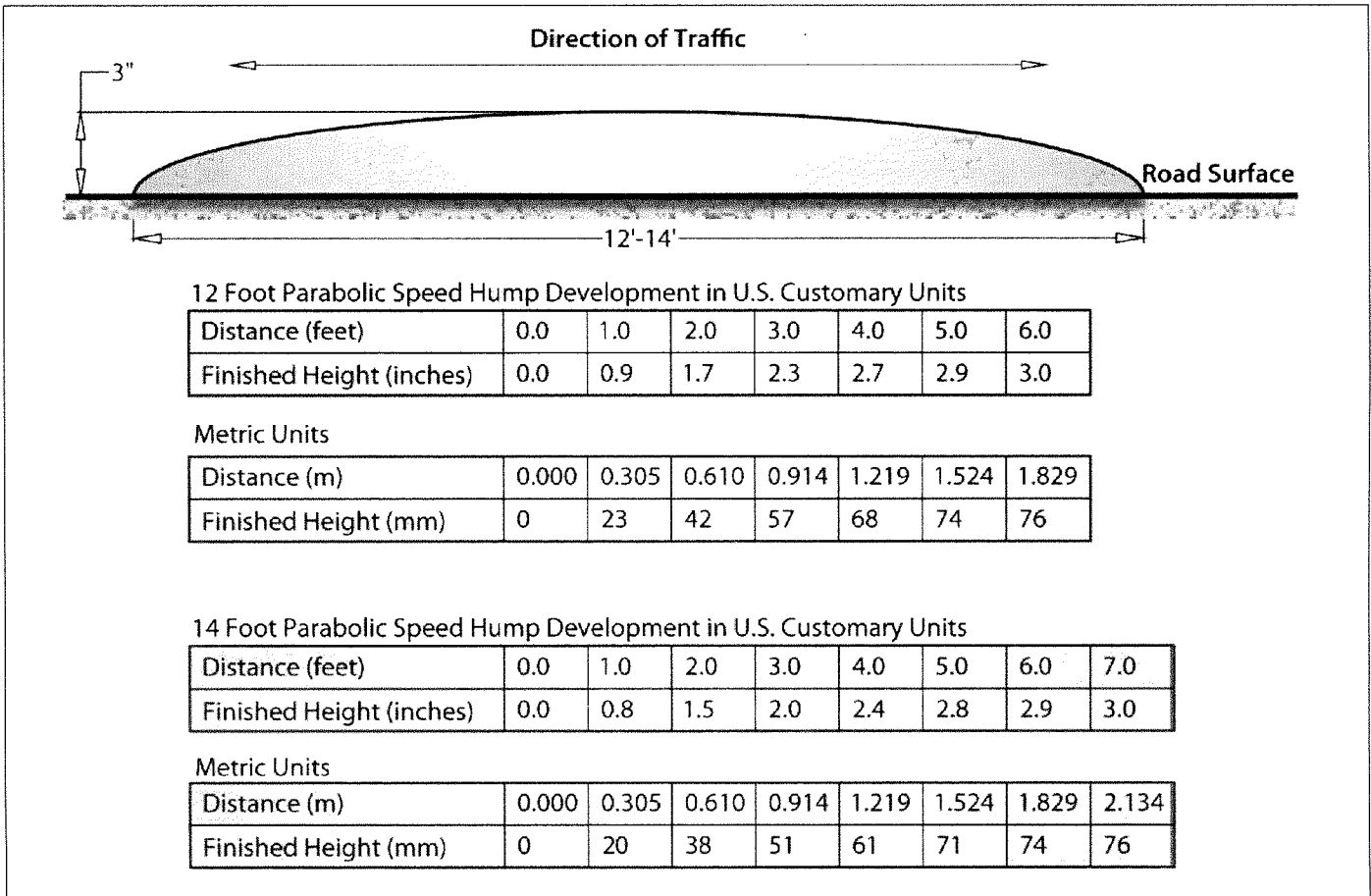
Figure 4.1. Typical parabolic speed hump. Note: Not to scale.
