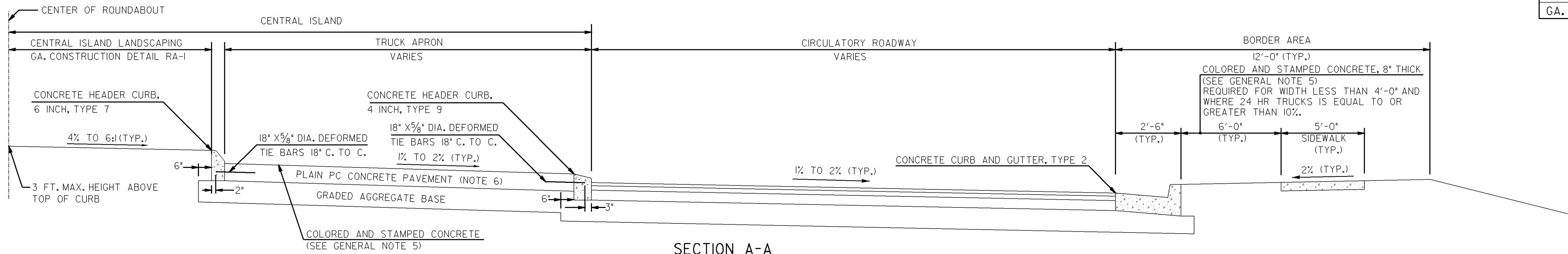
SECTION A-A NOT TO SCALE (NOTE 3)
