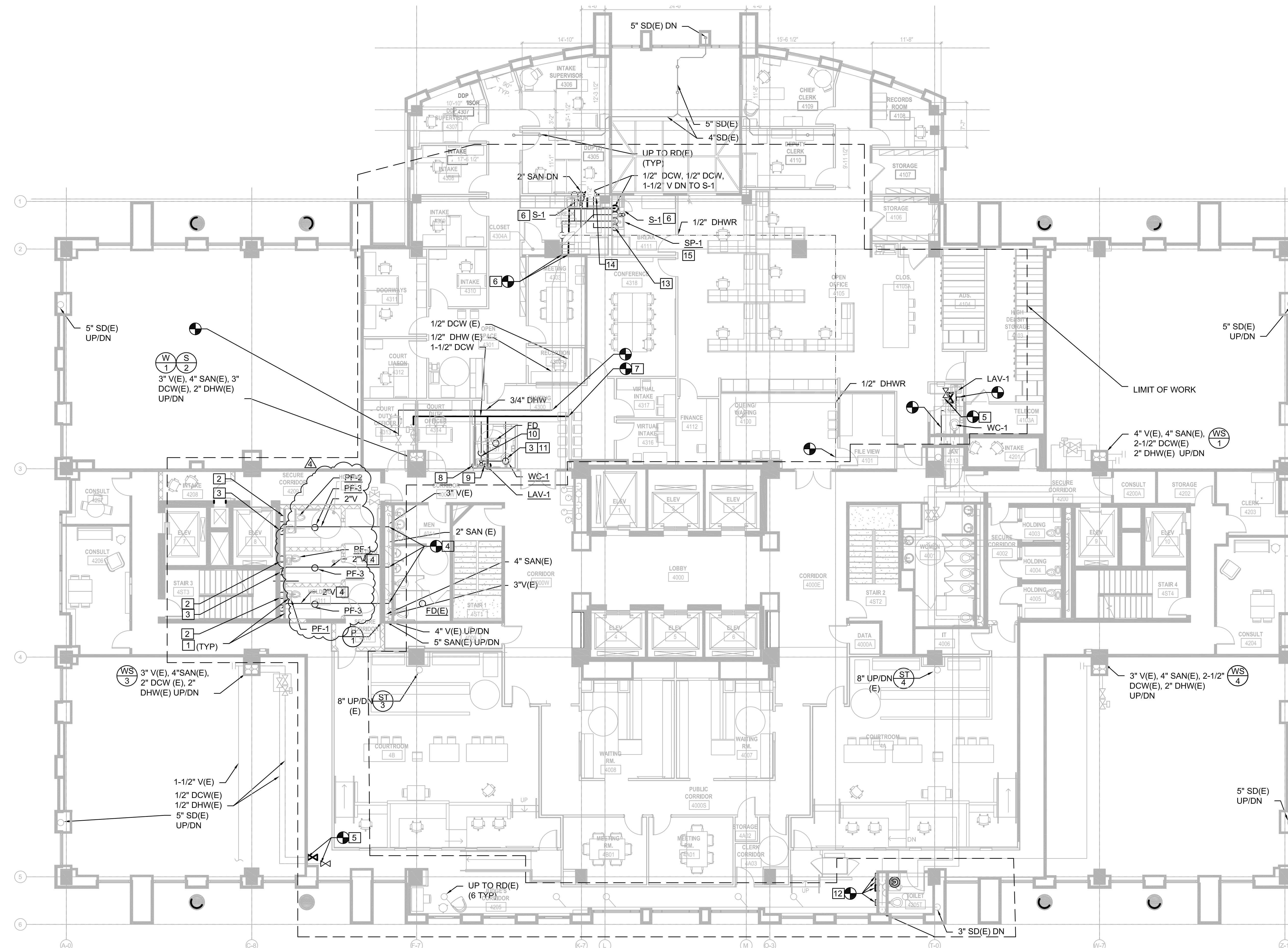
1 4TH FLOOR PLAN PLUMBING - NEW WORK Scale: 1/8"=1'-0"
