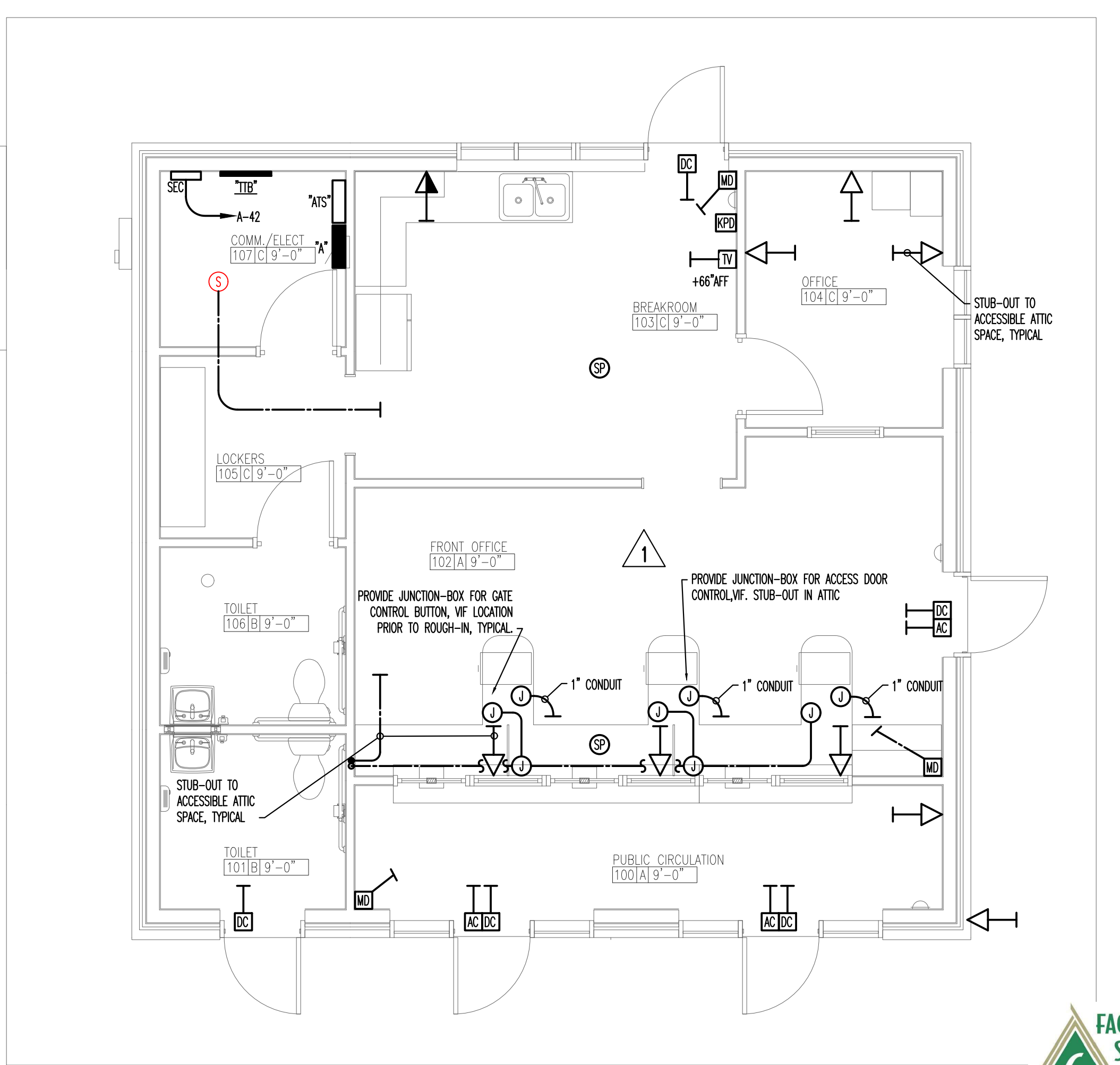
COMMUNICATIONS PLAN
