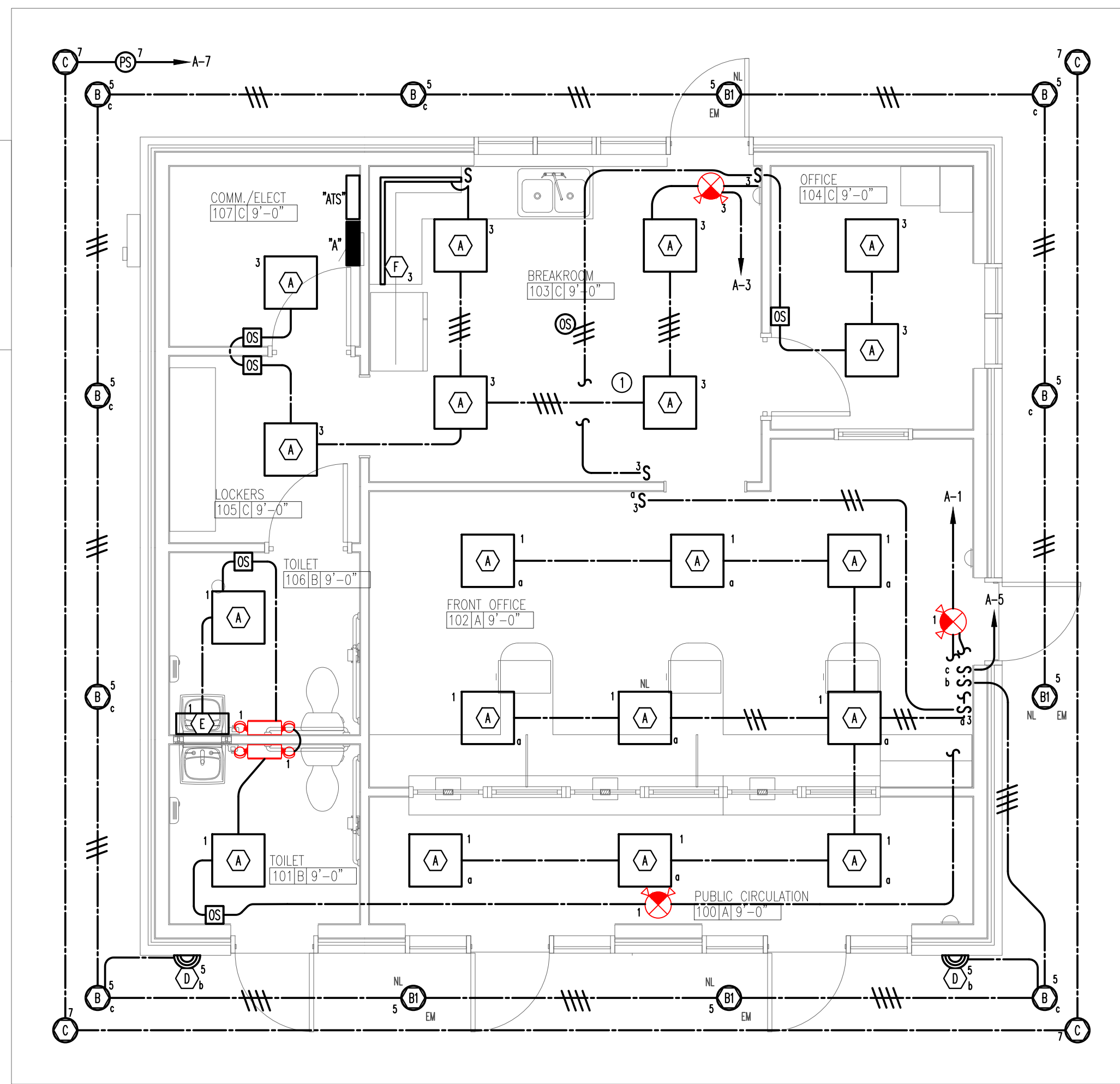
LIGHTING PLAN
