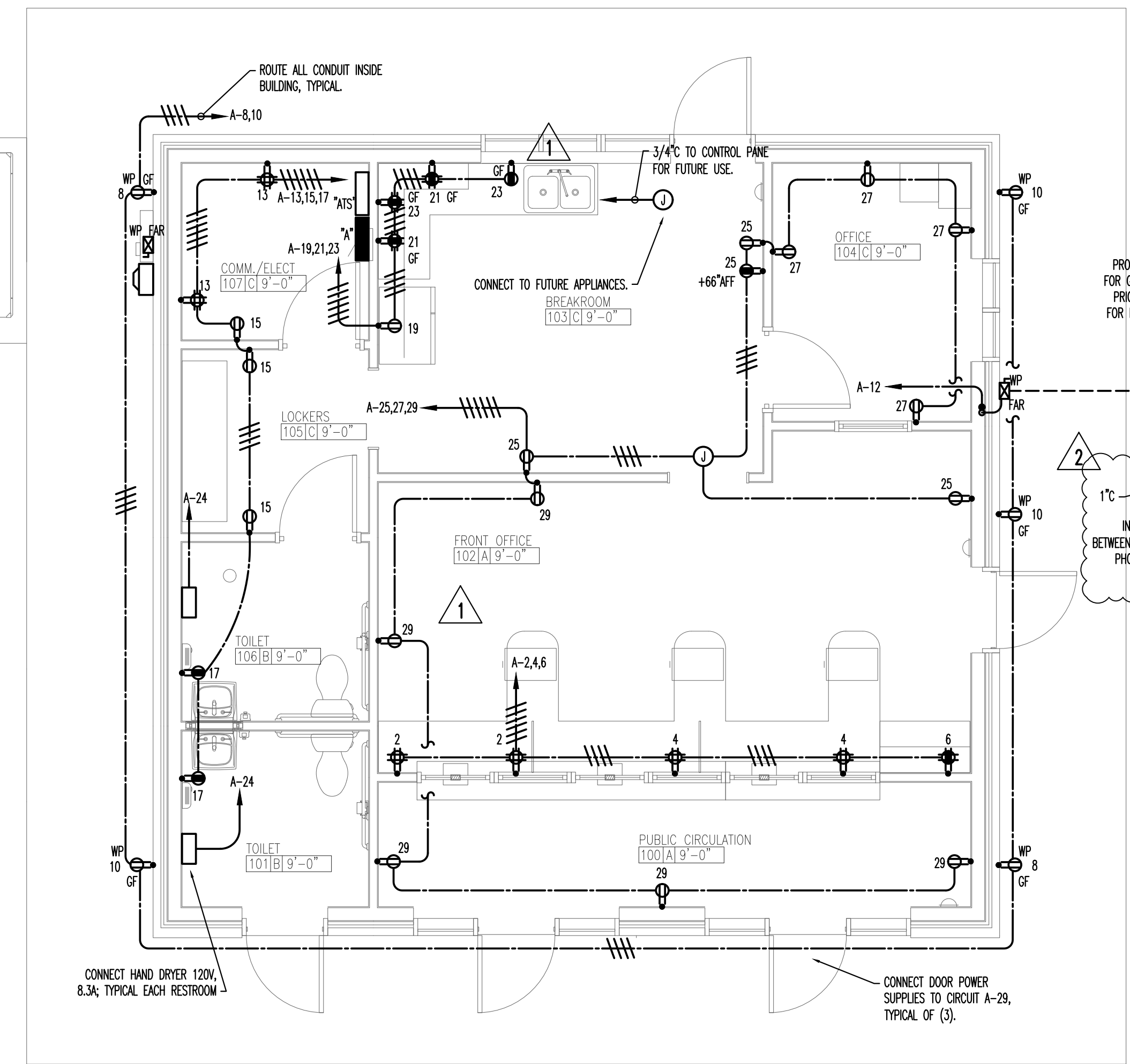
POWER PLAN
