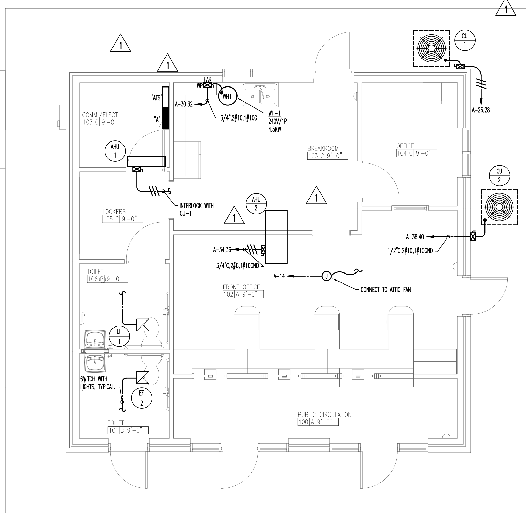
HVAC POWER PLAN
