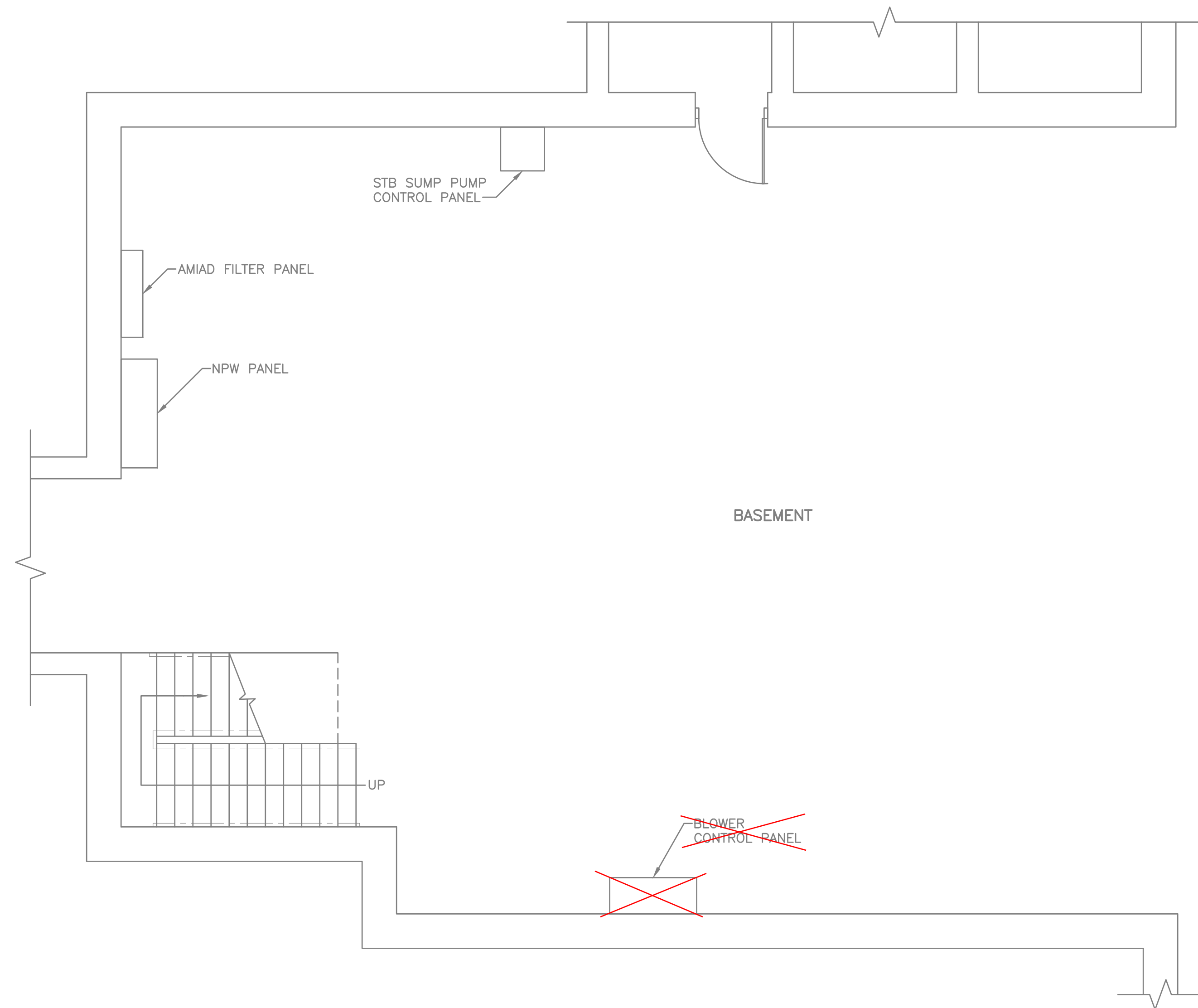
LOWER LEVEL ELECTRICAL PLAN
