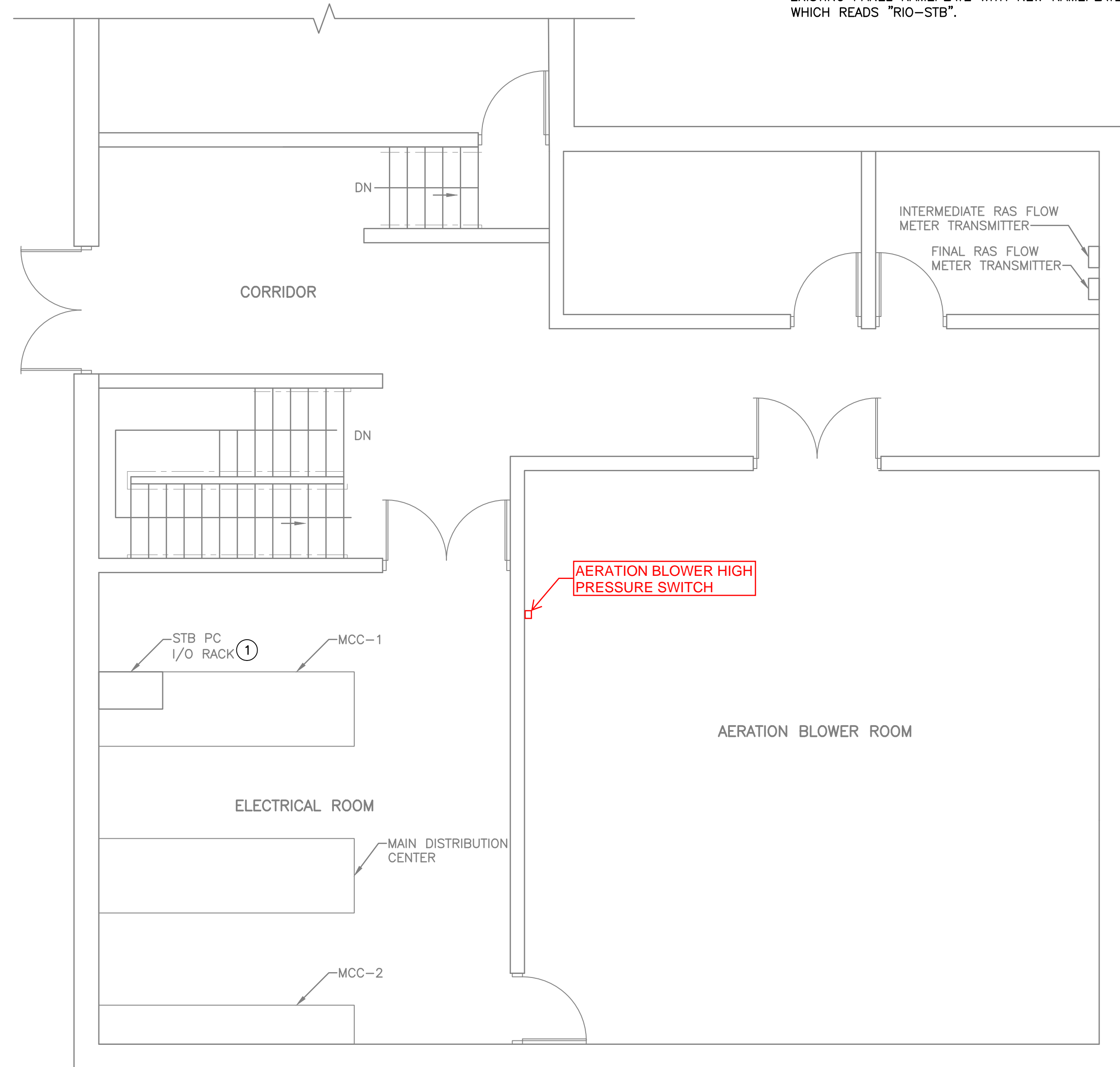
UPPER LEVEL ELECTRICAL PLAN
