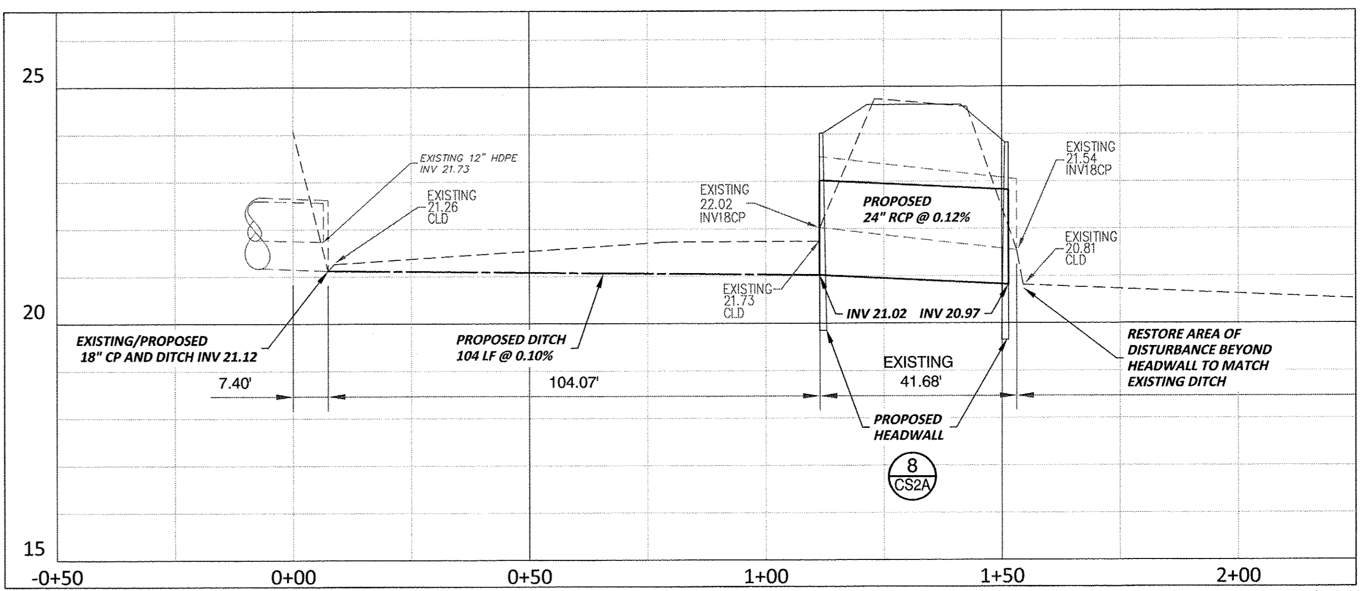
3 PROFILE - AREA 3 SCALE: 1" = 20'
