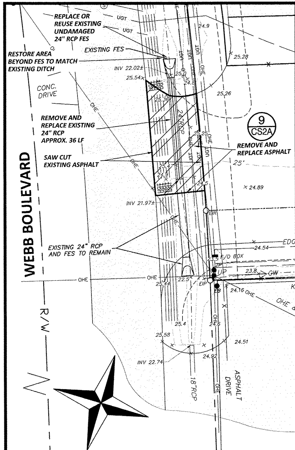
1 AREA 1 PLAN - CULVERT REPLACEMENT SCALE: 1" = 20'
