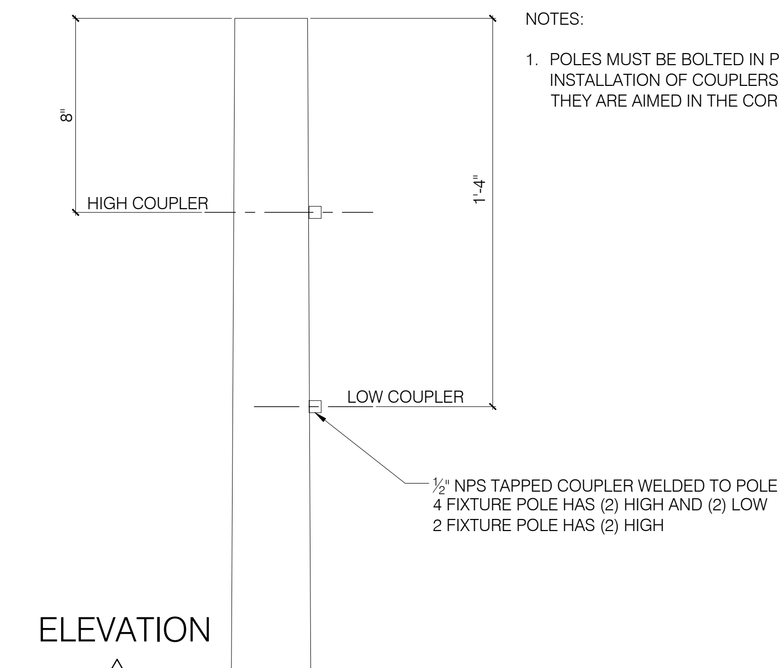
3 LP FIXTURE DETAILS L4.03 SCALE: 3" = 1'-0"
