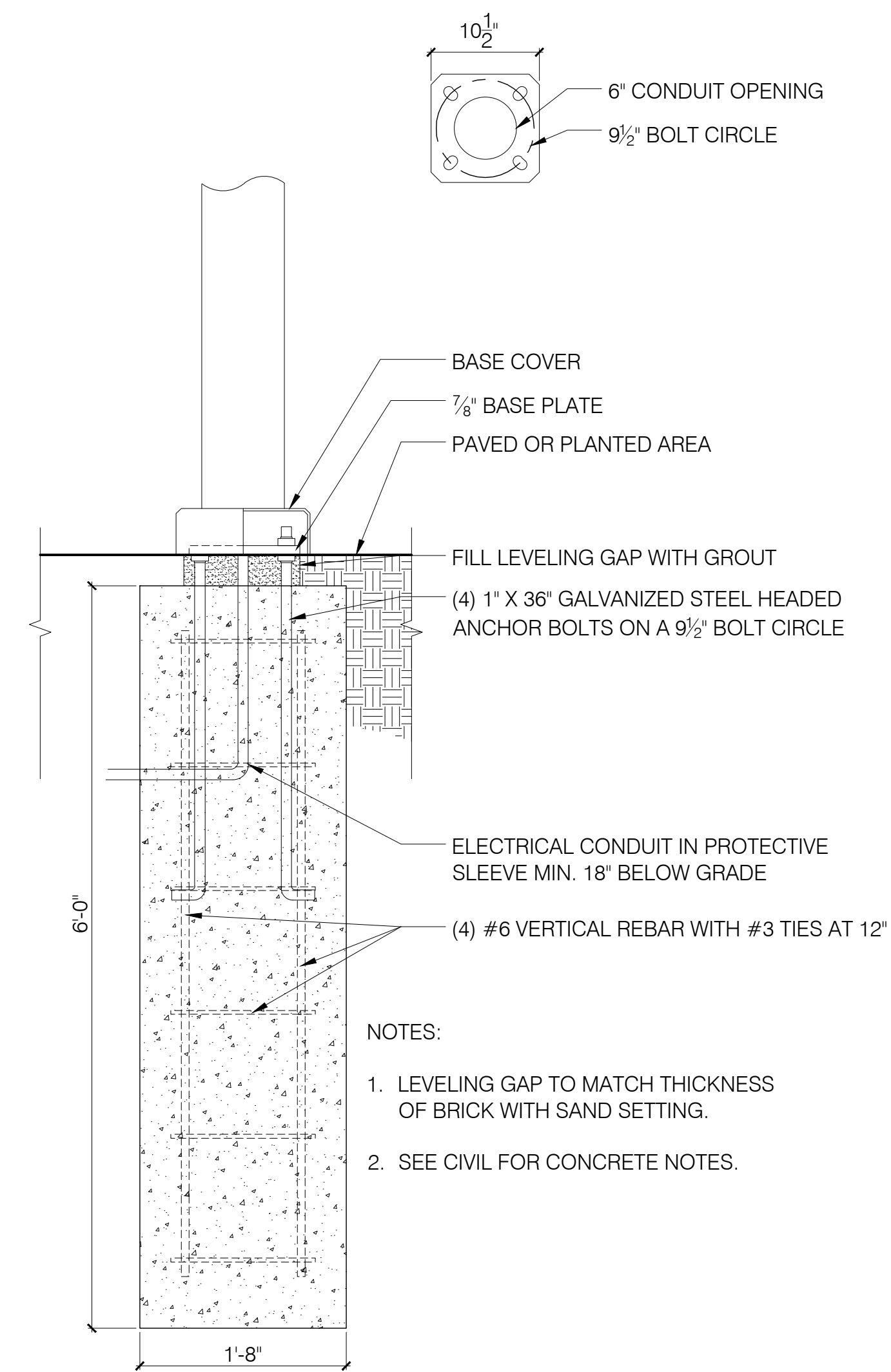
2 LIGHT POLE FOOTING - SECTION L4.03 SCALE: 1" = 1'-0"
