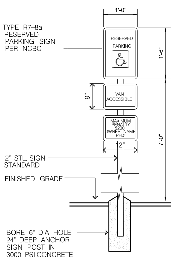
7 HANDICAP SIGN C2.1 NOT TO SCALE
