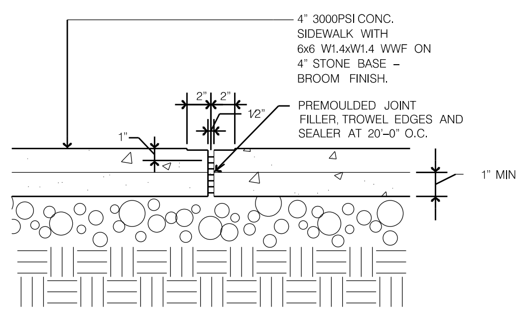
4 EXPANSION JOINT DETAIL C2.1 NOT TO SCALE
