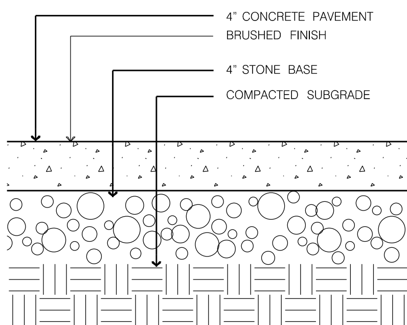
2 TYPICAL SIDEWALK SECTION C2.1 NOT TO SCALE
