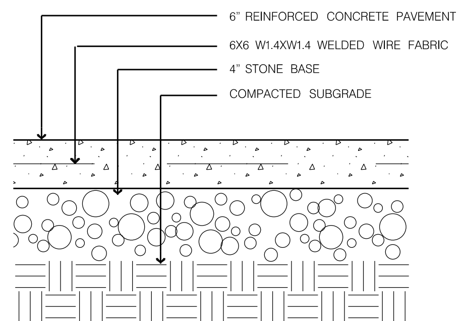
1 TYPICAL CONCRETE PAVING SECTION C2.1 NOT TO SCALE
