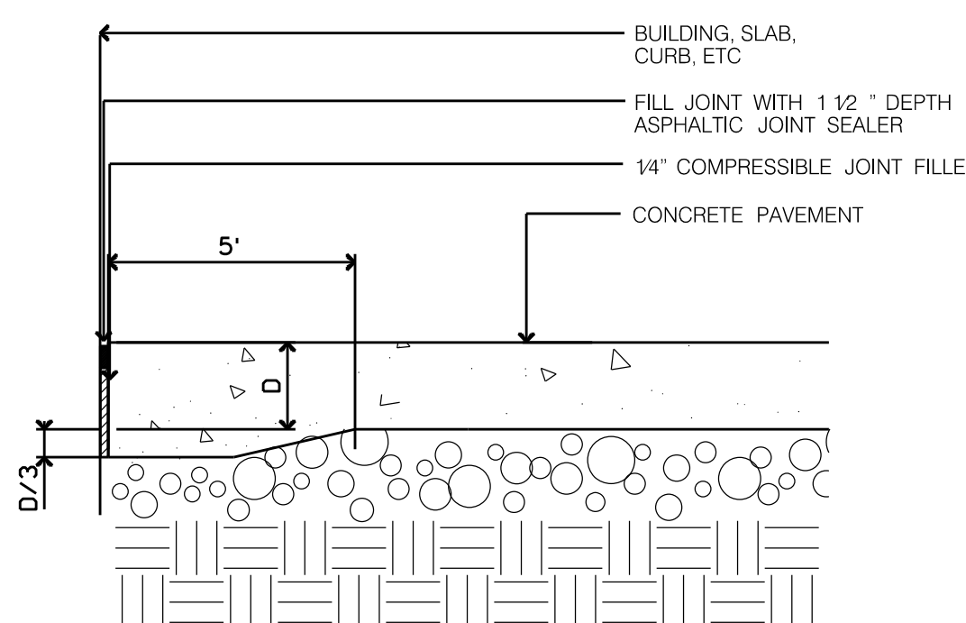
1 TYPICAL CONCRETE PAVING SECTION C2.1 NOT TO SCALE
