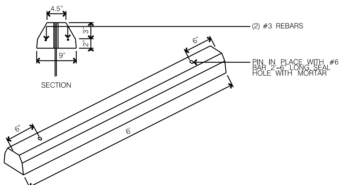
9 PRECAST CONCRETE WHEEL STOP C2.1 NOT TO SCALE
