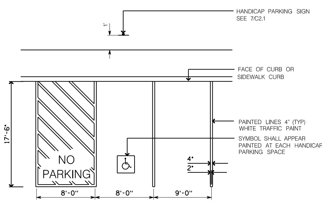
6 TYPICAL PARKING SPACE DETAIL C2.1 NOT TO SCALE
