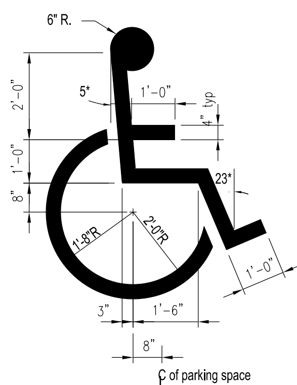
8 ACCESSIBILITY SYMBOL C2.1 NOT TO SCALE
