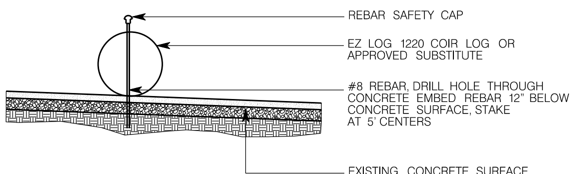
10 COIR LOG DETAIL C2.1 NOT TO SCALE
