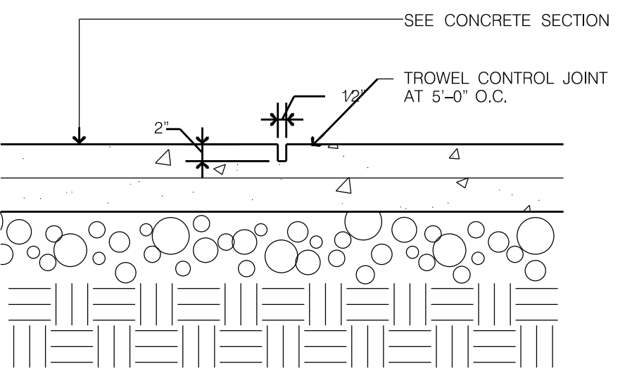
3 CONTROL JOINT DETAIL C2.1 NOT TO SCALE
