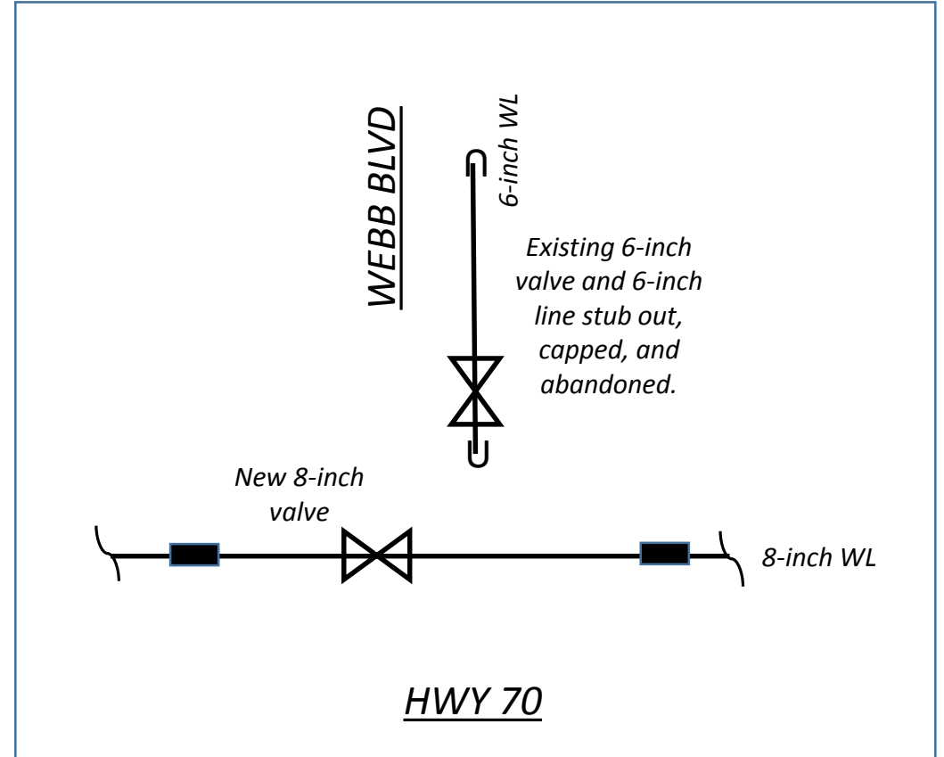
New Piping Configuration
