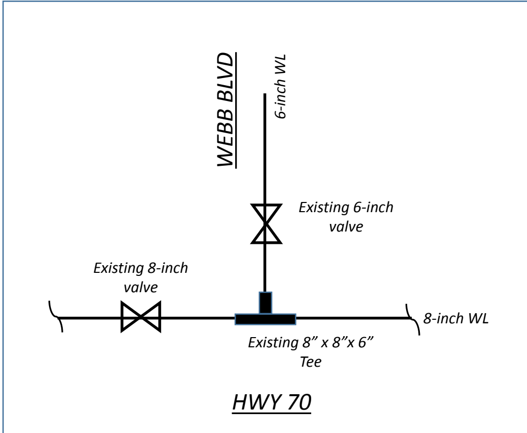
Existing Piping Configuration
