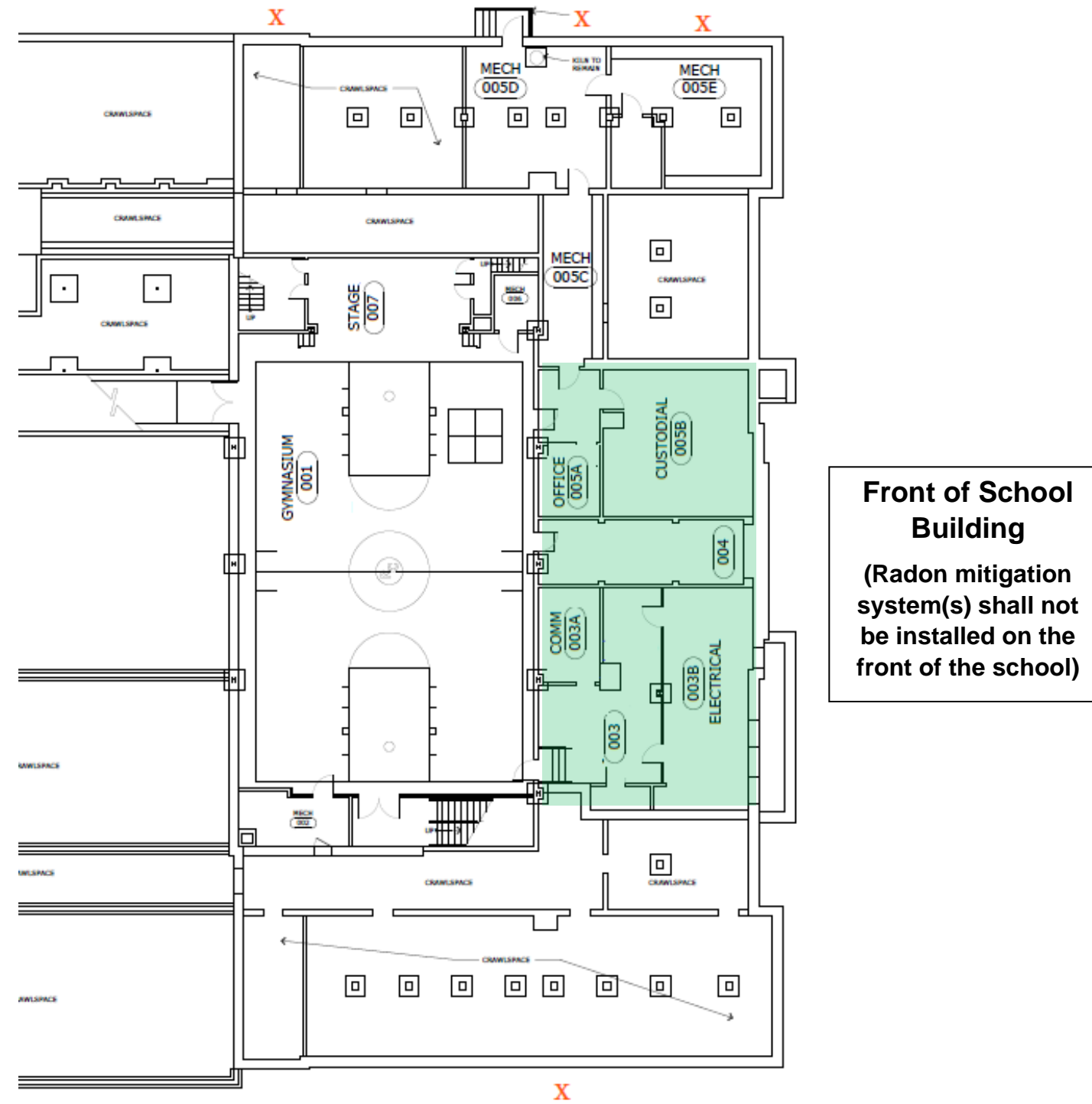
Figure 2: Figure 1: Targeted areas of Russell Cave Elementary School for ASD Radon Mitigation (Green). X - Current Radon Mitigation Systems Slab A above corresponds to the suction point in Appendix A: Radon Diagnostic Report.
