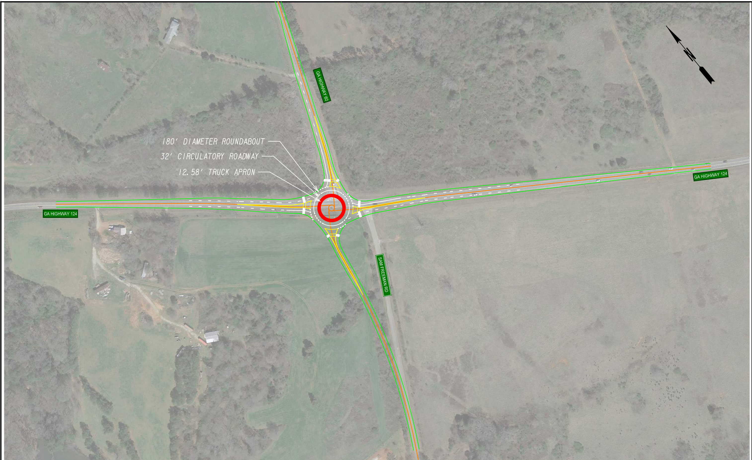
SR 60 AT SR 124 MULTILANE ROUNDABOUT DESIGN
