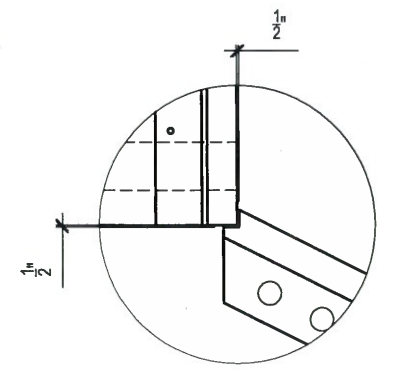
WINGWALL JOINT DETAIL SCALE: 1/4" = 1'-0"
