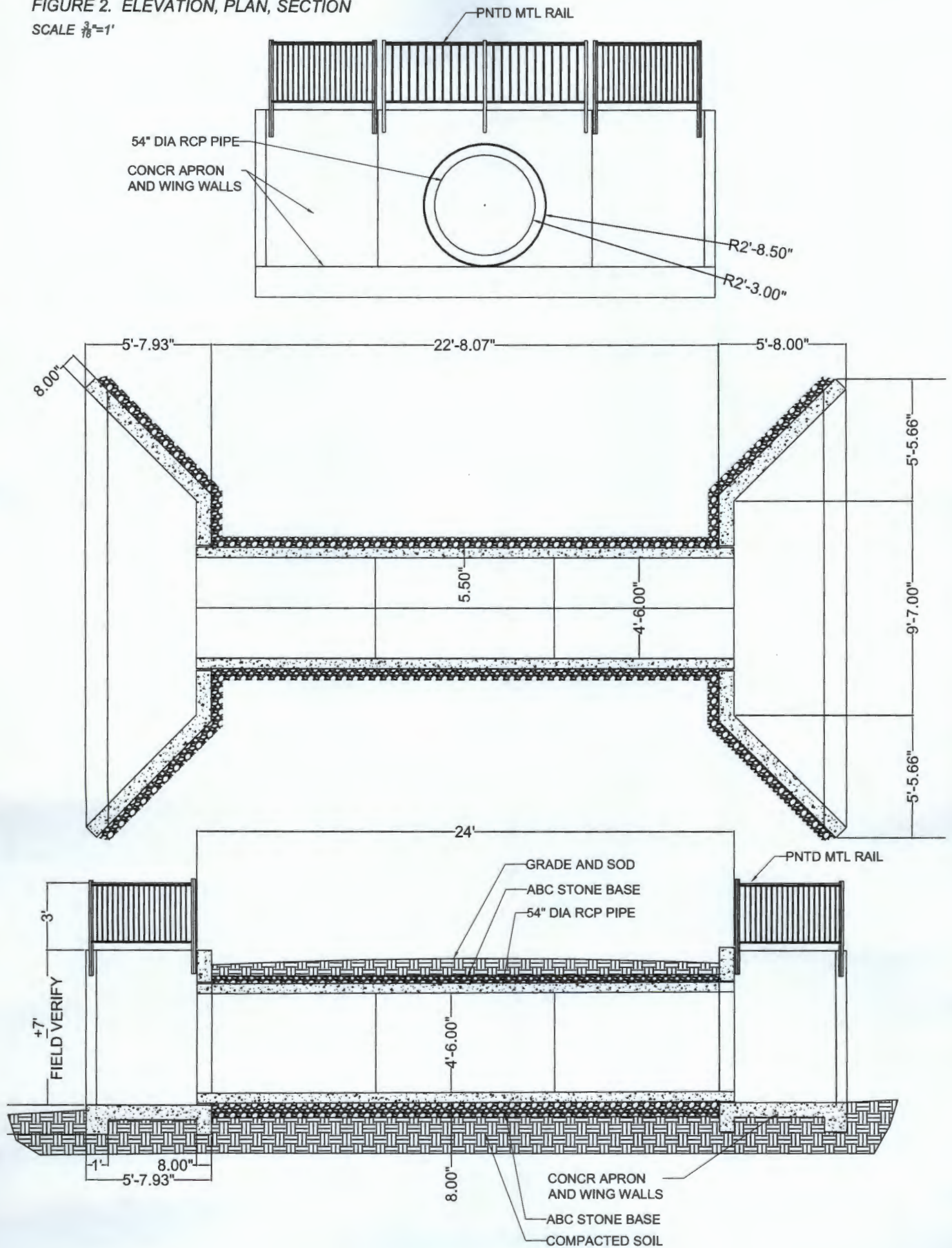
FIGURE 2. ELEVATION, PLAN, SECTION
