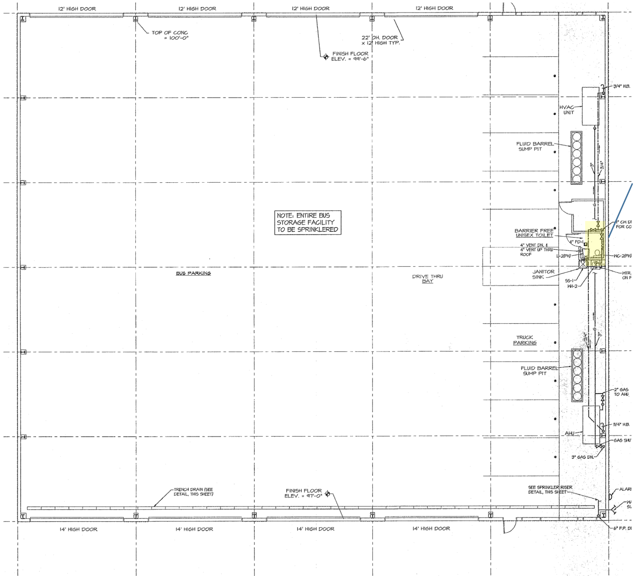
BUS STORAGE FACILITY PLUMBING FLOOR PLAN SCALE 1/8"=1'-0"
