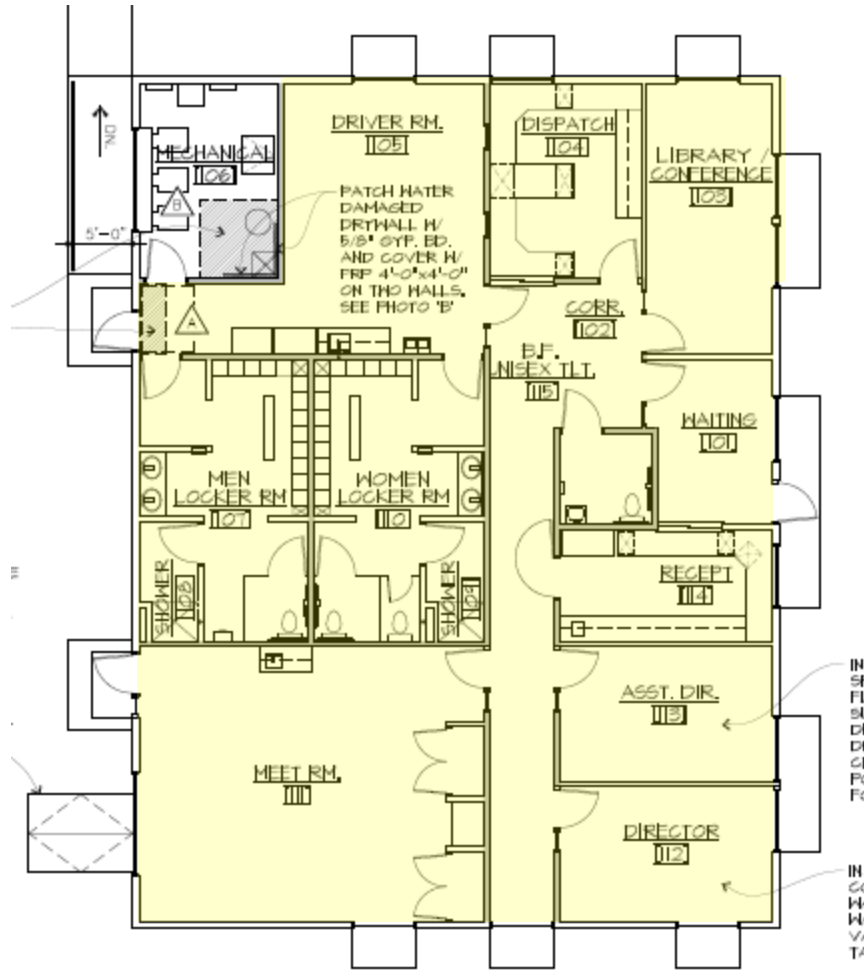
FLOOR PLAN ADMINISTRATION BUILDING SCALE 1/8" = 1'-0"
