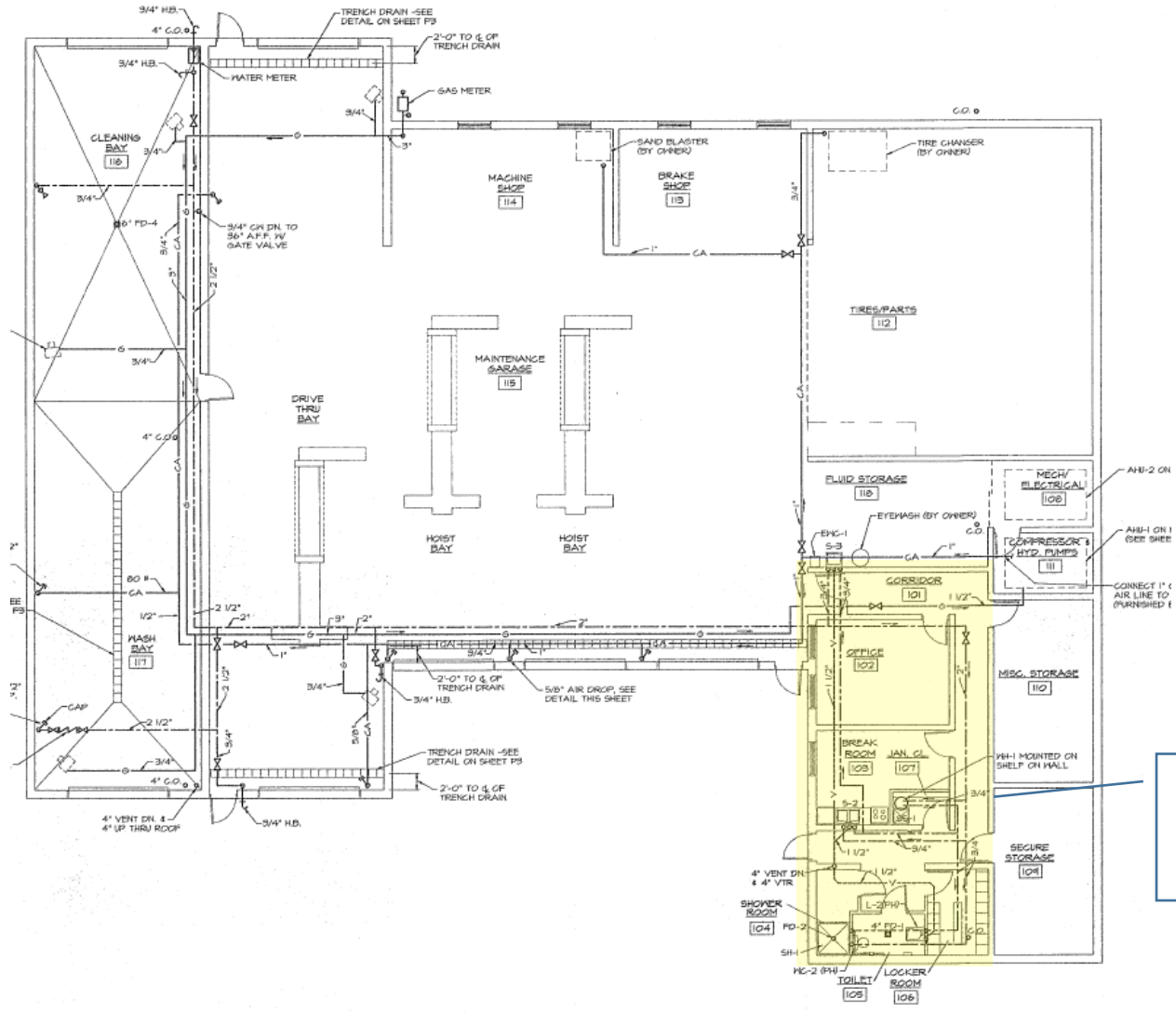
BUS MAINTENANCE FACILITY PLUMBING FLOOR PLAN SCALE 1/8"=1'-0"
