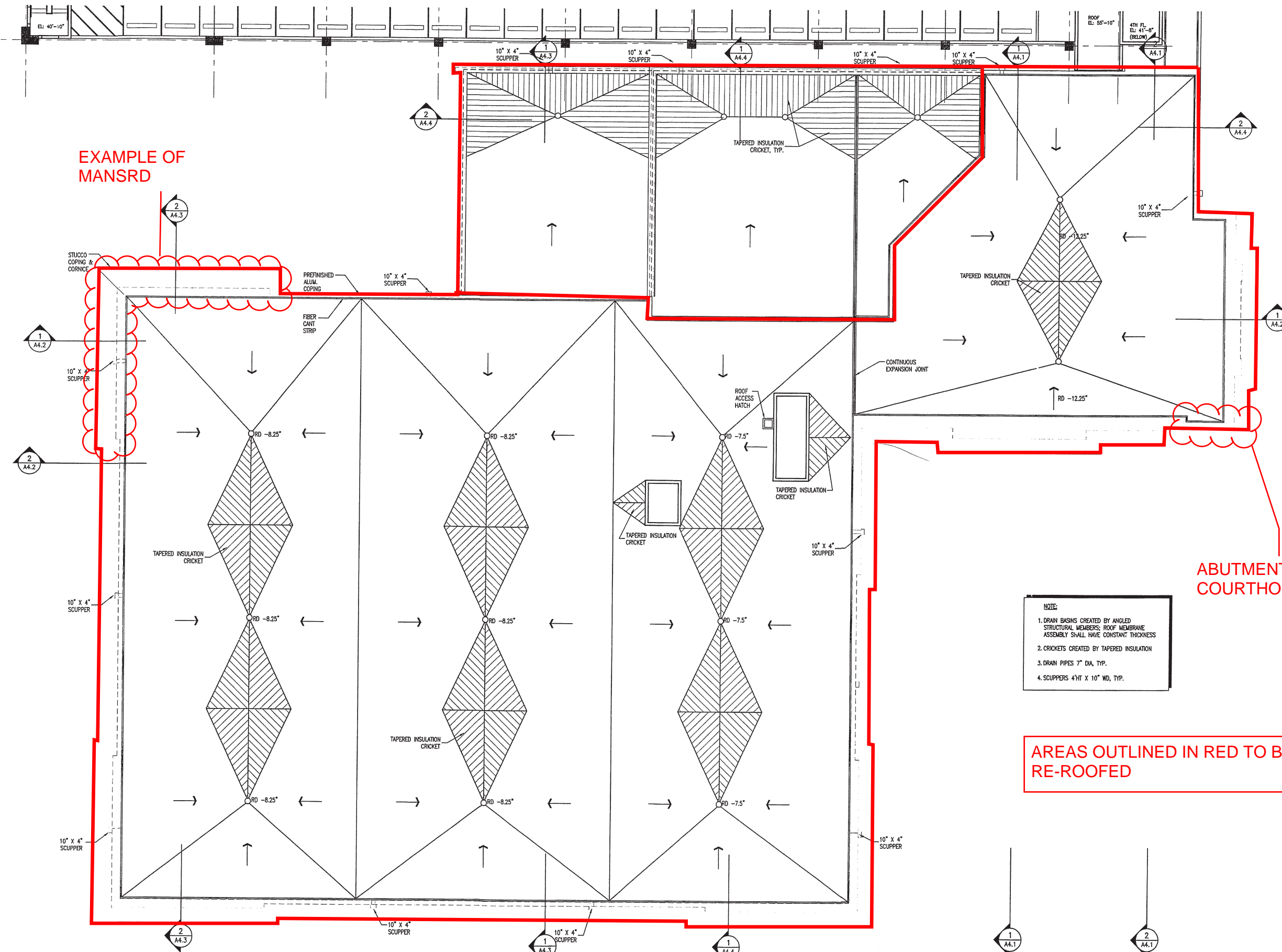
1 ROOF PLAN A1.5 SCALE: 3/32"=1'-0"
