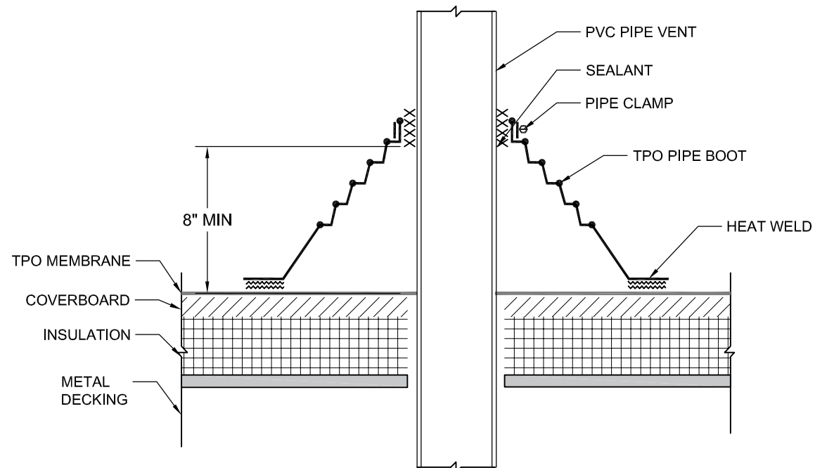
3 PIPE VENT FLASHING SCALE: NTS
