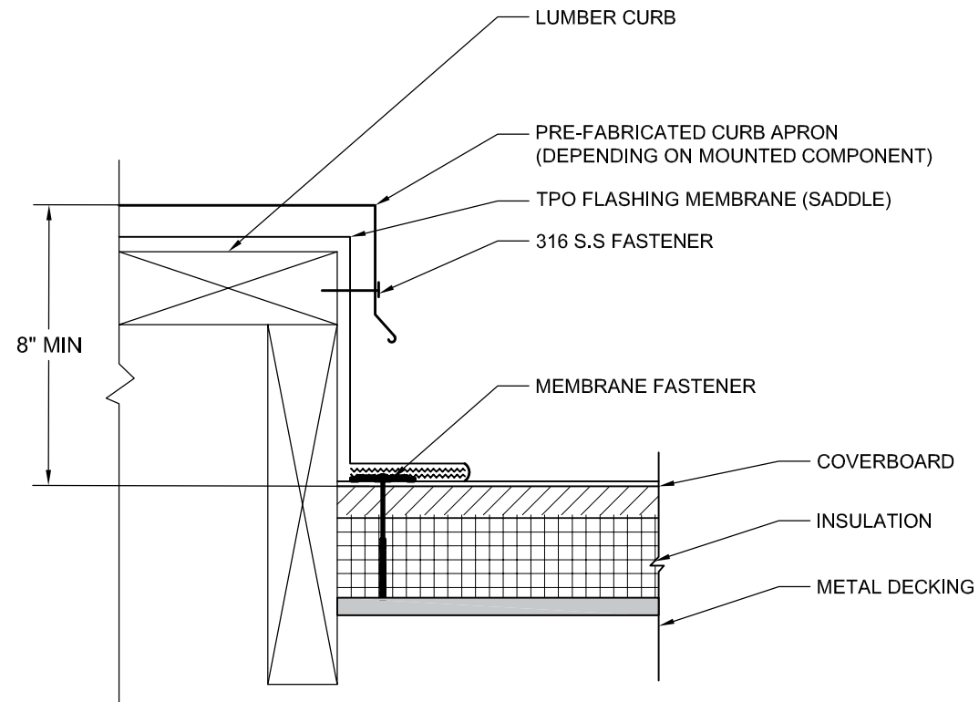
1 ROOFTOP CURB FLASHING SCALE: NTS
