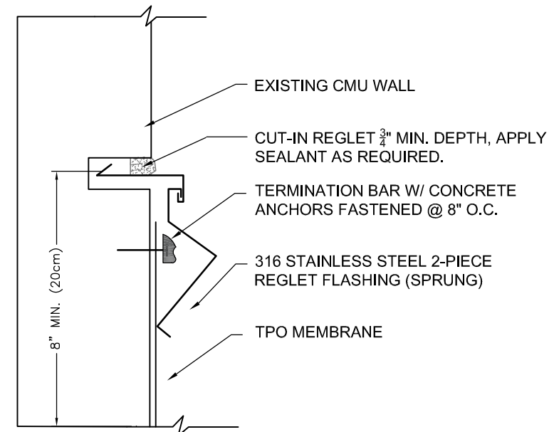
2 ROOF TO CMU WALL FLASHING SCALE: NTS
