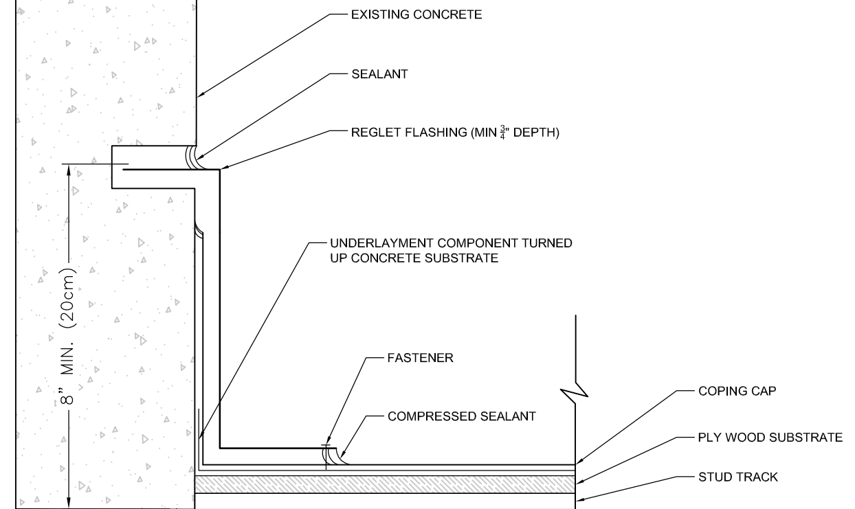
2 COPING TO CONCRETE WALL FLASHING SCALE: NTS
