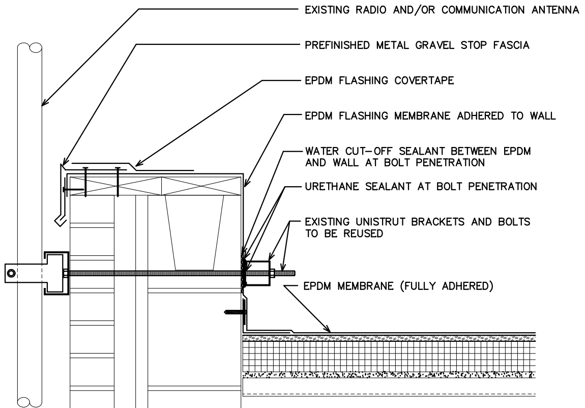
(A) ANTENNA SUPPORT AT PENTHOUSE "B"
