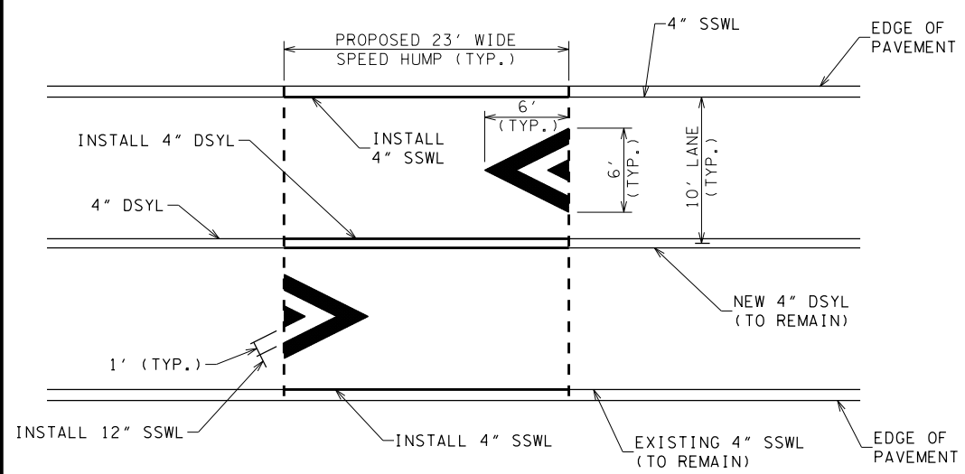
PROPOSED SPEED HUMP PAVEMENT MARKING DETAIL NOT TO SCALE
