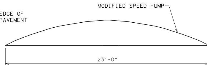
TYPICAL SPEED HUMP CROSS SECTION NOT TO SCALE
