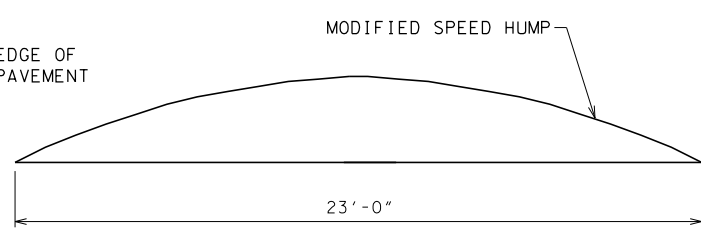
TYPICAL SPEED HUMP CROSS SECTION NOT TO SCALE
