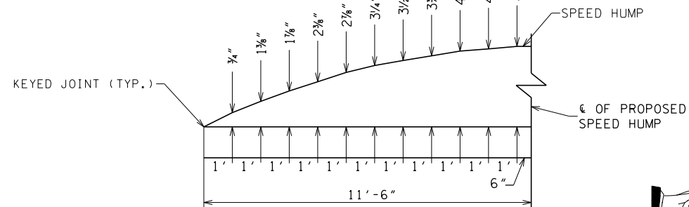
MODIFICATION DETAIL
