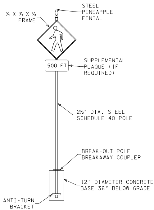
STEEL SIGN POLE (TRAFFIC SIGN) NOT TO SCALE
