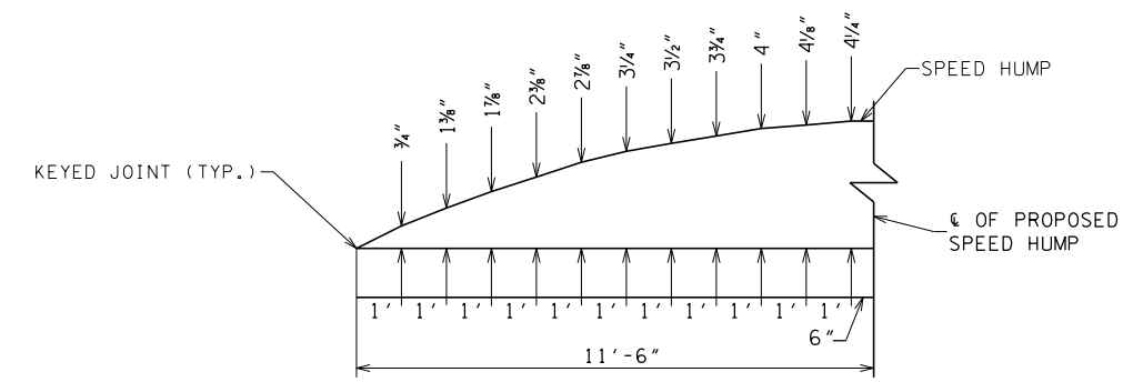
MODIFICATION DETAIL NOT TO SCALE
