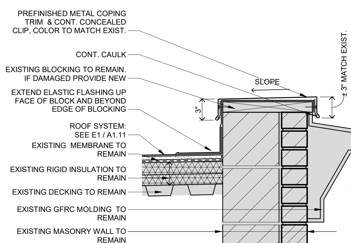
E4 COPING DETAIL 1 1/2" = 1'-0" 0 1/2 1'
