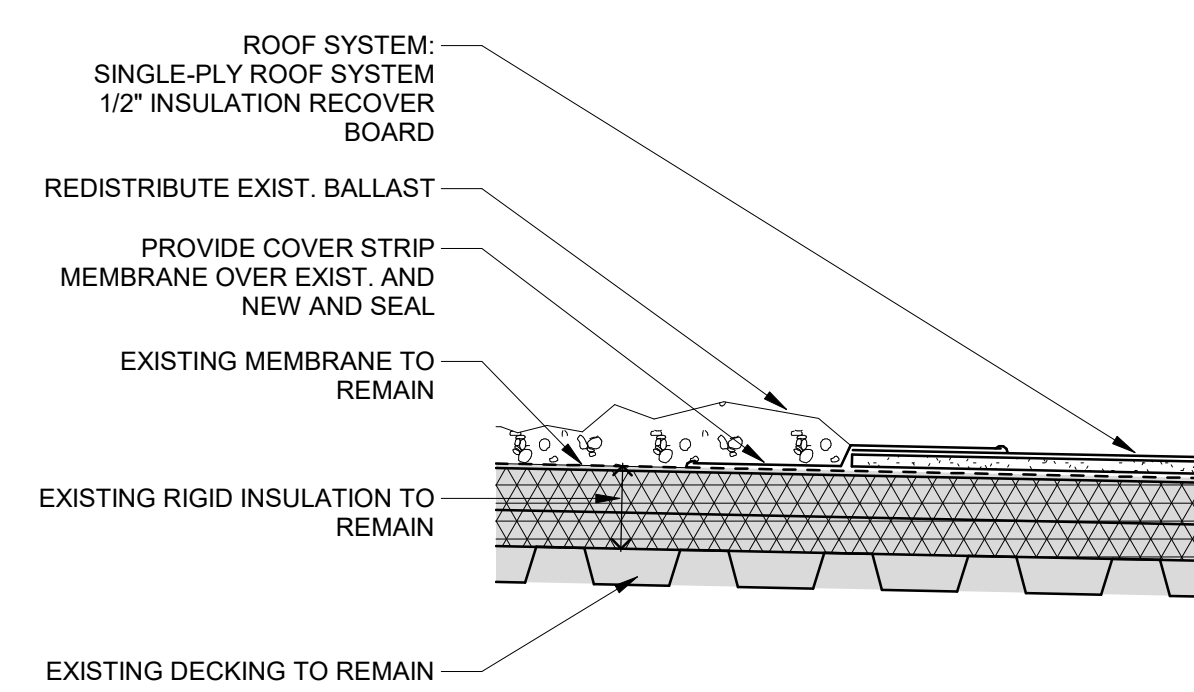
E1 TRANSITION DETAIL 1 1/2" = 1'-0" 0 1/2 1'
