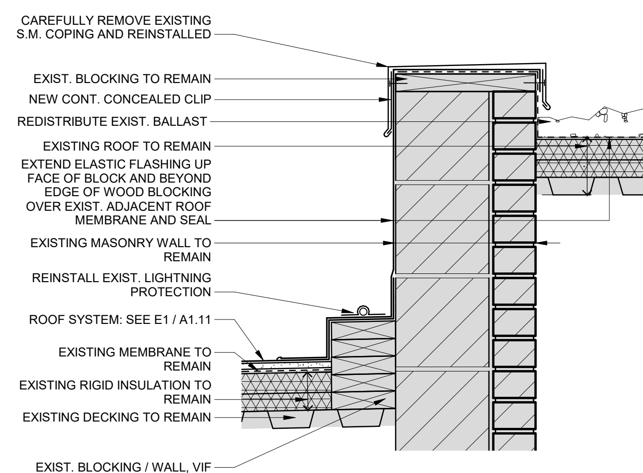
F4 COPING DETAIL 1 1/2" = 1'-0" 0 1/2 1'
