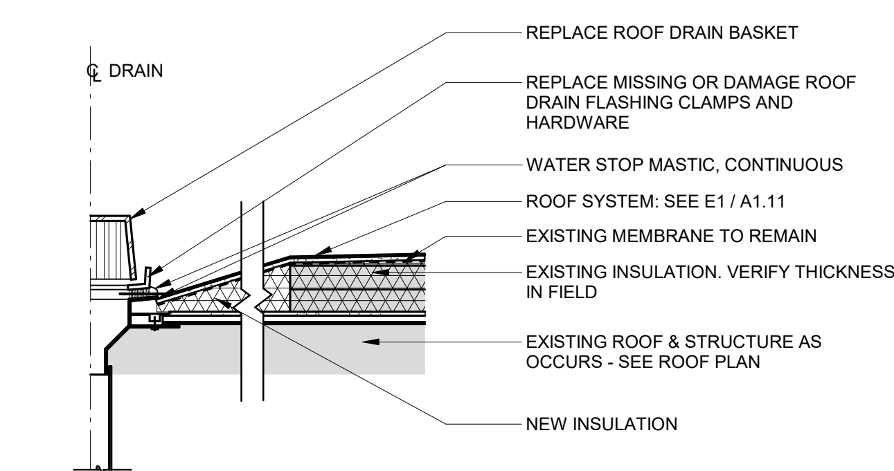
B5 ROOF DRAIN SUMP SECTION 3/4" = 1'-0" 0 1 2'
