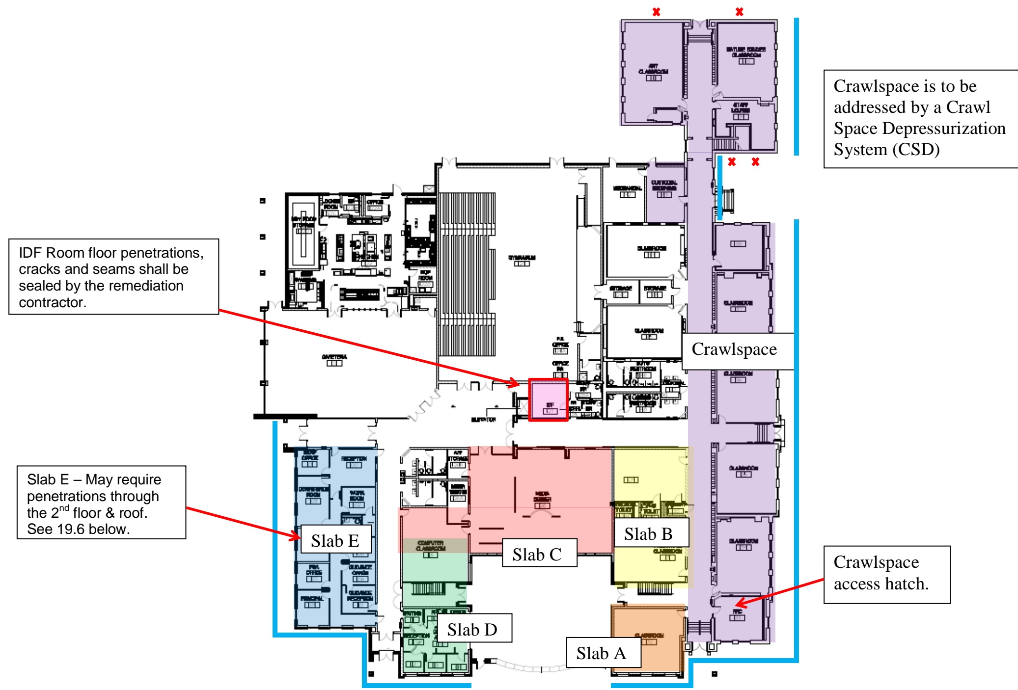
Figure 1: Targeted areas of Arlington Elementary School for ASD Radon Mitigation are identified above. Each color should be considered as one contiguous slab segment. The crawlspace areas are identified by the purple shading. The X's identify crawlspace vents. No radon fans or piping shall be placed on exterior walls identified by the blue lines above.
