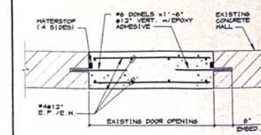
4 PLAN DETAIL OF DOOR IN-FILL
