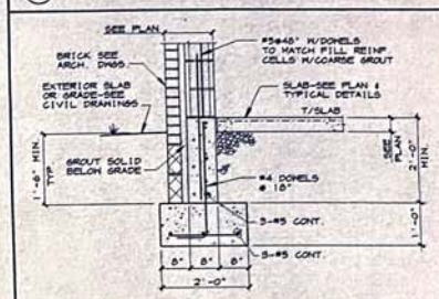
2 SECTION AT EXTERIOR WALL FOOTING (AT 8\"/>
