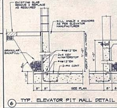
6 TYP. ELEVATOR PIT WALL DETAIL
