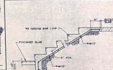
E CONCRETE STAIR ON GRADE
