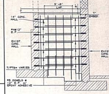
5 SECTION AT STAIR
