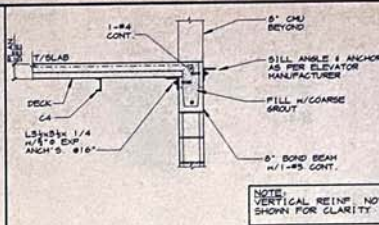
7 SECTION AT ELEVATOR DOOR
