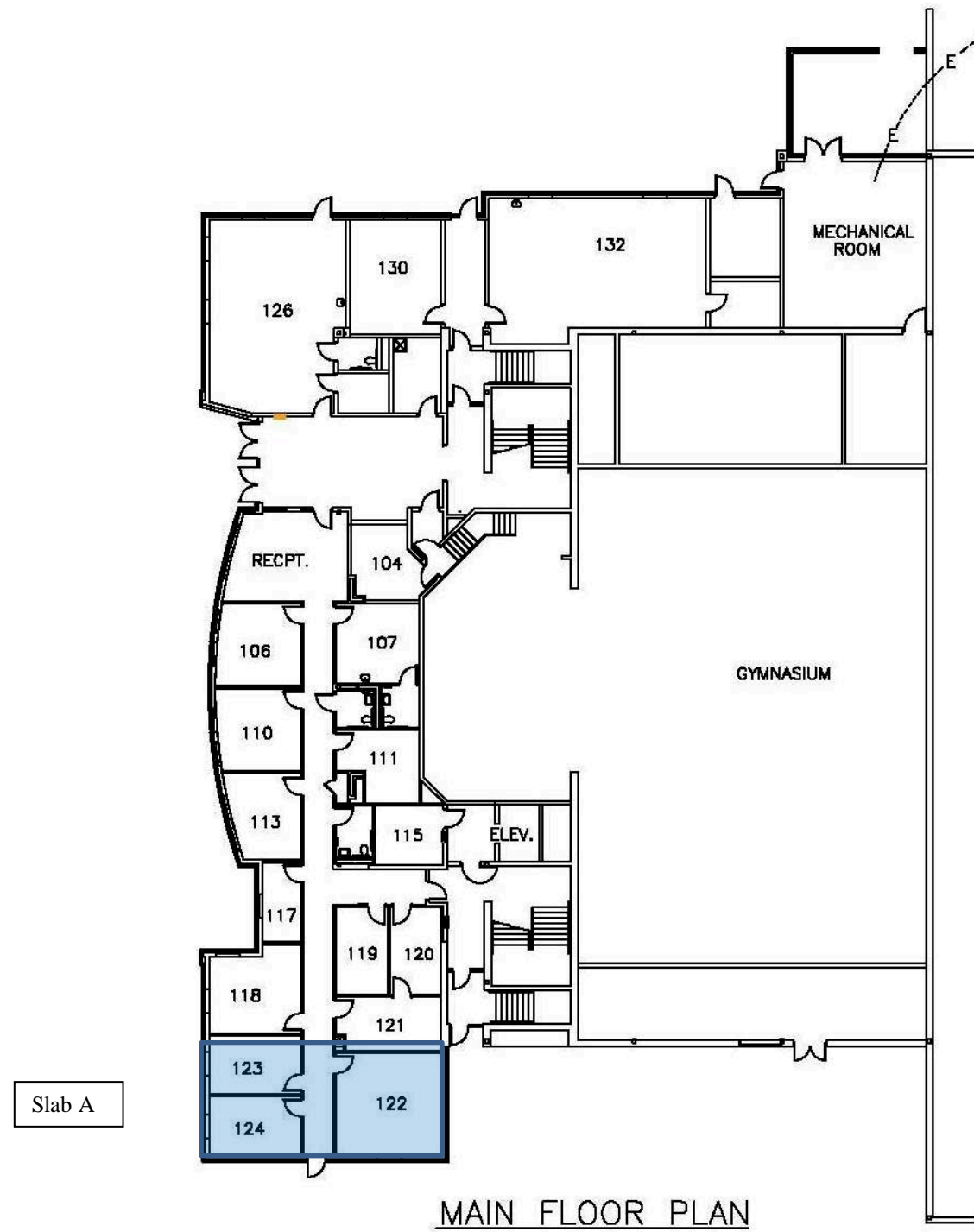
Figure 1: Targeted areas of Picadome Elementary School for ASD Radon Mitigation (Blue). Slab A above corresponds to the suction point in Appendix A: Radon Diagnostic Report. Each color should be considered as one contiguous slab segment.
