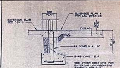
3 SECTION AT EXTERIOR DOOR
