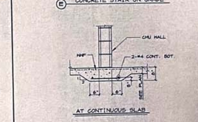
D THICKENED SLAB AT NON-LOADBEARING CMU WALLS
