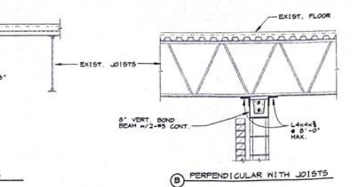
B PERPENDICULAR WITH JOISTS
