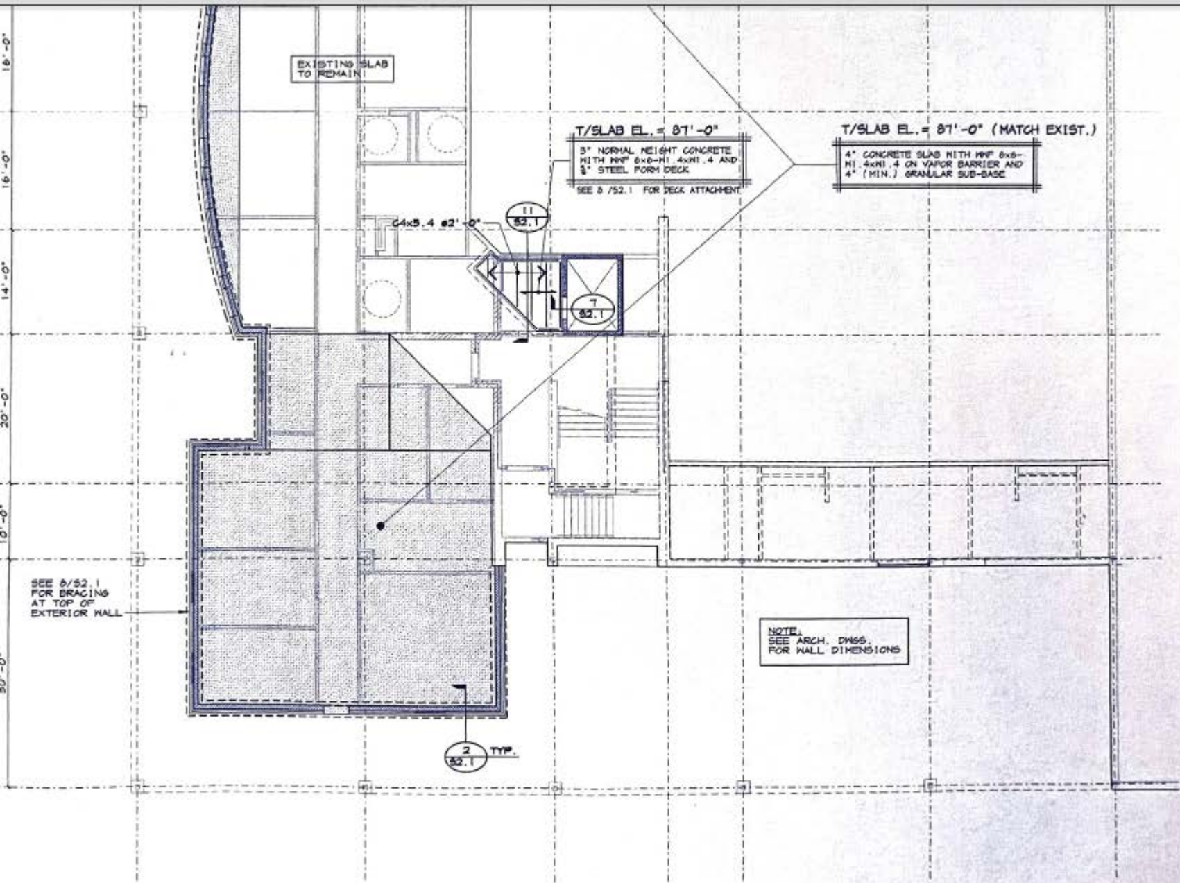
GROUND LEVEL FLOOR PLAN
