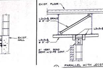
A PARALLEL WITH JOISTS
