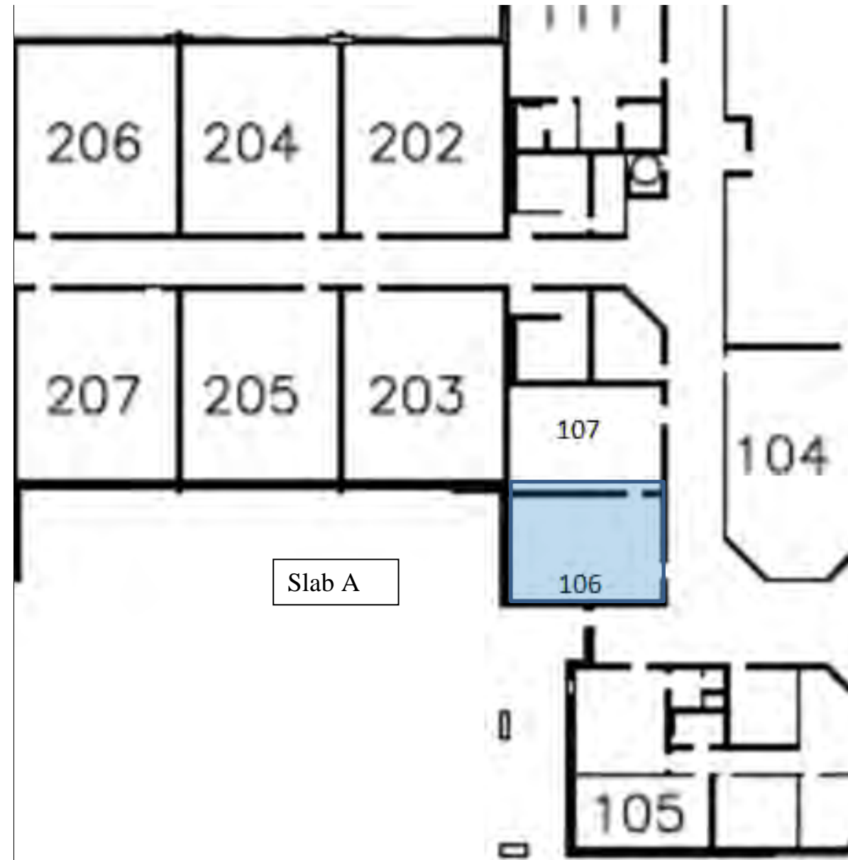
Figure 1: Targeted area of Rosa Parks Elementary School for ASD Radon Mitigation (Blue). Slab A above corresponds to the suction point in Appendix A: Radon Diagnostic Report. Each color should be considered as one contiguous slab segment.
