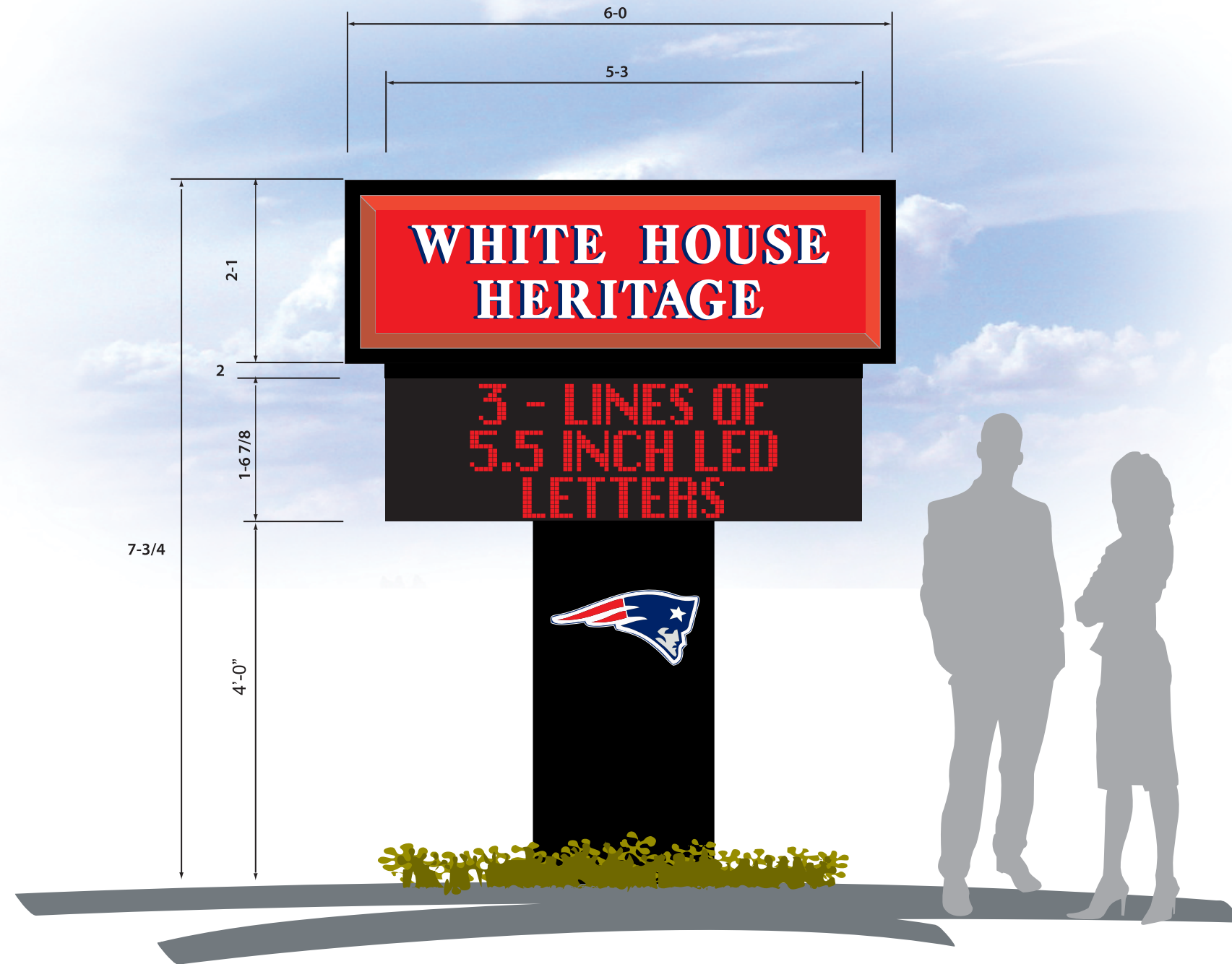
DOUBLE FACE ILLUMINATED MONUMENT SIGN (ELEVATION)
