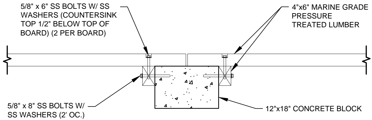
C1 NORTHERN CROSS OVER 1 SCALE: 3/4" = 1'-0"
