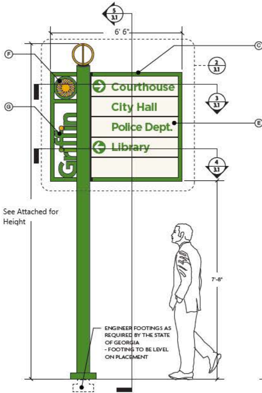
1 VEHICULAR DIRECTIONAL - FRONT ELEVATION SCALE: 1/2" = 1'-0"
