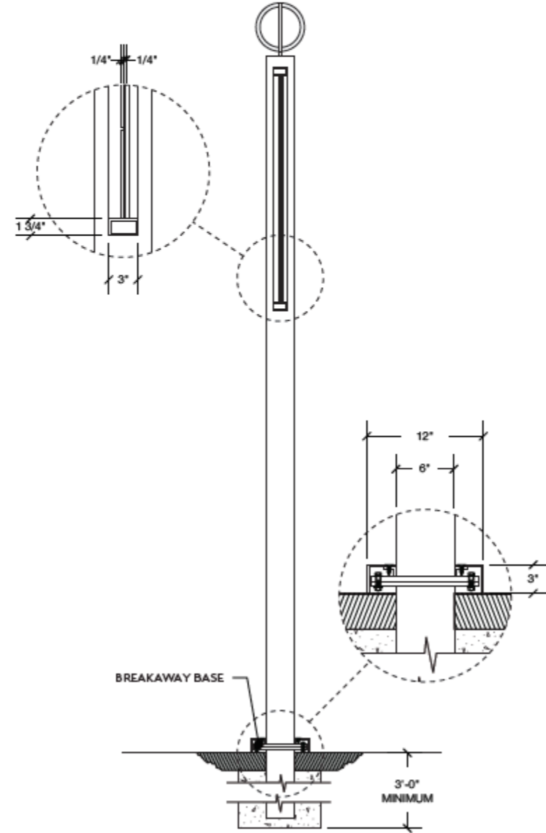
5 SECTION VIEW SCALE: 3/4"=1'-0"
