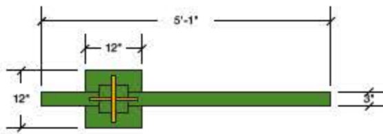
4 VEHICULAR DIRECTIONAL - PLAN VIEW SCALE: 1/2" = 1'-0"
