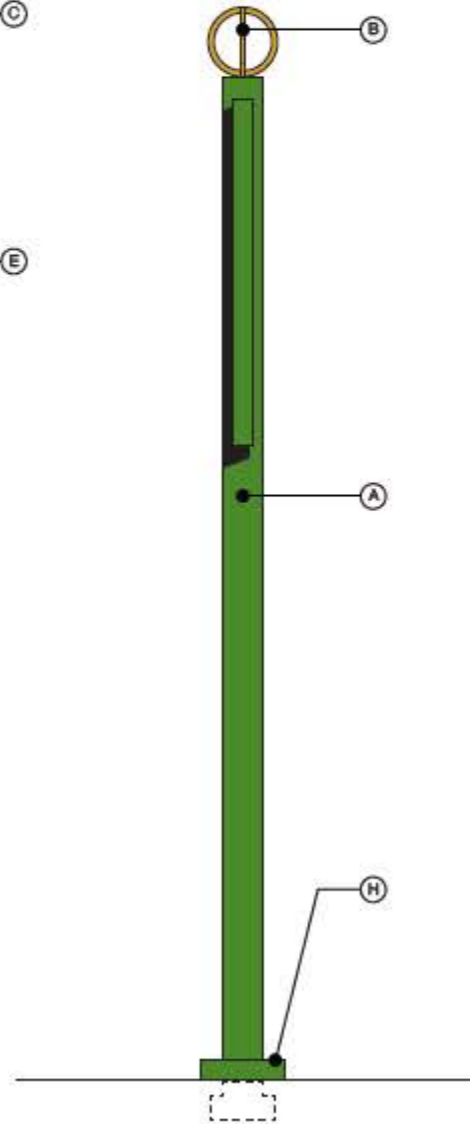
2 VEHICULAR DIRECTIONAL - SIDE ELEVATION SCALE: 1/2" = 1'-0"
