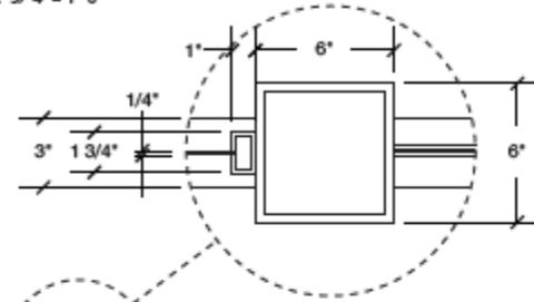
4 SECTION VIEW SCALE: 3/4"=1'-0"
