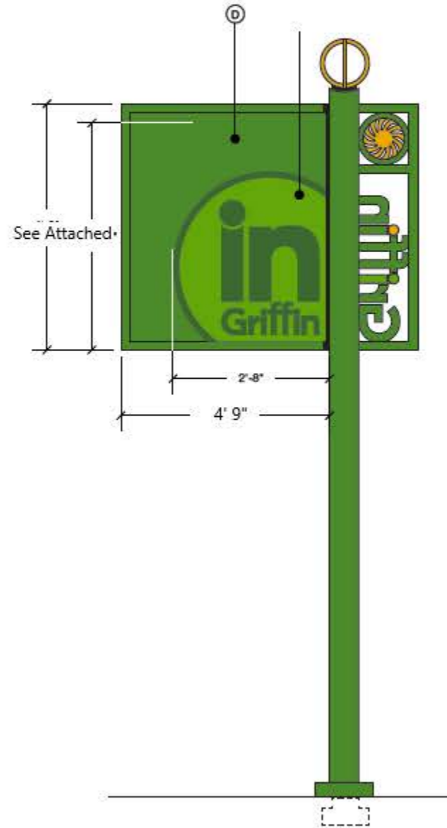
3 VEHICULAR DIRECTIONAL - BACK ELEVATION SCALE: 1/2" = 1'-0"
