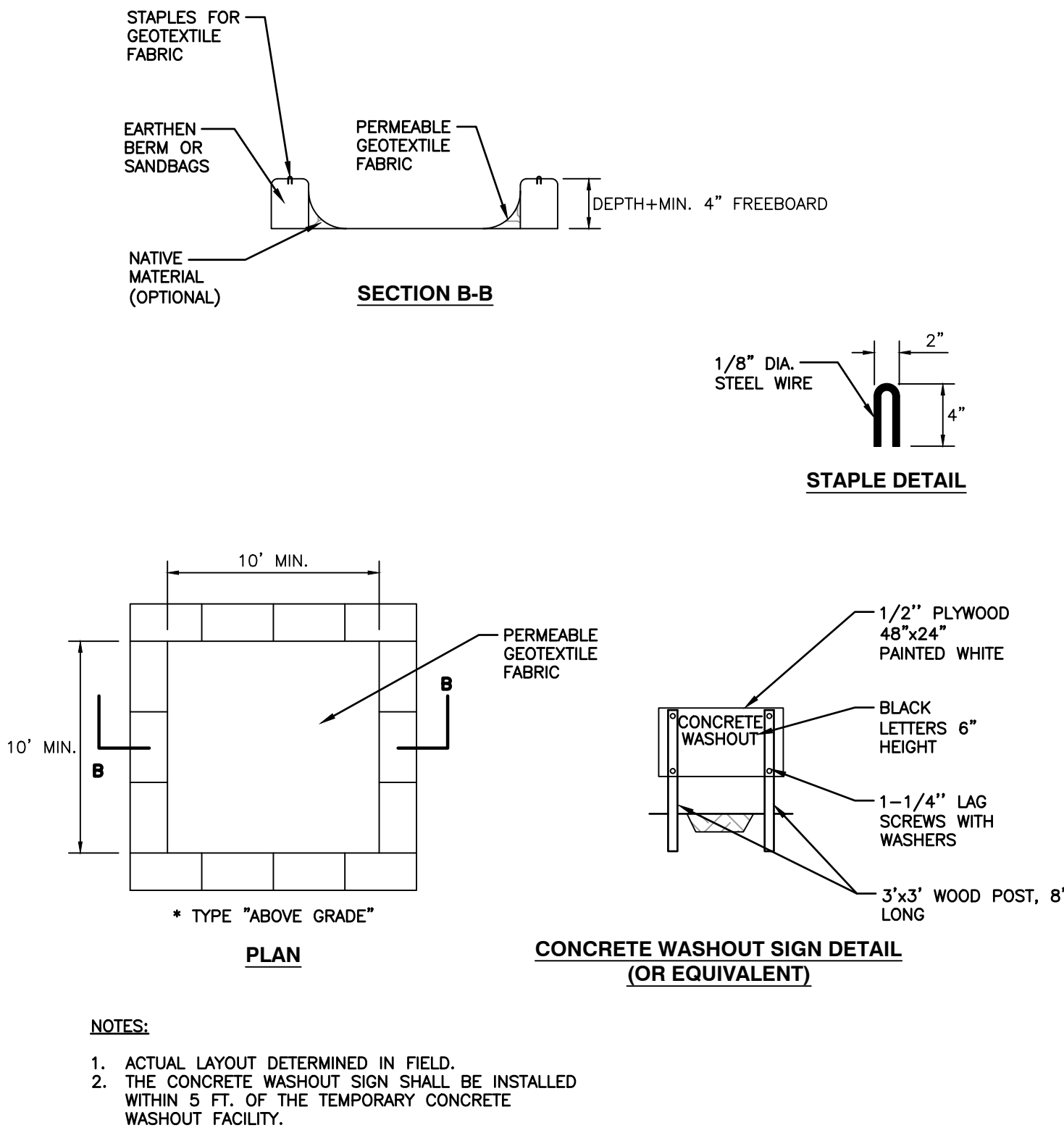
DETAIL 807 CONCRETE WASHOUT FACILITY N.T.S.
