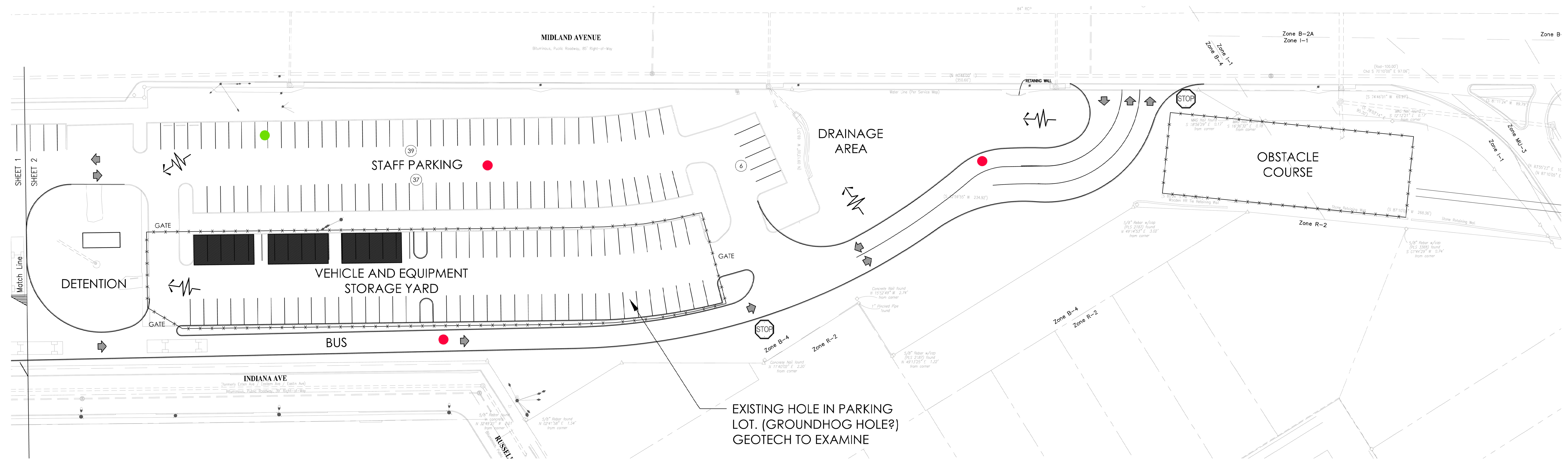
FCPS CTC - EAST SCALE 1" = 30'-0"
