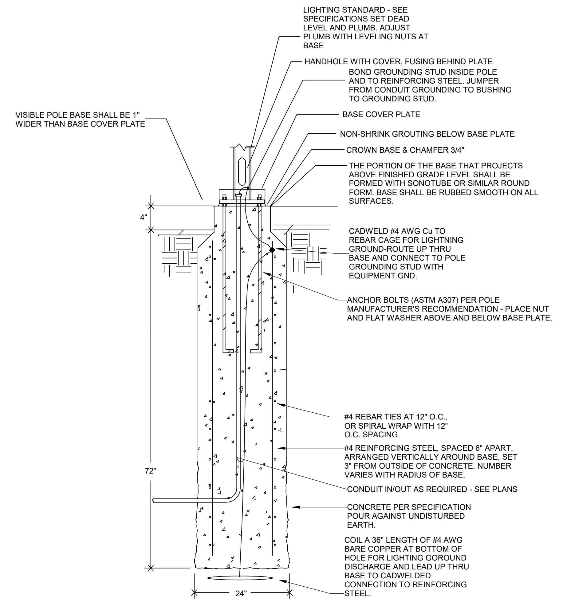
2 LIGHTING STANDARD BASE DETAIL SCALE: NONE
