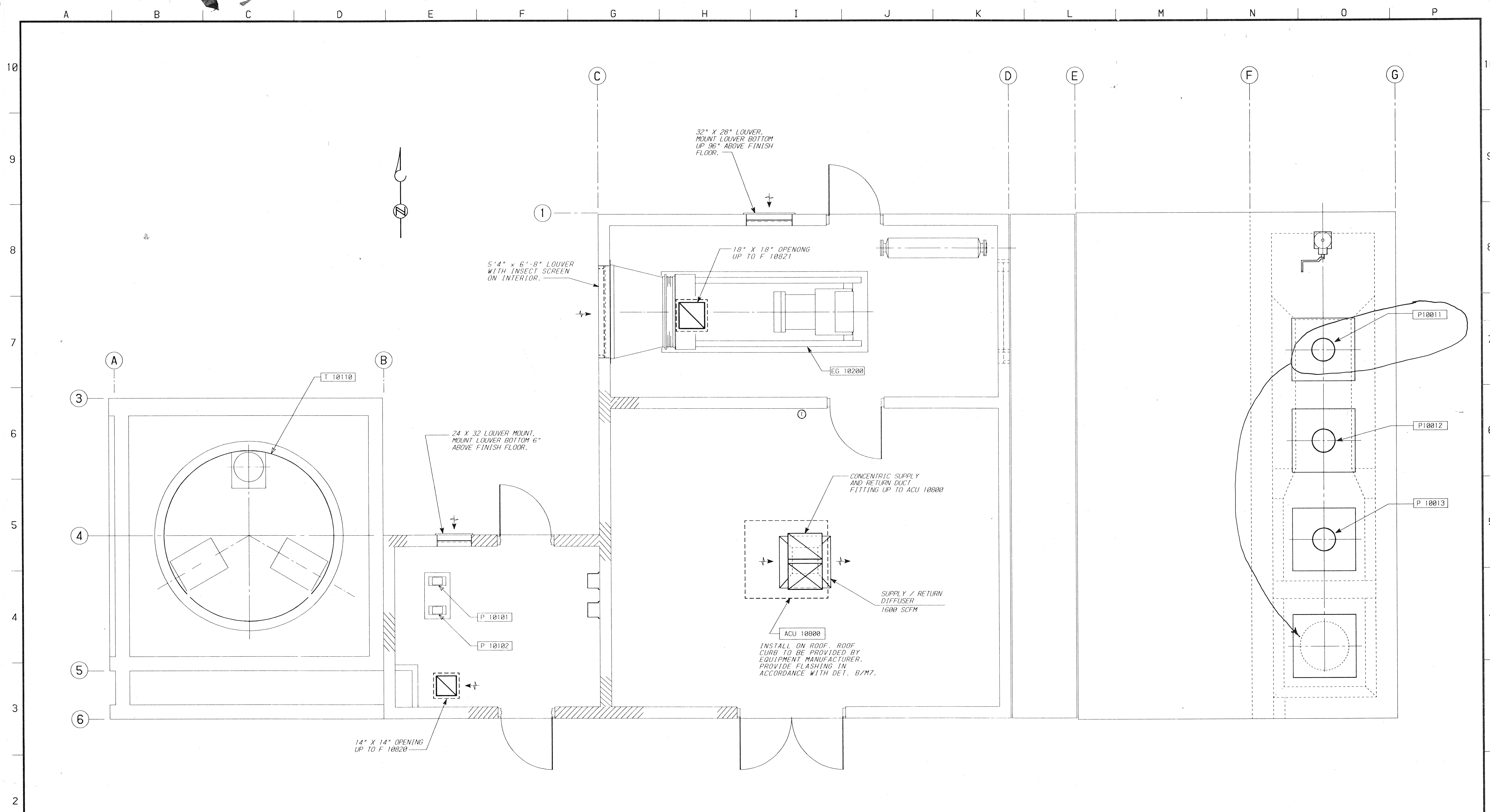
HVAC PLAN SCALE: 3/8"=1'-0"
