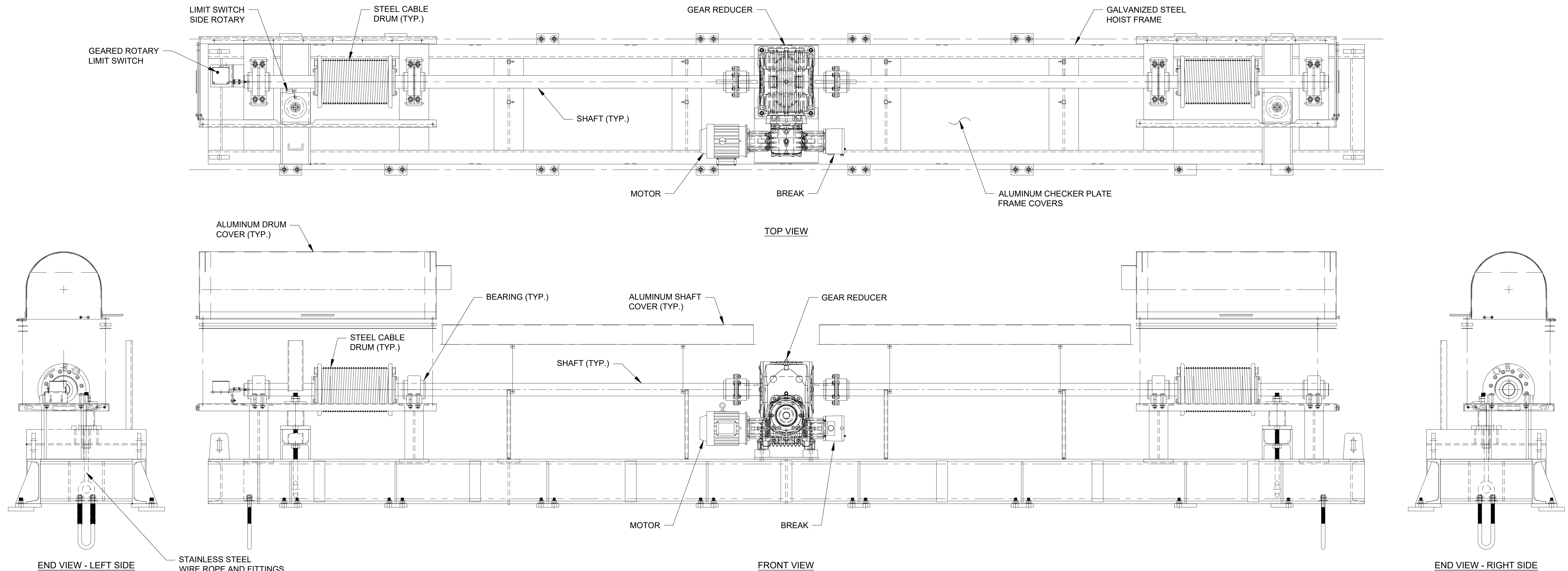
S1 CABLE HOIST ASSEMBLY (2 REQ'D. BY OTHERS) NOT TO SCALE
