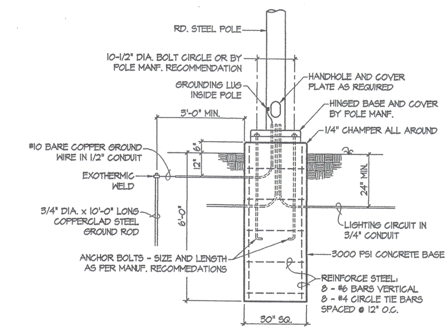
CONCRETE BASE DETAIL FIXTURES "H1", "H2" & "M3" NOT TO SCALE
