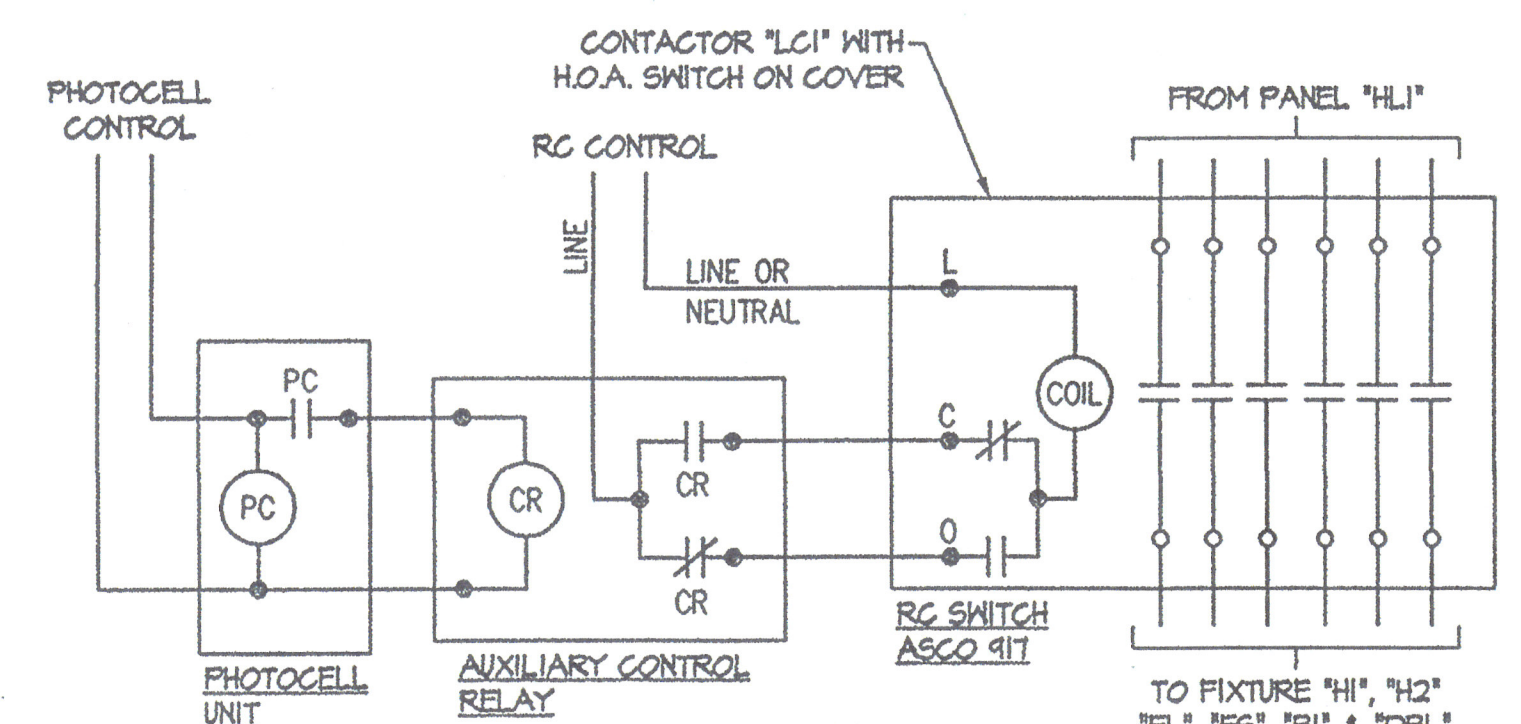
PARKING LOT LIGHTING CONTROL DIAGRAM NOT TO SCALE
