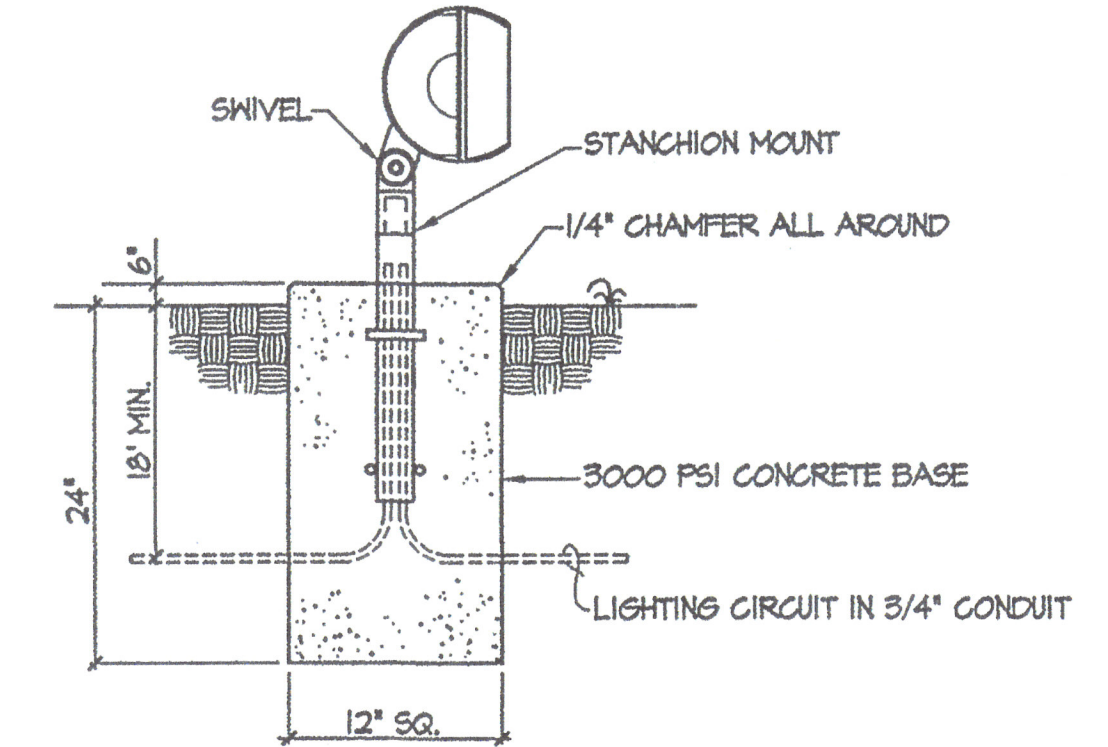
CONCRETE BASE DETAIL FIXTURE "FL" & "FS" NOT TO SCALE
