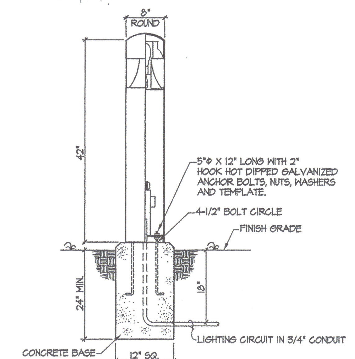
CONCRETE BASE DETAIL FIXTURE "B1" NOT TO SCALE
