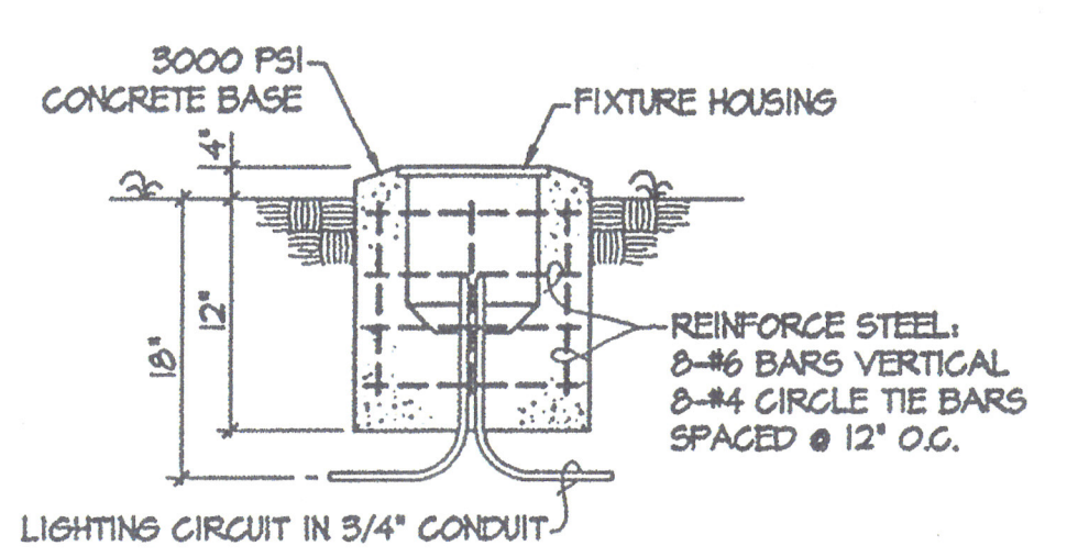
CONCRETE BASE DETAIL FIXTURE "DBL" NOT TO SCALE
