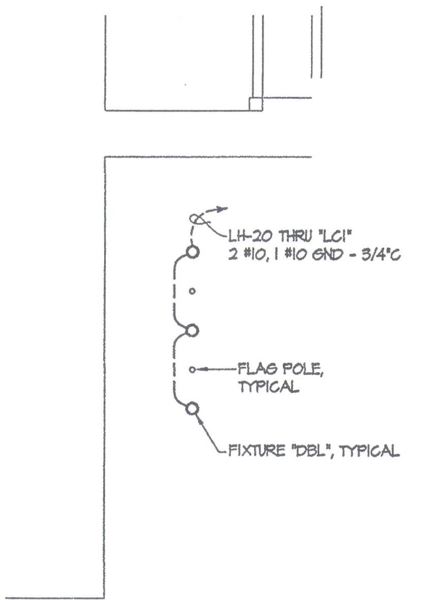
PARTIAL ELECTRICAL PLAN SCALE: 1" = 10'-0"
