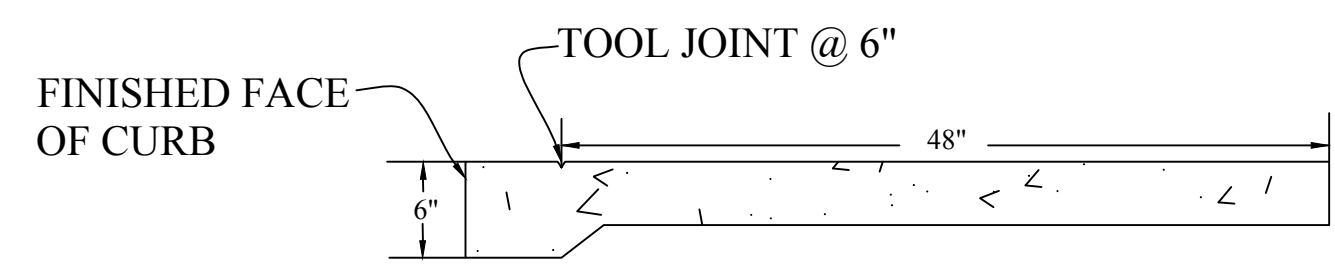
SIDEWALK DETAIL
