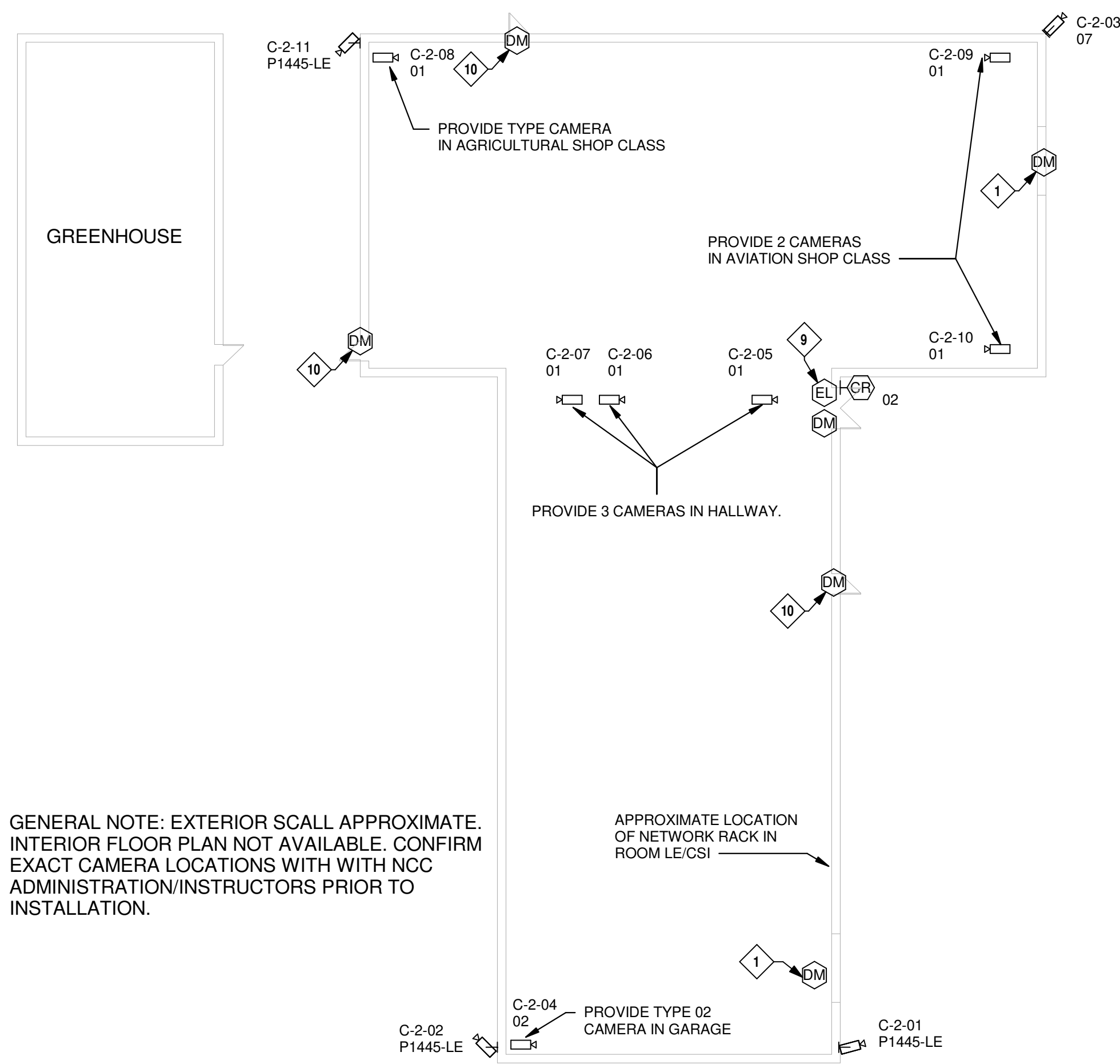
2 NORTHLAND CAREER CENTER SECURITY PLAN ANNEX 1/16" = 1'-0"
