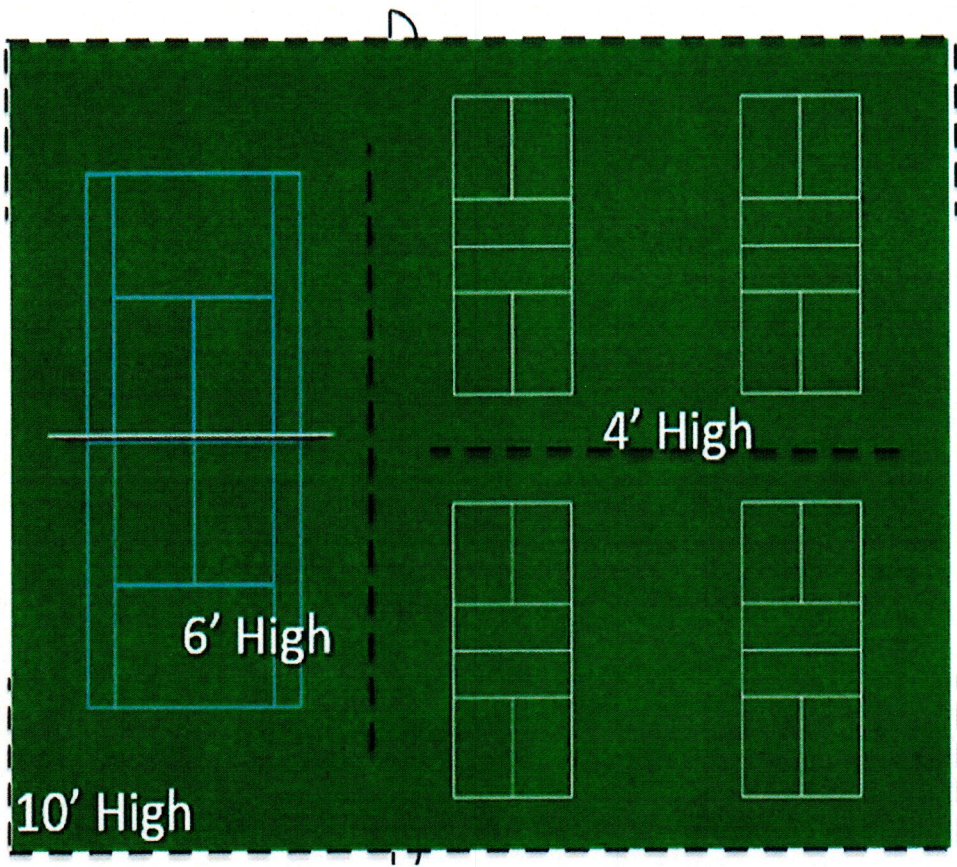
Fencing layout
