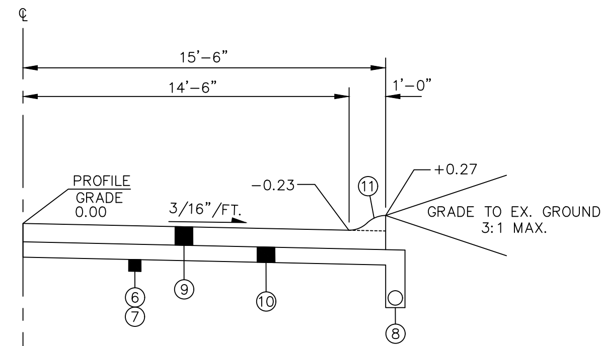
TYPICAL HALF SECTION CONCRETE PAVEMENT SECTION
