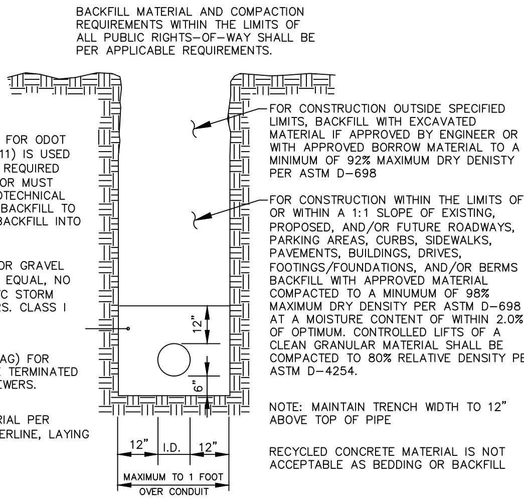
PIPE BEDDING AND BACKFILL DETAIL NOT TO SCALE
