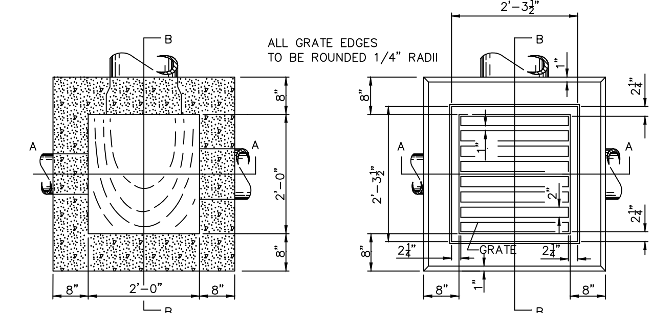
CATCH BASIN No. 2-2B NOT TO SCALE
