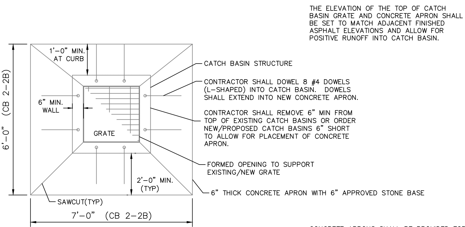
CONCRETE APRON AROUND CATCH BASINS PLAN VIEW NOT TO SCALE
