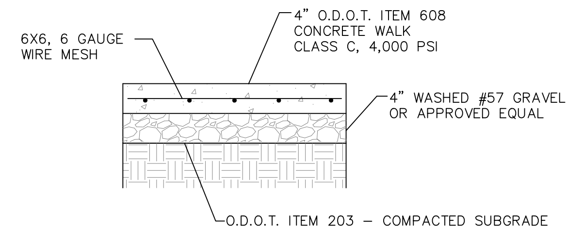
CONCRETE PAD AND SIDEWALK SECTION
