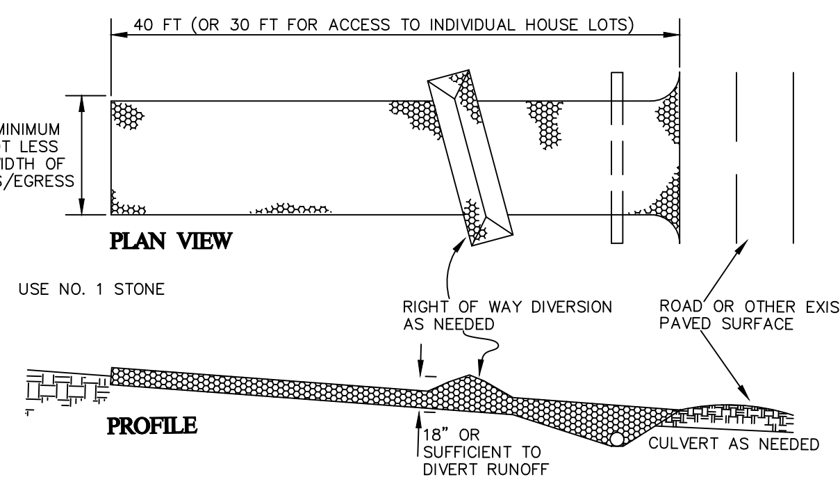
STABILIZED CONSTRUCTION ENTRANCE DETAIL NOT TO SCALE
