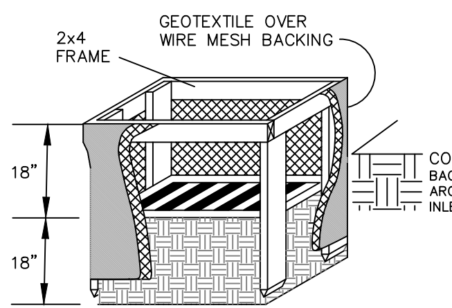
INLET PROTECTION DETAIL NOT TO SCALE
