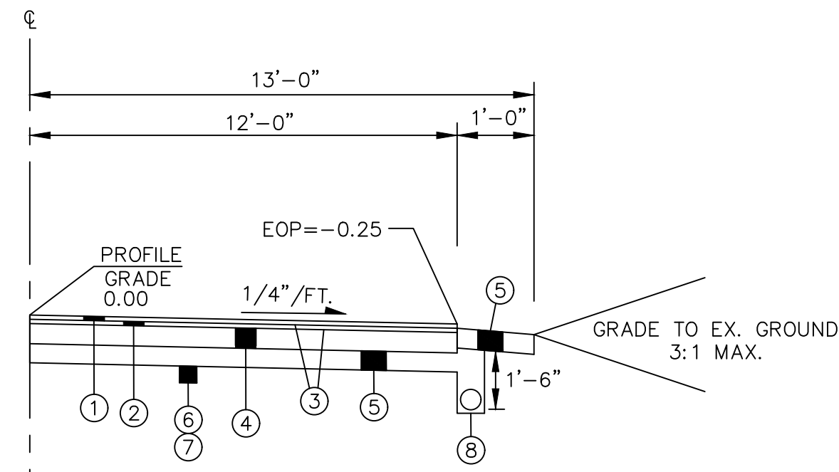
TYPICAL HALF SECTION ASPHALT PAVEMENT SECTION
