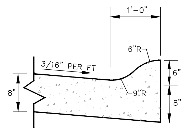
CONCRETE ROLL CURB (MATCH EXISTING)
