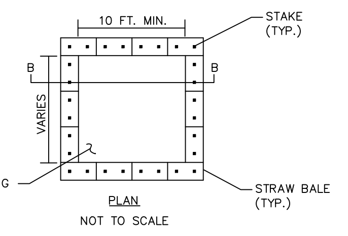
CONCRETE WASHOUT NOT TO SCALE
