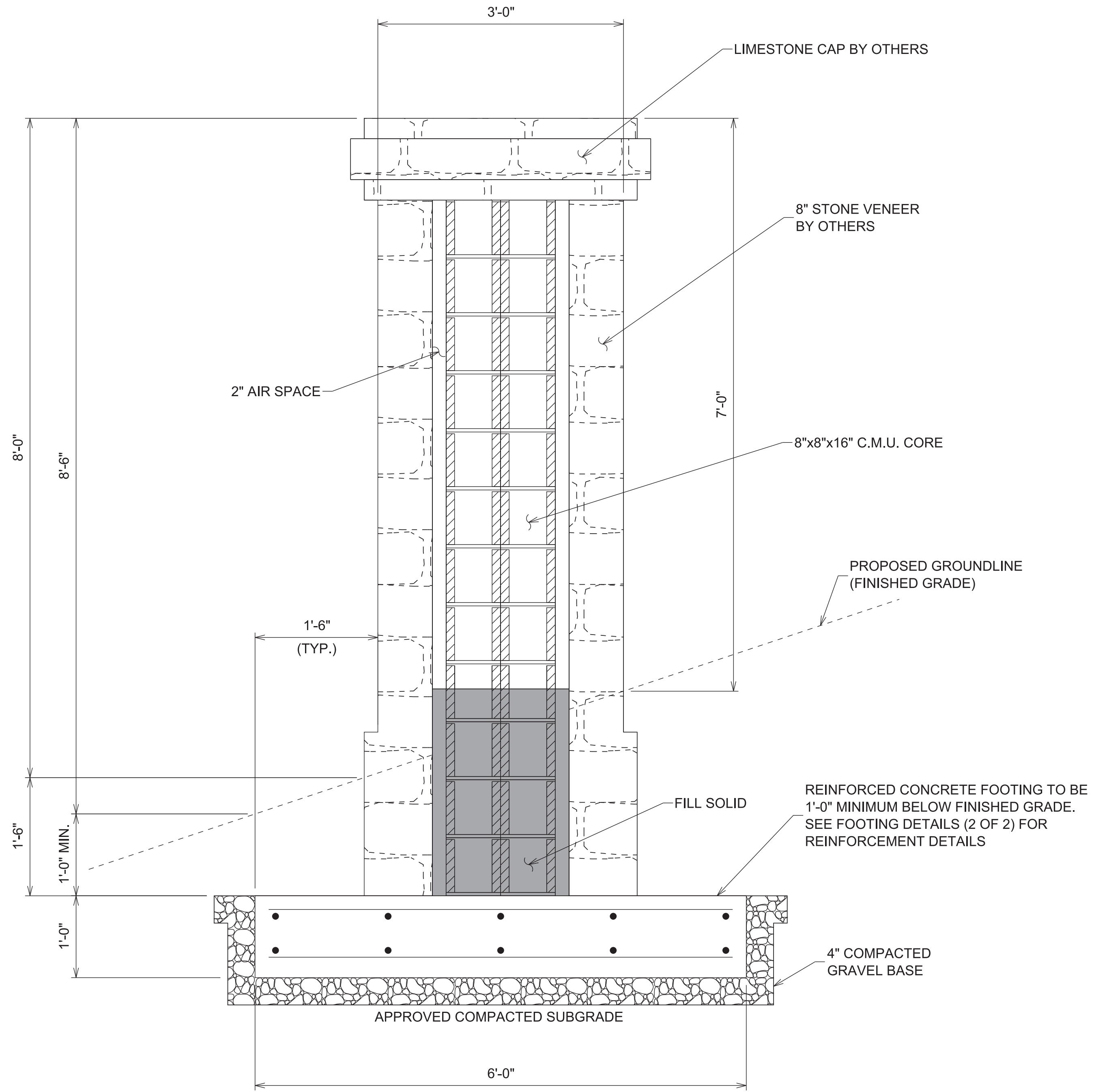
ELEVATION VIEW REINFORCEMENT NOT SHOWN FOR CLARITY NOT TO SCALE
