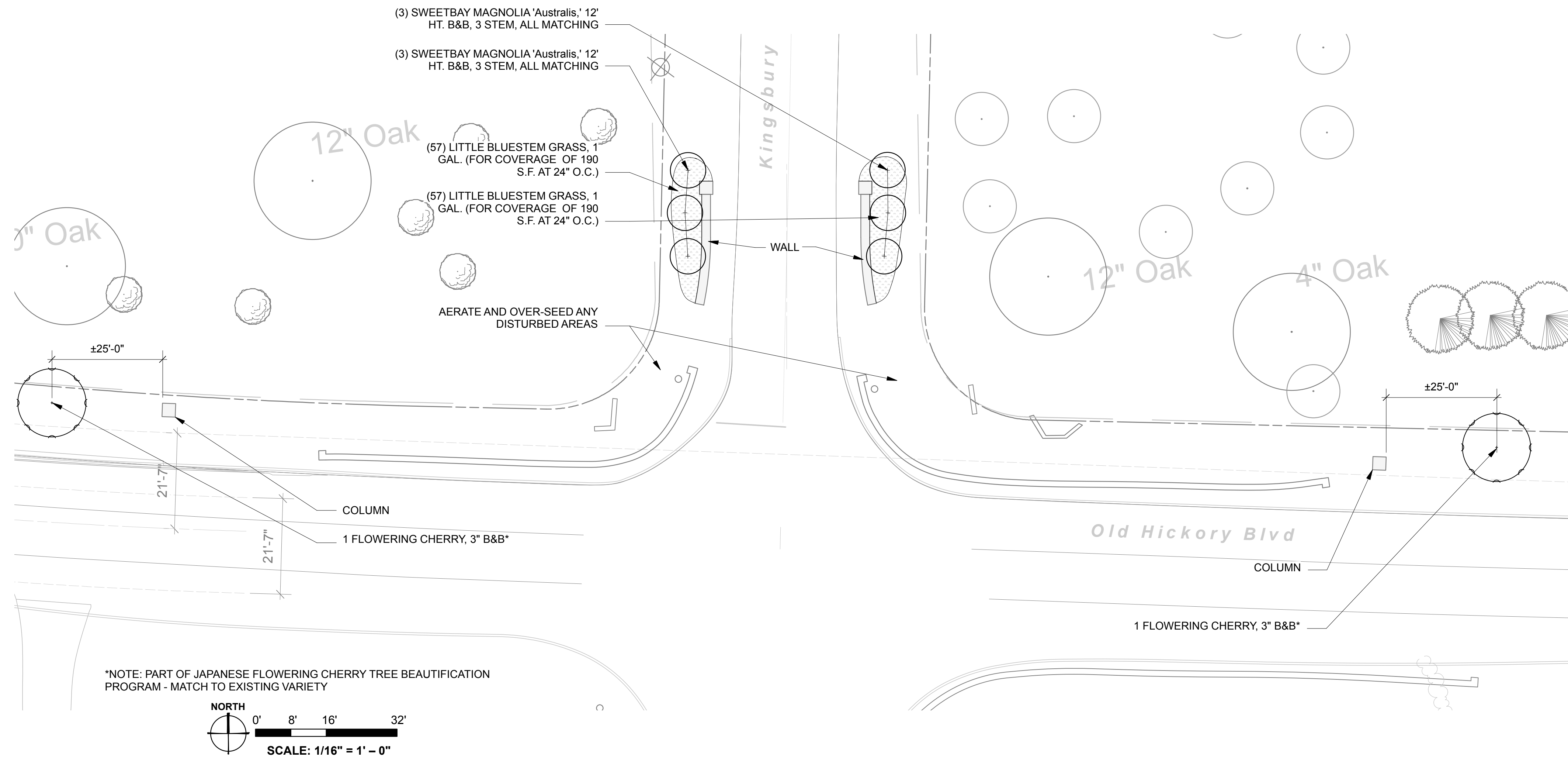
DETAIL 1: DETAILED PLANTING PLAN SCALE: 1/16" = 1' - 0"
