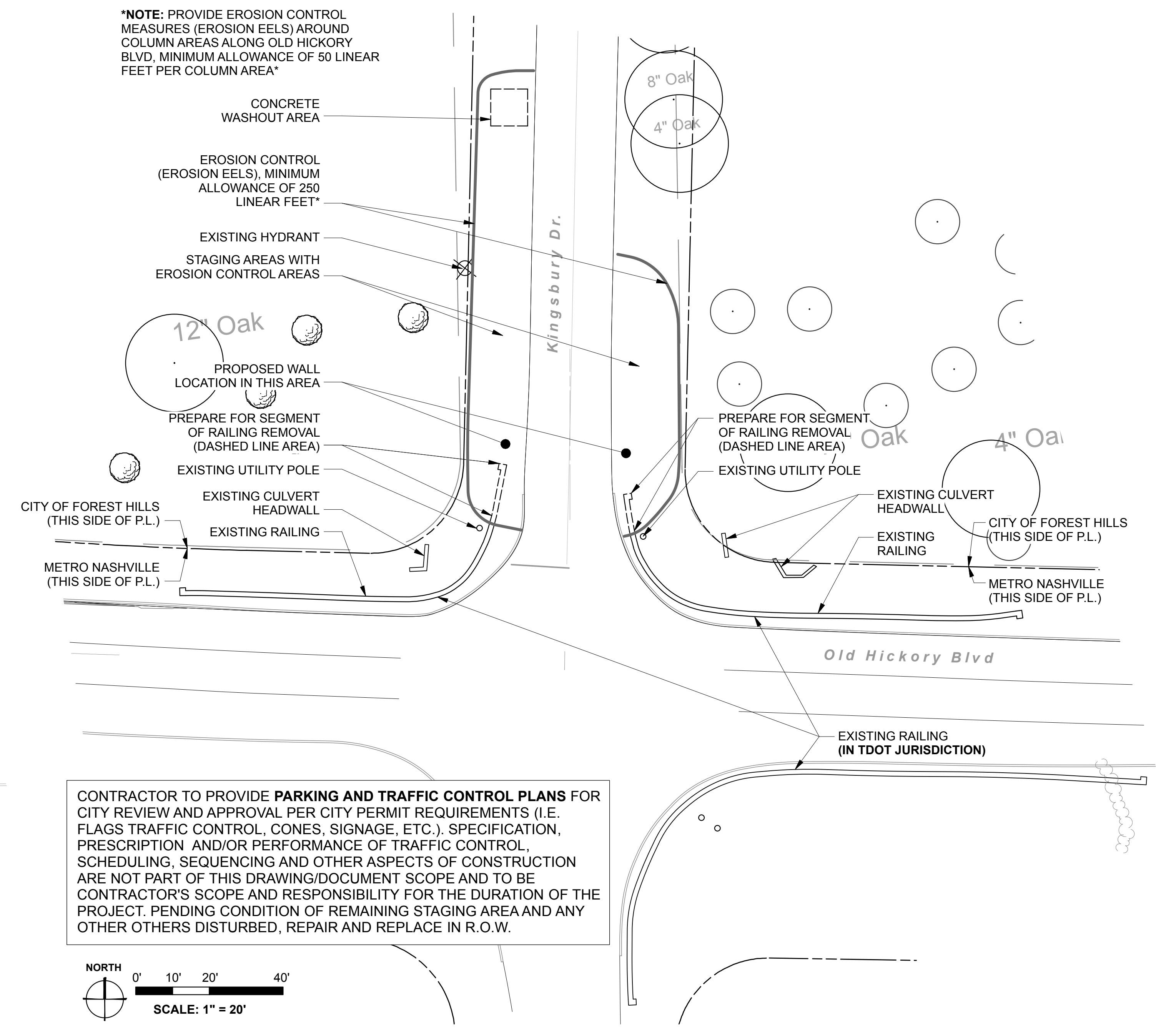
DETAIL 1: EXISTING CONDITIONS AND SITE PREPARATION SCALE: 1" = 20'
