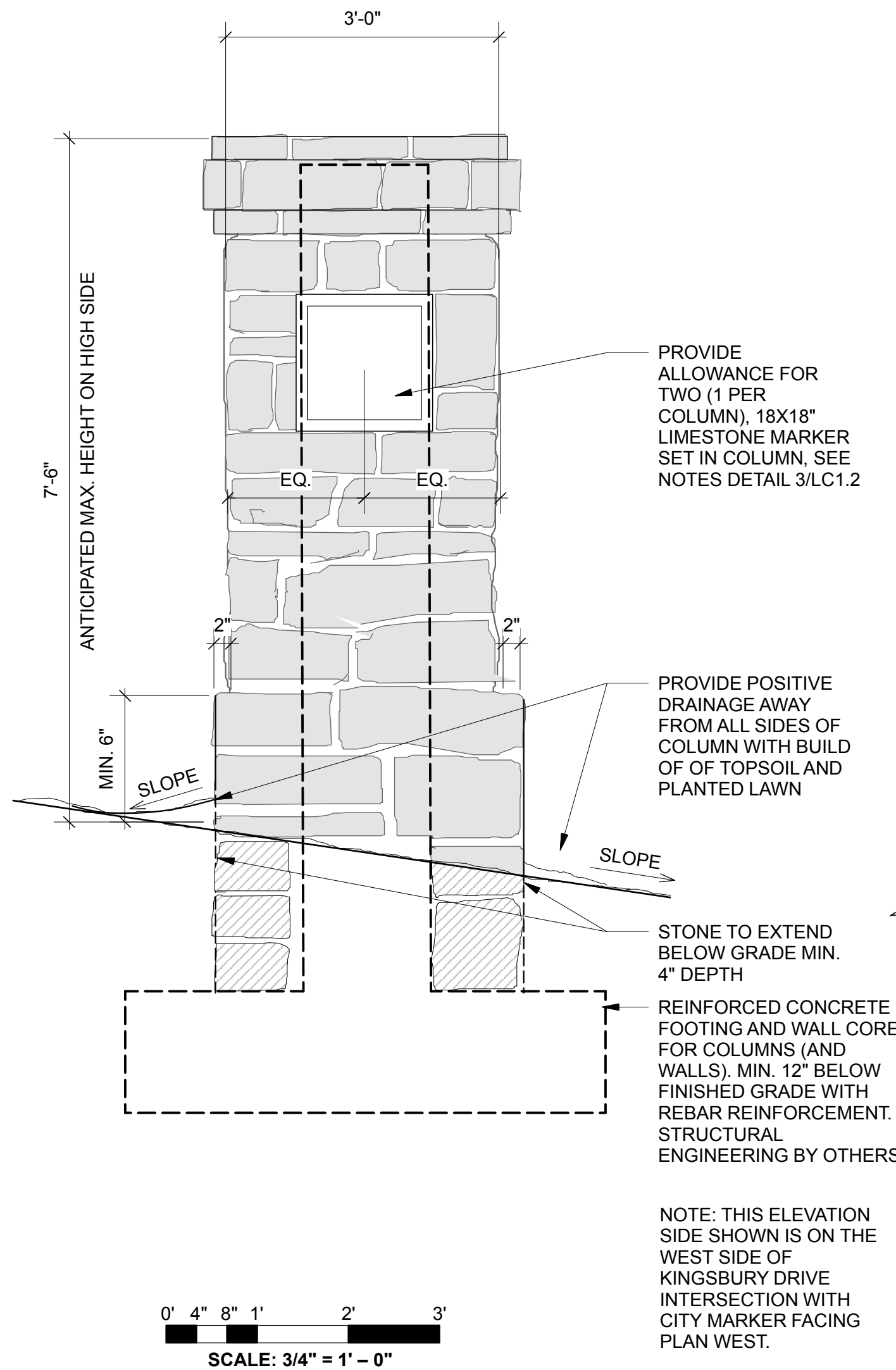
DETAIL 4: OLD HICKORY BLVD FACING COLUMN ELEVATION (COLUMN WEST OF KINGSBURY DR AND OHB INTERSECTION) SCALE: 1" = 20'
