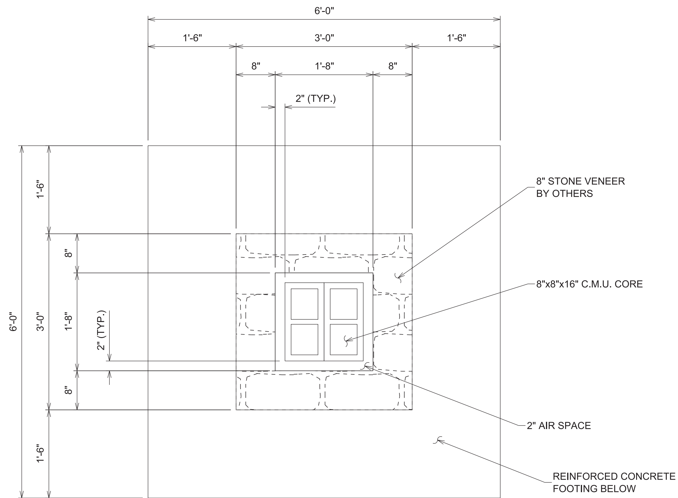
SECTION "B"-"B" NOT TO SCALE
