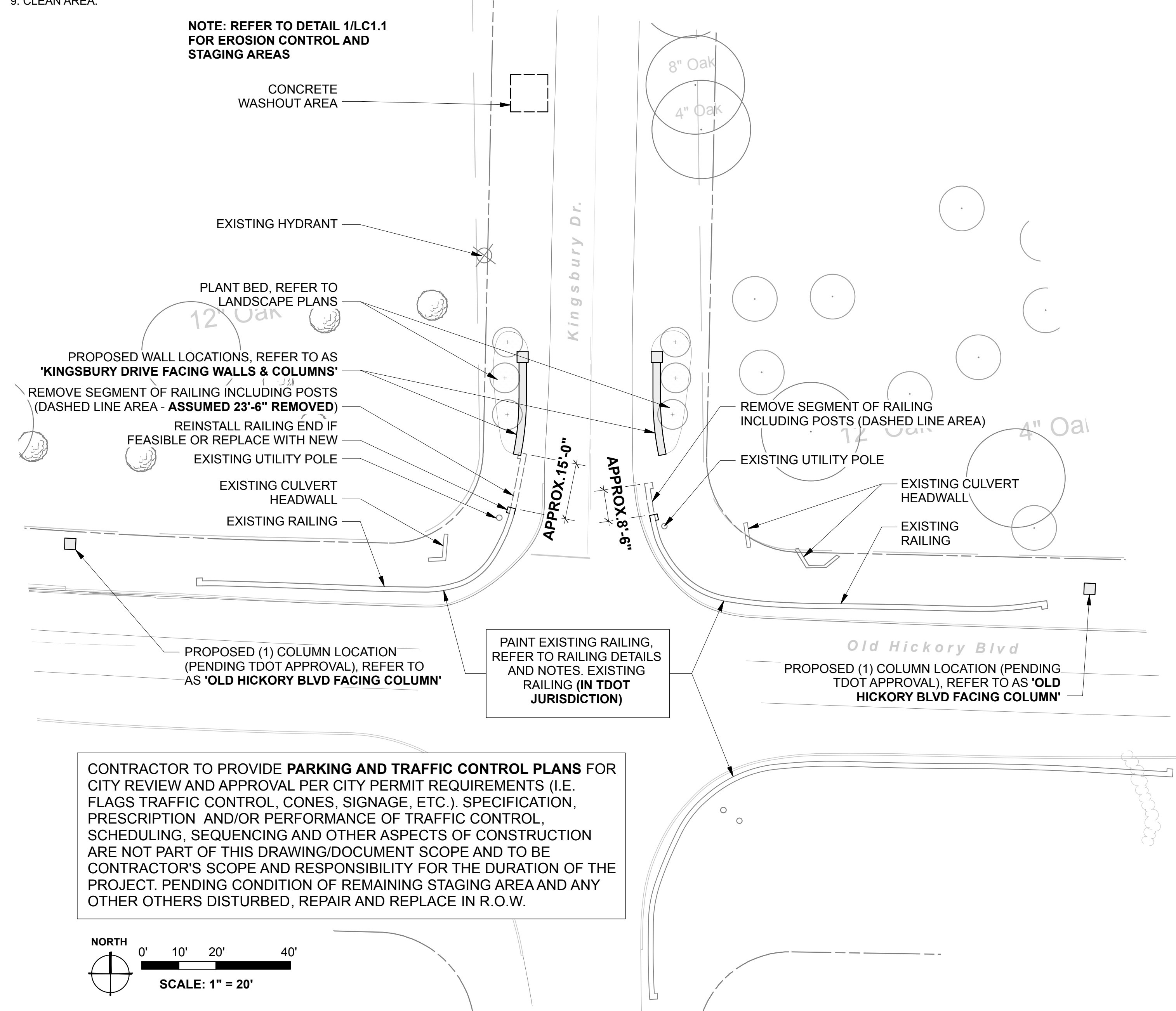
DETAIL 3: OVERALL SITE MATERIAL PLAN SCALE: 1" = 20'
