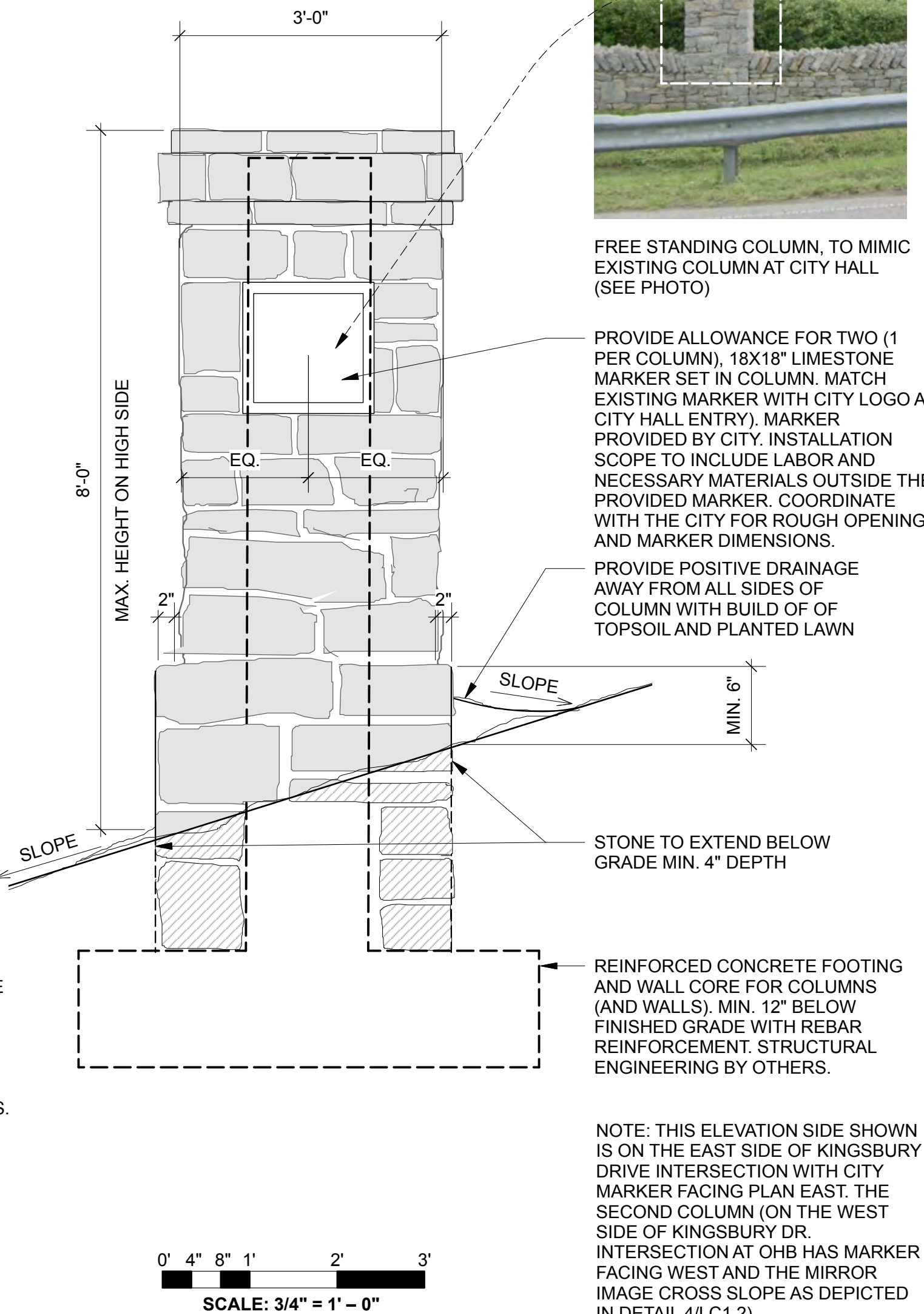
DETAIL 3: OLD HICKORY BLVD FACING COLUMN ELEVATION (COLUMN EAST OF KINGSBURY DR AND OHB INTERSECTION) SCALE: 1" = 20'
