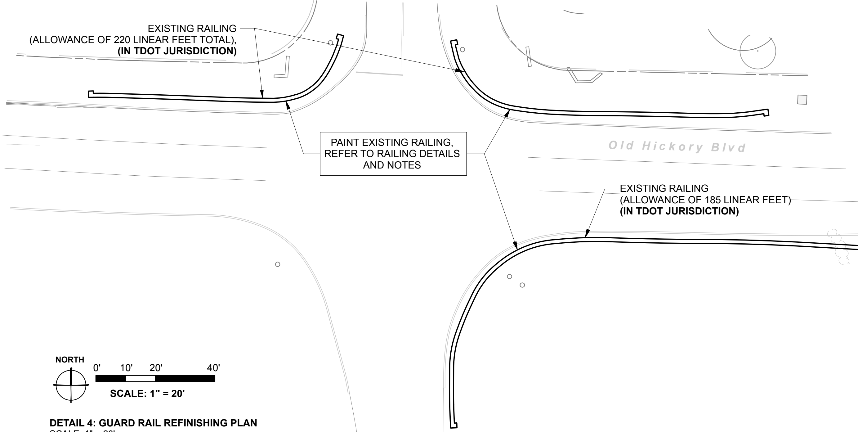
DETAIL 4: GUARD RAIL REFINISHING PLAN SCALE: 1" = 20'
