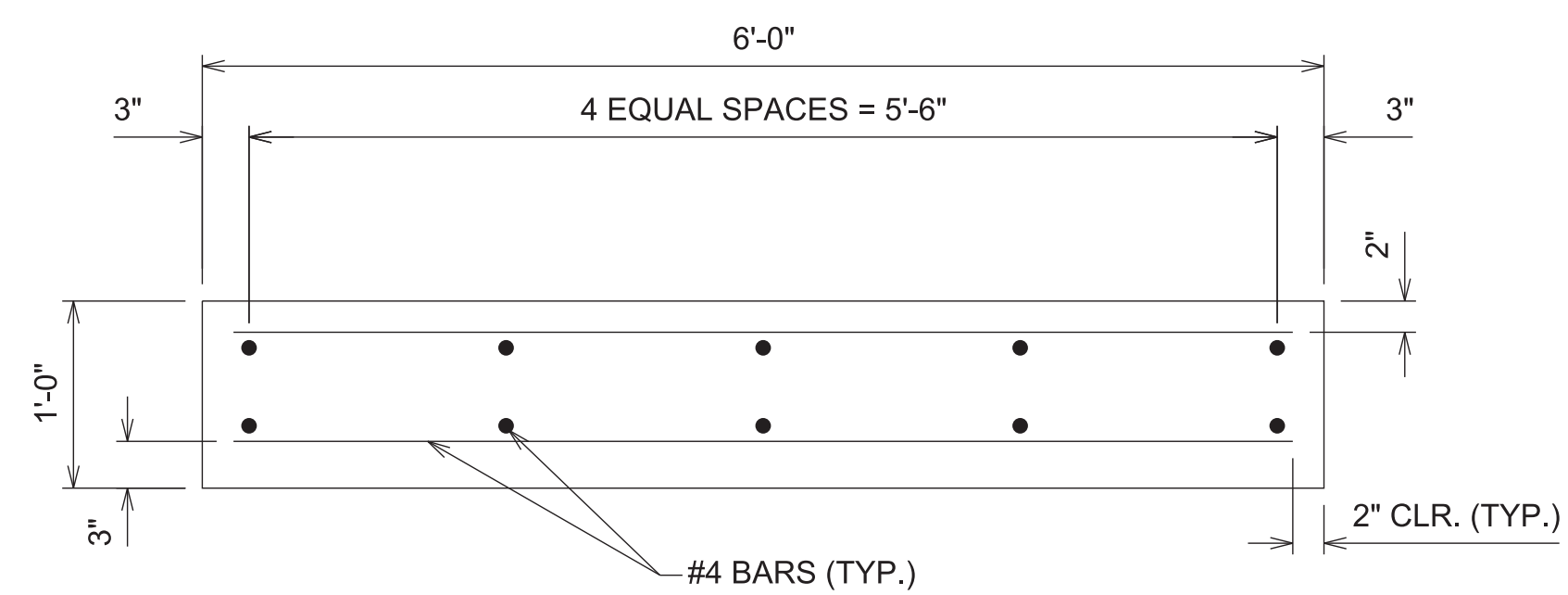
SECTION "D"-"D" SHOWING REINFORCEMENT NOT TO SCALE
