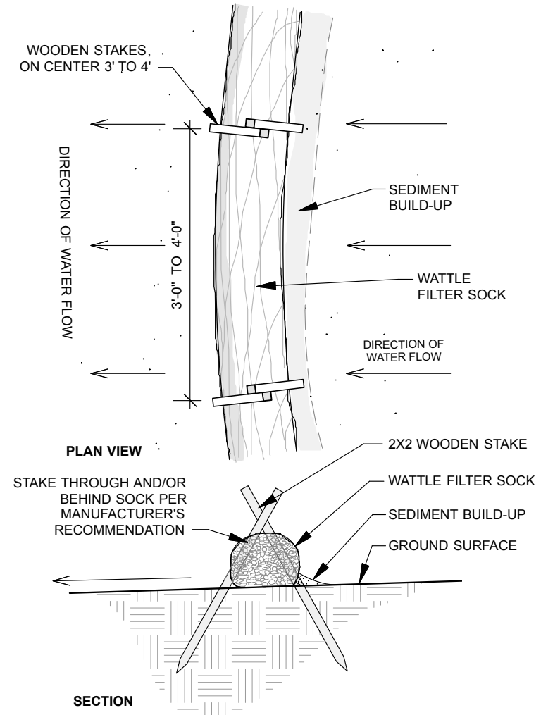
DETAIL 2: EROSION EEL/WATTLE FILTER SOCK DETAIL SCALE: N.T.S.
