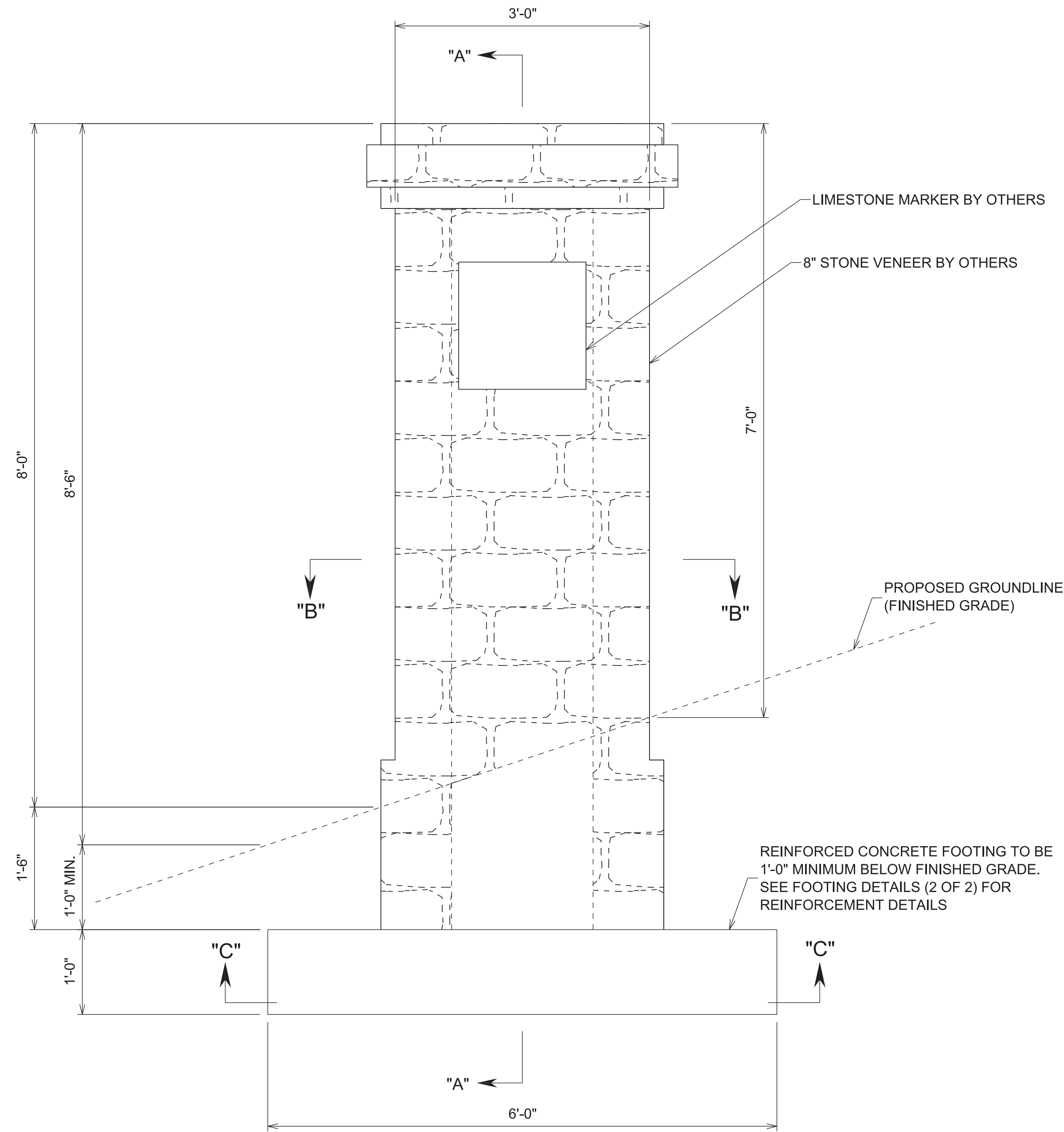
ELEVATION VIEW REINFORCEMENT NOT SHOWN FOR CLARITY NOT TO SCALE
