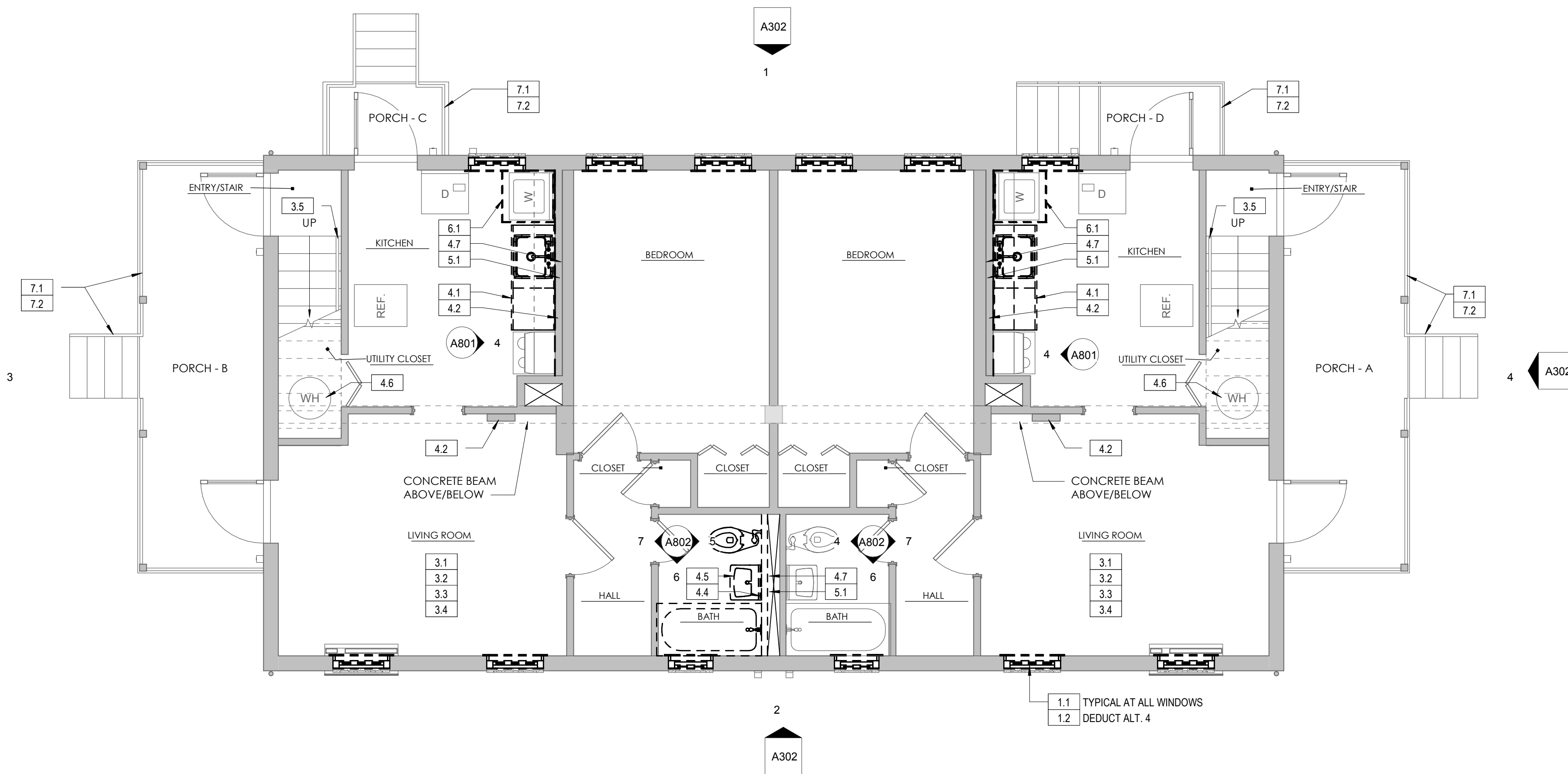
TYPE B - EXISTING FIRST FLOOR PLAN 1/4" = 1'-0"
