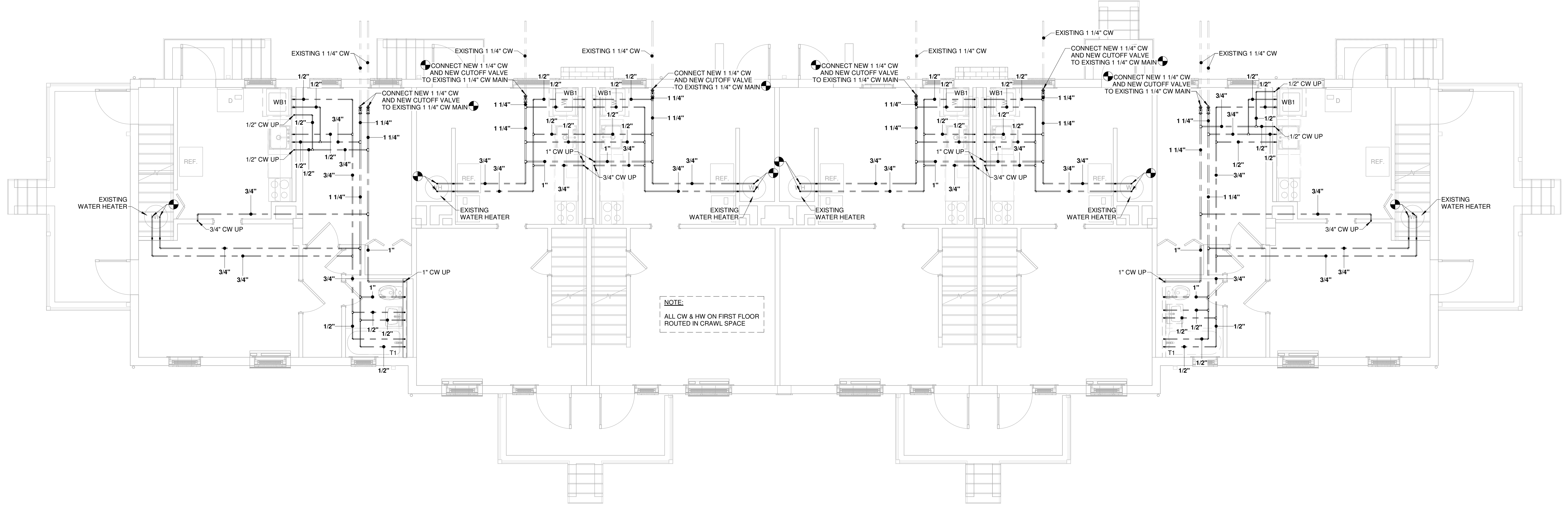
1 TYPE A - FIRST FLOOR DOMESTIC WATER PLAN 1/4" = 1'-0"
