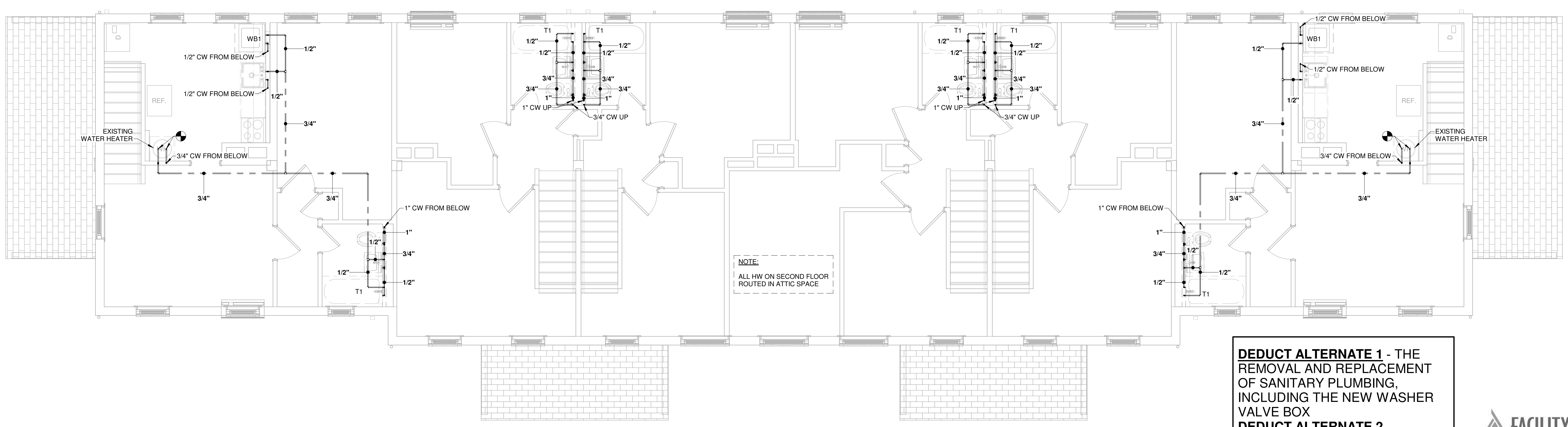
2 TYPE A - SECOND FLOOR DOMESTIC WATER PLAN 1/4" = 1'-0"
