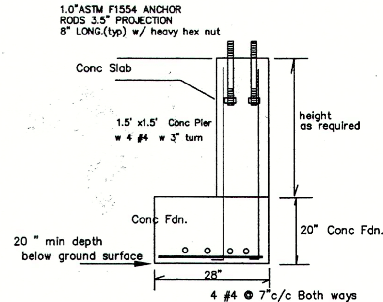
Main Frame Column Support Foundation Elevation -Section 1
