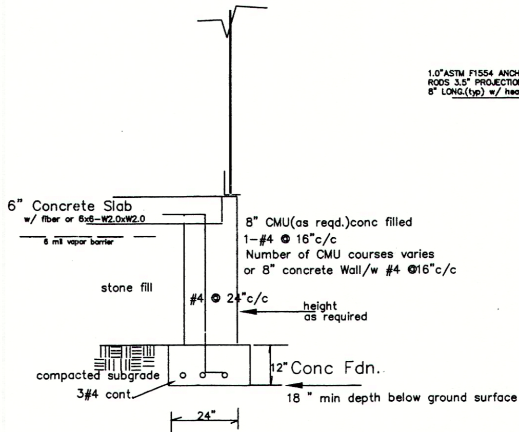
Section 3--Wall Footing NTS
