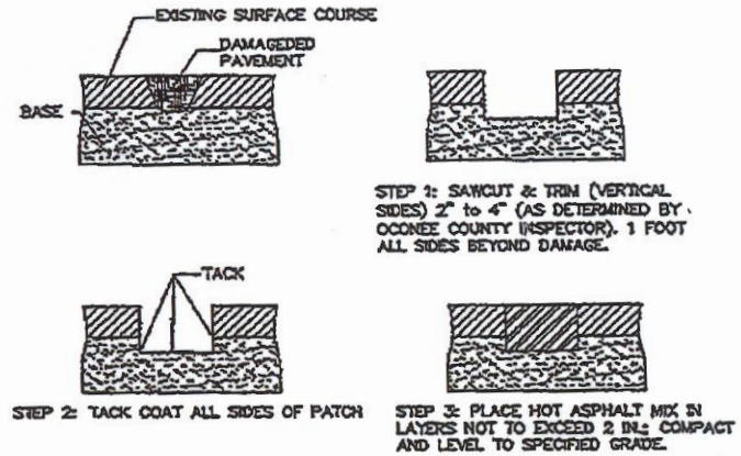
REPAIR OF FLEXIBLE PAVEMENT NOT TO SCALE
