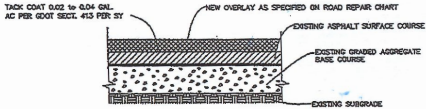
OVERLAY DETAIL NOT TO SCALE
