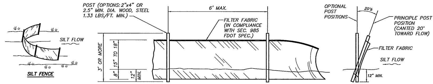
TYPICAL SILT FENCE
