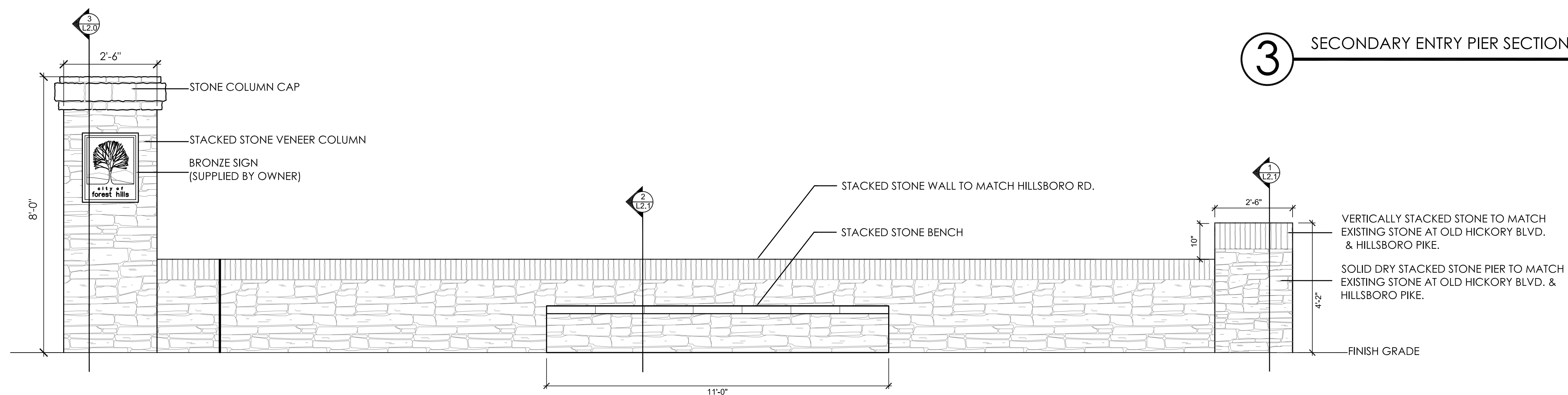
4 WALL ELEVATION
