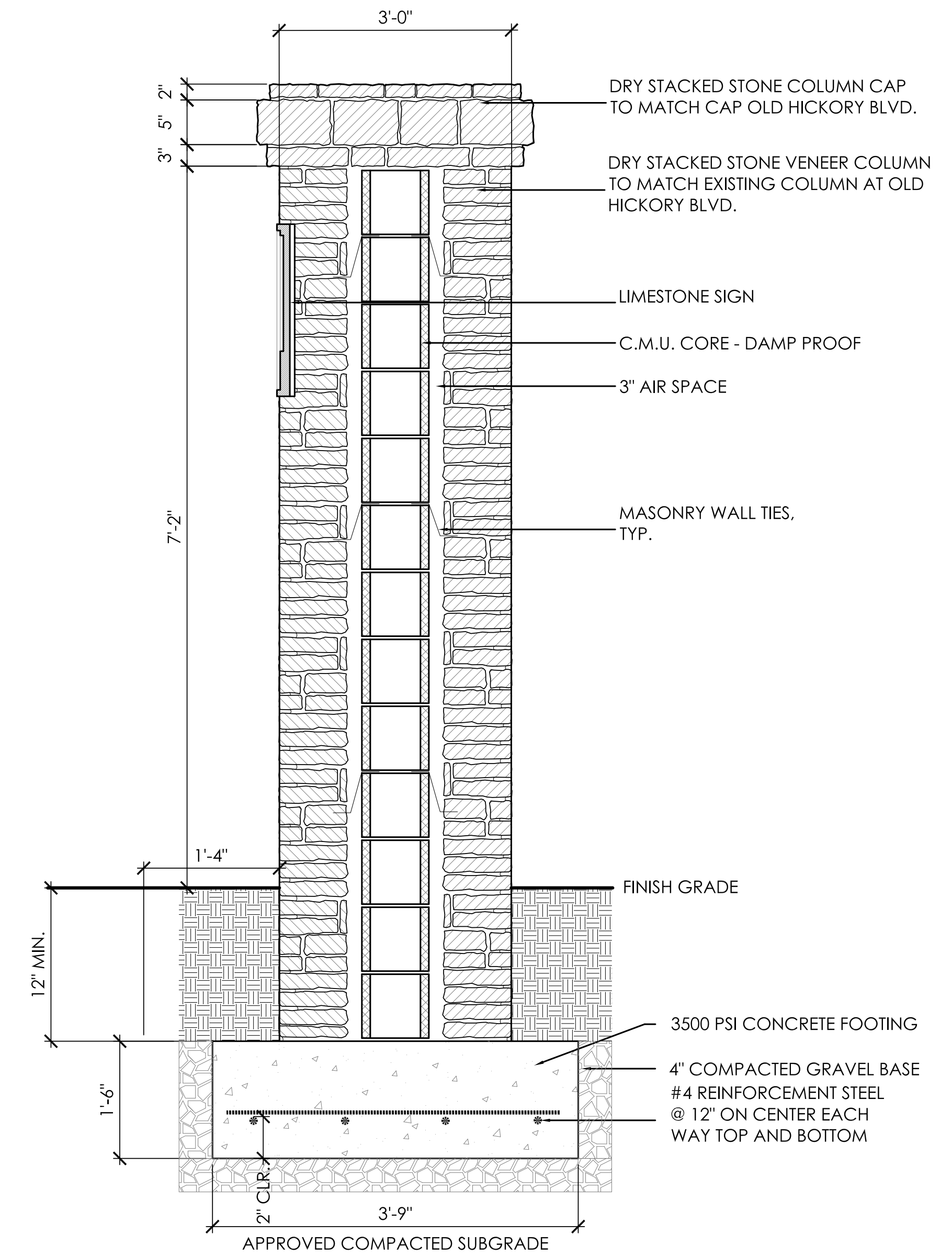
3 SECONDARY ENTRY PIER SECTION
