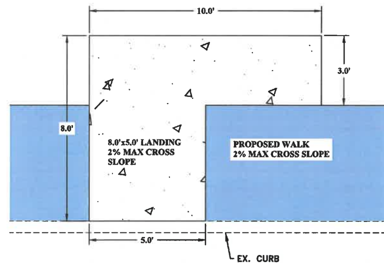
ADA BUS STOP LANDING AND BENCH PAD
