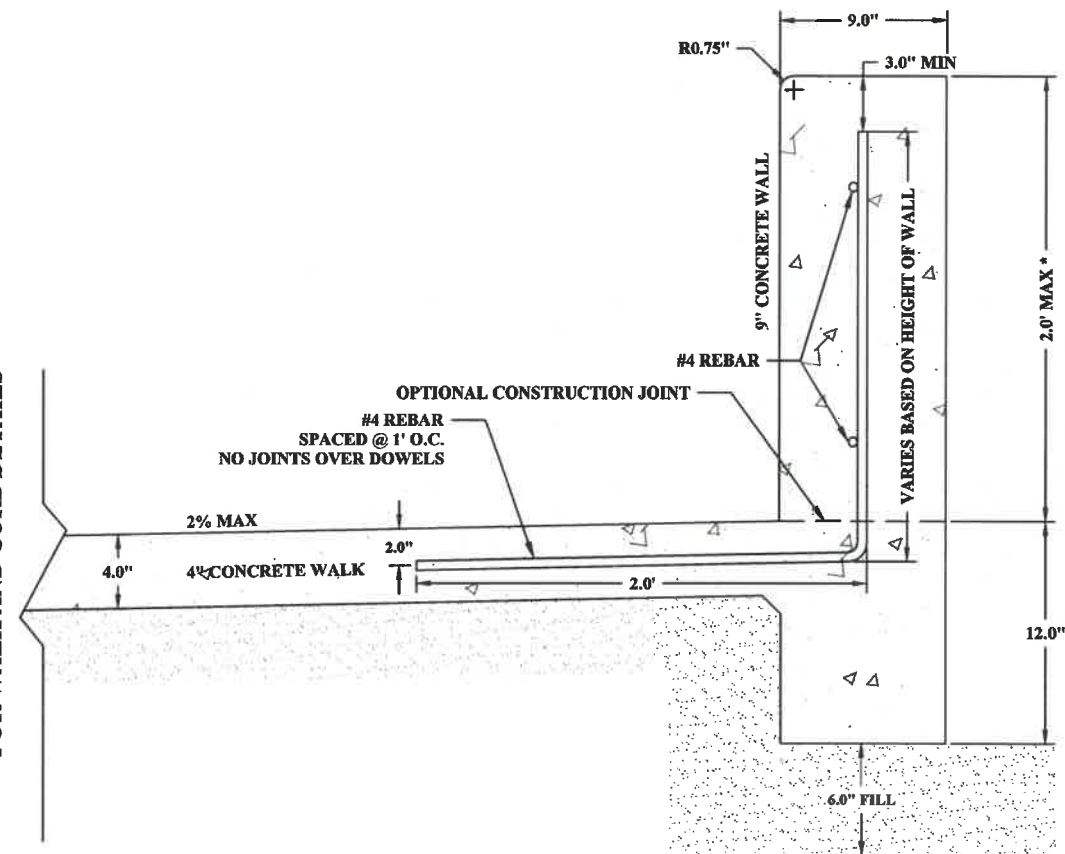
CURB AND SIDEWALK WITH WALL DETAIL
