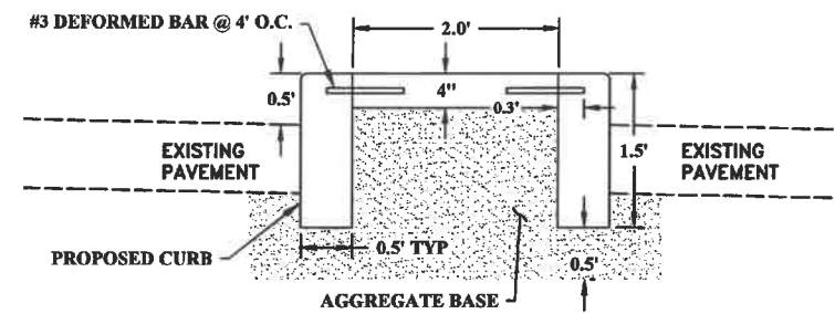
PROPOSED TRAFFIC ISLAND SEPARATOR
