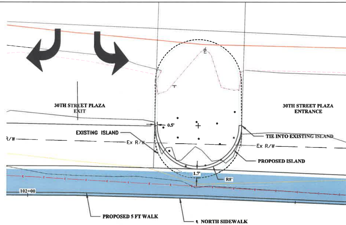
30TH STREET PLAZA DRIVEWAY ISLAND DETAIL
