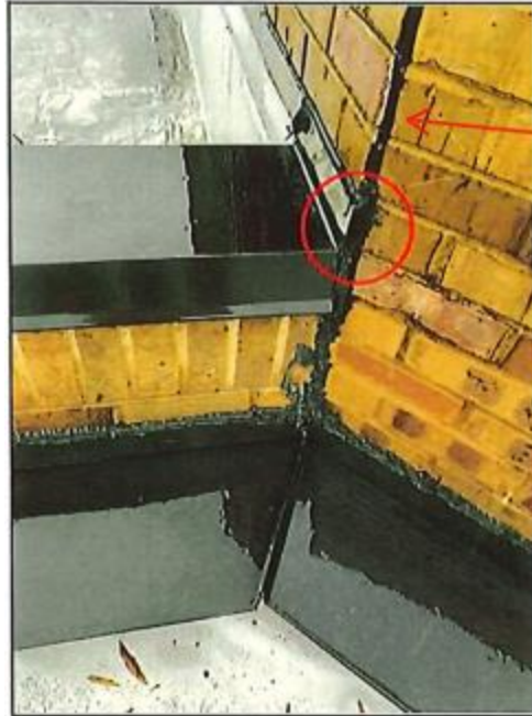
43 - Roof Level; sealant cracking
