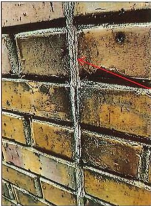
18 - Typical control joint cohesive failure
