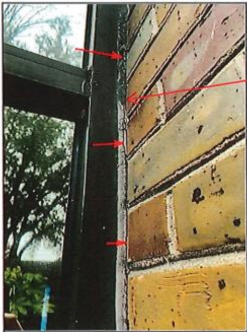
32 - Typical window sealant cracking
