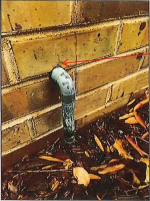
33 - Typical unsealed penetration
