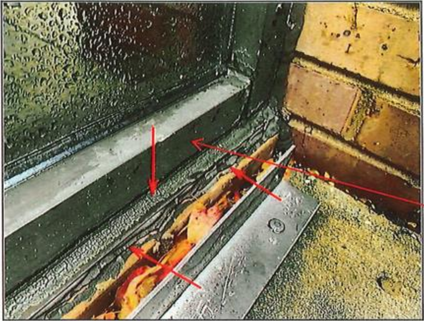
31 - Typical window sealant cracking
