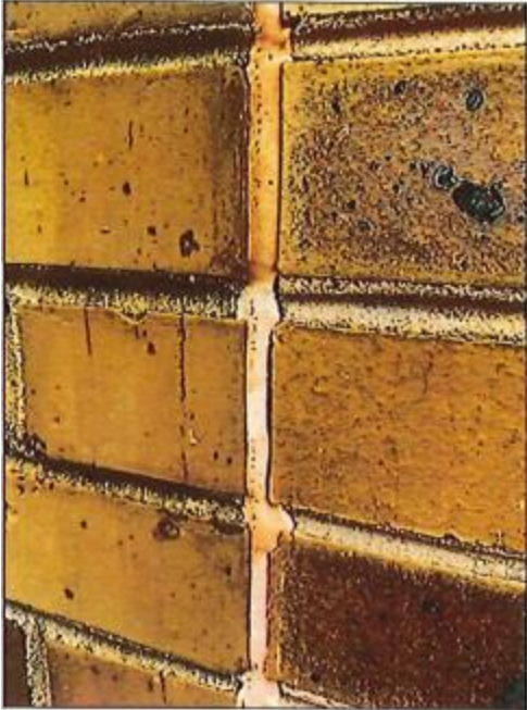
21 - Typical control joint cohesive failure
