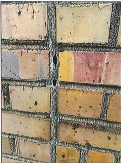
46 - Roof Level; sealant cohesive failure
