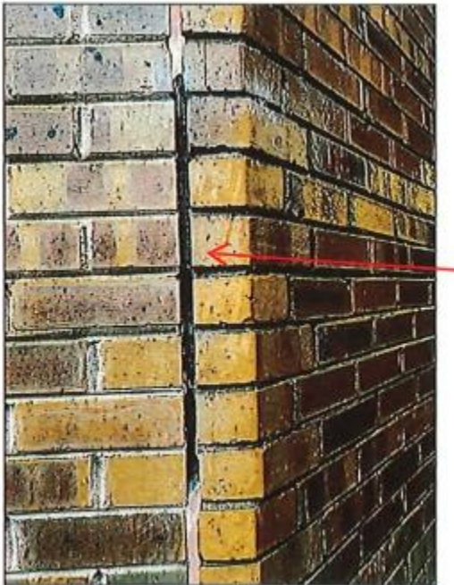
16 - Control joint damage
