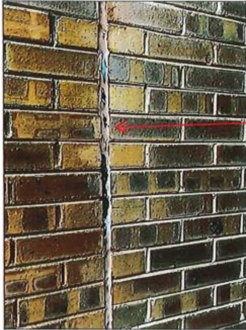
17 - Control joint cohesive failure and damage
