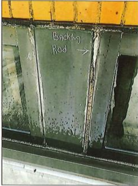
49 - Roof Level; clerestory window sealant cracking & backer rod exposure
