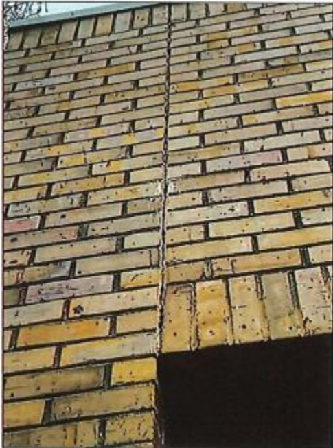
22 - Typical control joint cohesive failure
