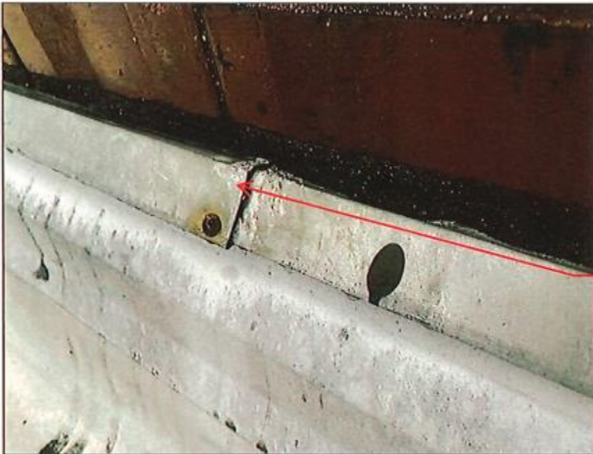
42 - Roof Level; through-wall flashing negatively sloped
