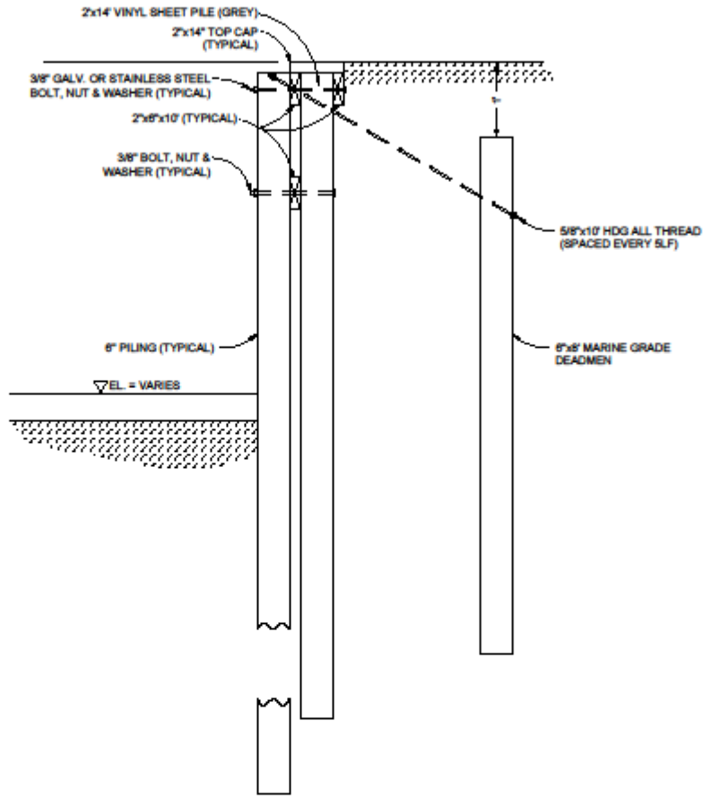
SECTION VIEW A-A SCALE 1/2" = 1'
