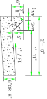
TYPE 3 MOUNTABLE CURB & GUTTER NTS.
