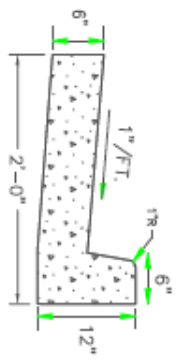
TYPE 1 CONCRETE CURB & GUTTER INDUSTRIAL ROAD NTS.
